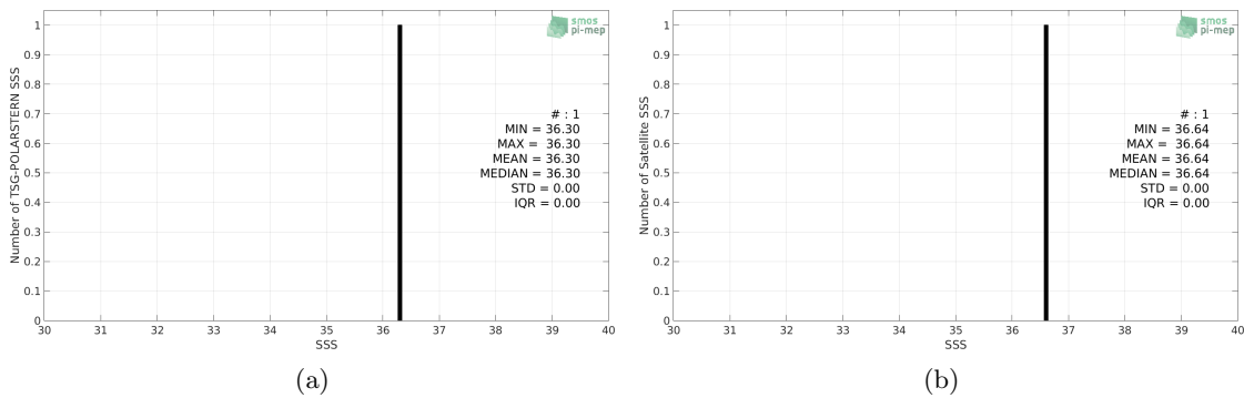
Figure 2: Histograms of SSS from TSG-POLARSTERN (a) and SMOS-L3-CATDS-CECOS-LOCEAN-V3-9DAYS-25KM (b) considering all match-up pairs per bins of 0.1 over the Congo river plume Pi-MEP region and for the full satellite product period.
