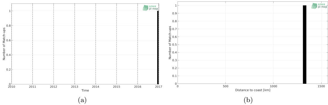
Figure 1: Number of match-ups between TSG-POLARSTERN and SMOS-L3-CATDS-CECOS-LOCEAN-V3-9DAYS-25KM SSS as a function of time (a) and as function of the distance to coast (b) over the Congo river plume Pi-MEP region and for the full satellite product period.
