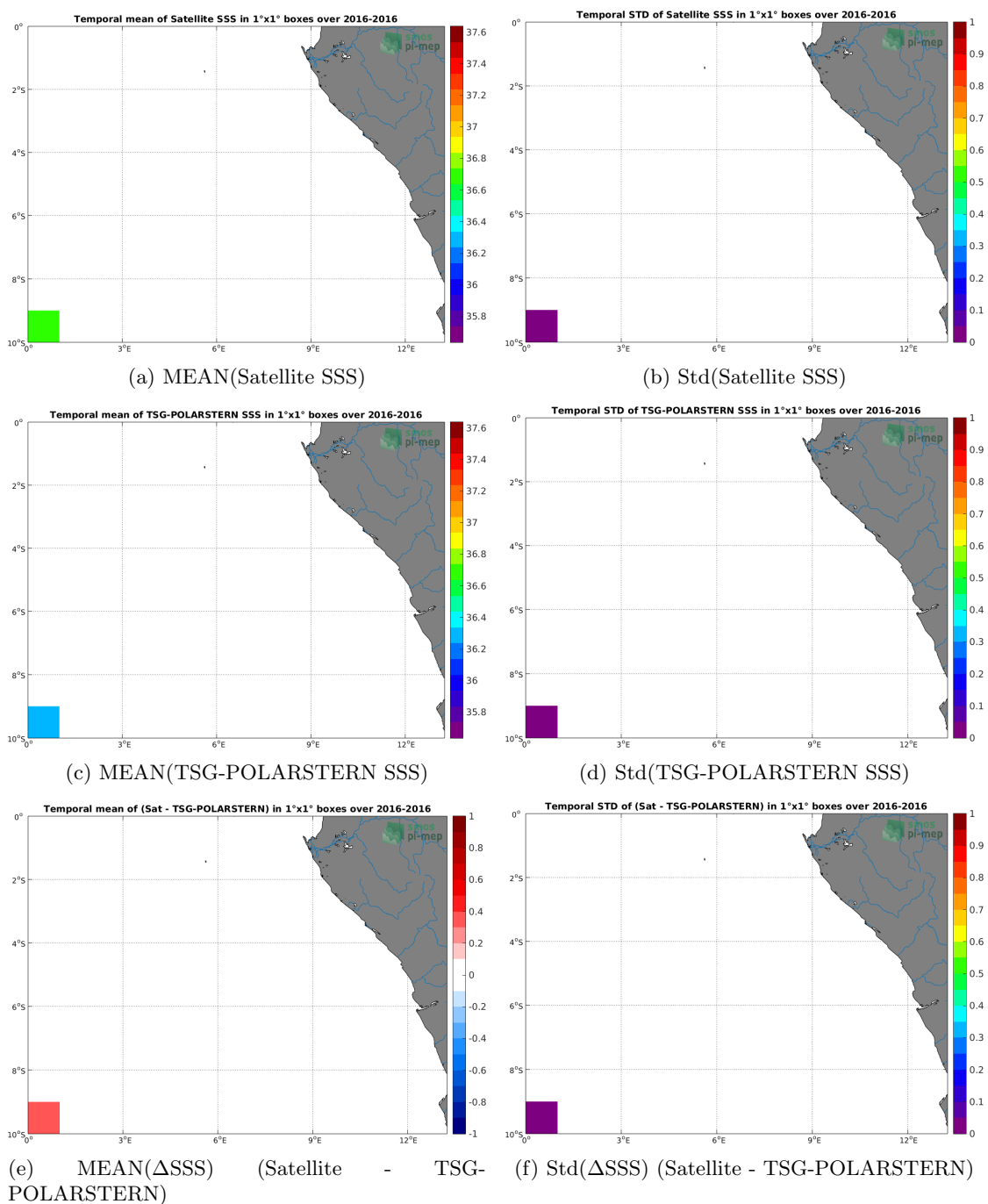
Figure 6: Temporal mean (left) and Std (right) of SSS from SMOS-L3-CATDS-CECOS-LOCEAN-V3-9DAYS-25KM (top), TSG-POLARSTERN (middle), and of \Delta SSS (Satellite - TSG-POLARSTERN). Only match-up pairs are used to generate these maps.
