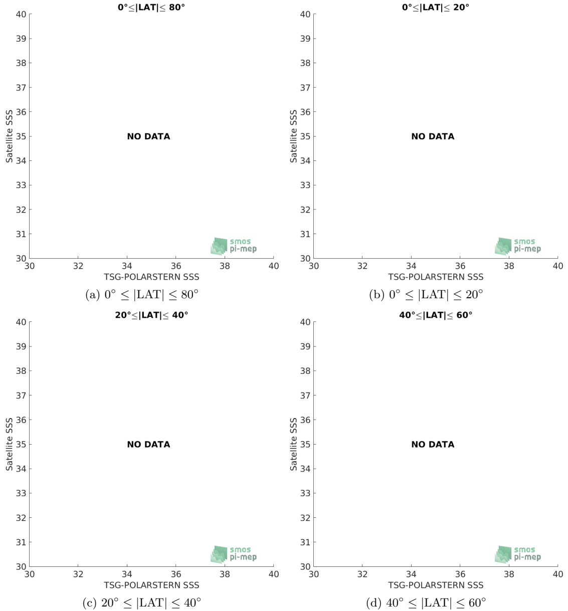
Figure 9: Contour maps of the concentration of SMOS-L3-CATDS-CECOS-LOCEAN-V3-9DAYS-25KM SSS ( y -axis) versus TSG-POLARSTERN SSS ( x -axis) at match-up pairs for different latitude bands. For each plot, the red line shows x=y . The black thin and dashed lines indicate a linear fit through the data cloud and the \pm 95\% confidence levels, respectively. The number match-up pairs n , the slope and R^2 coefficient of the linear fit, the root mean square (RMS) and the mean bias between satellite and in situ data are indicated for each latitude band in each plots.
