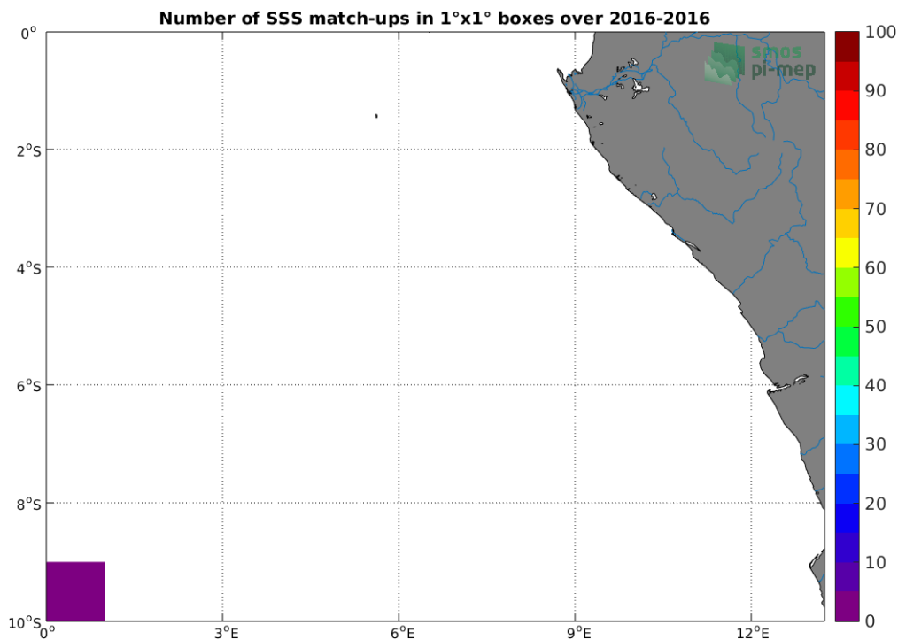
Figure 4: Number of SSS match-ups between TSG-POLARSTERN SSS and the SMOS-L3-CATDS-CECOS-LOCEAN-V3-9DAYS-25KM SSS product for the Congo river plume Pi-MEP region over 1^\circ \times 1^\circ boxes and for the full satellite product period.
