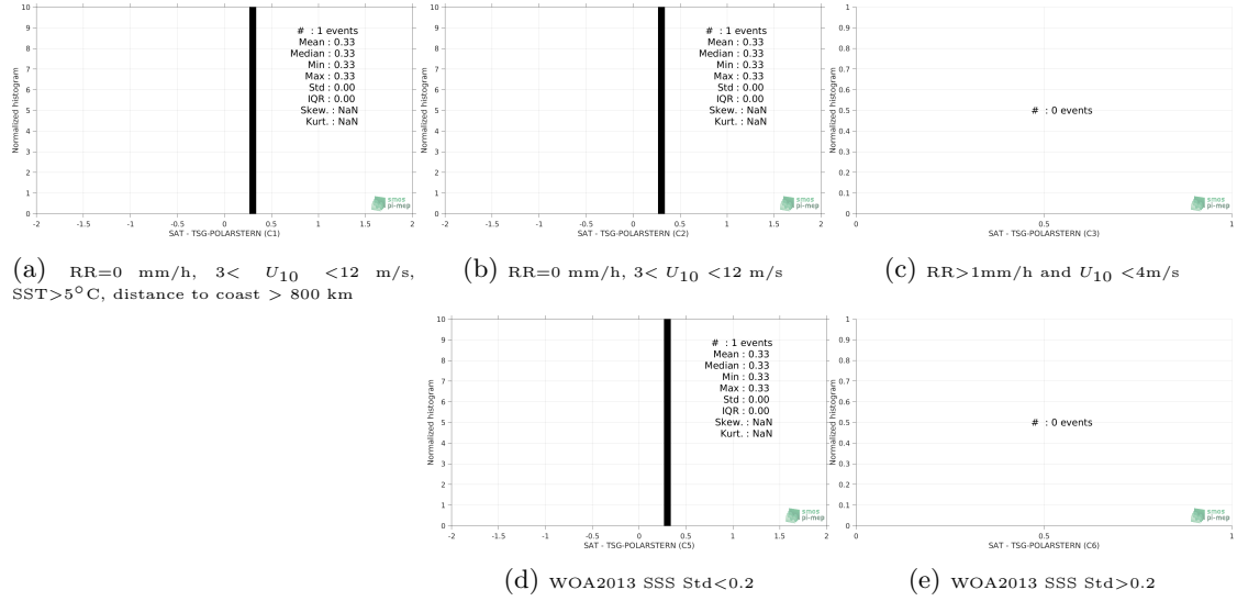
Figure 13: Normalized histogram of \Delta SSS (SMOS-L3-CATDS-CECOS-LOCEAN-V3-9DAYS-25KM - TSG-POLARSTERN) for 5 different subdatasets corresponding to: RR=0 mm/h, 3 < U_{10} < 12 m/s, SST>5°C, distance to coast > 800 km (a), RR=0 mm/h, 3 < U_{10} < 12 m/s (b), RR>1mm/h and U_{10} < 4 m/s (c), WOA2013 SSS Std<0.2 (d), WOA2013 SSS Std>0.2 (e).
