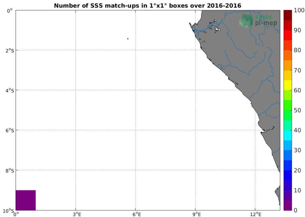
Figure 4: Number of SSS match-ups between TSG-POLARSTERN SSS and the SMOS-L3-CATDS-CECOS-LOCEAN-V3-9DAYS-25KM SSS product for the Congo river plume Pi-MEP region over 1°x1° boxes and for the full satellite product period.
