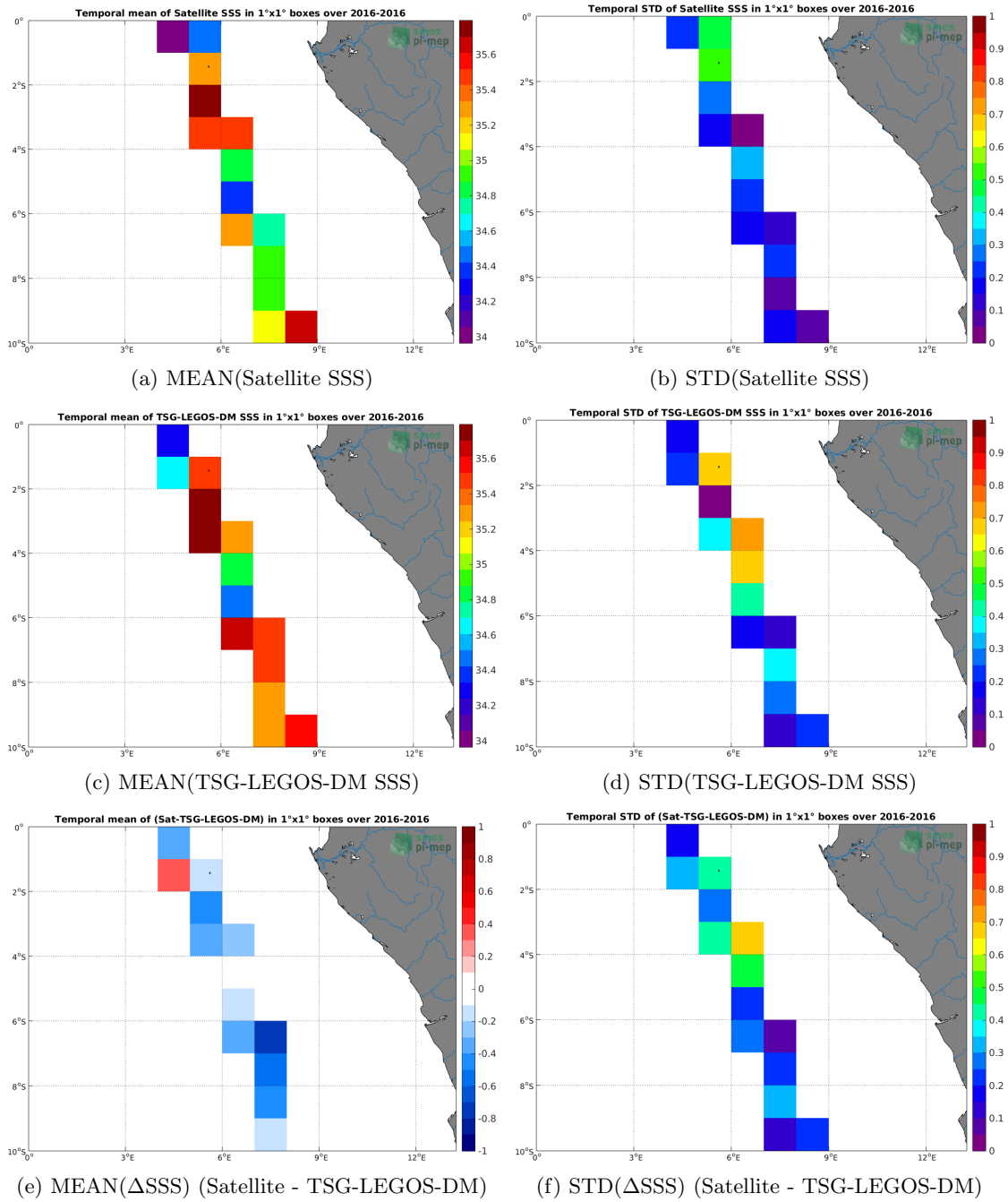
Figure 6: Temporal mean (left) and STD (right) of SSS from SMOS-L3-CATDS-CECOS-LOCEAN-V3-9DAYS-25KM (top), TSG-LEGOS-DM (middle), and of \Delta SSS (Satellite - TSG-LEGOS-DM). Only match-up pairs are used to generate these maps.
