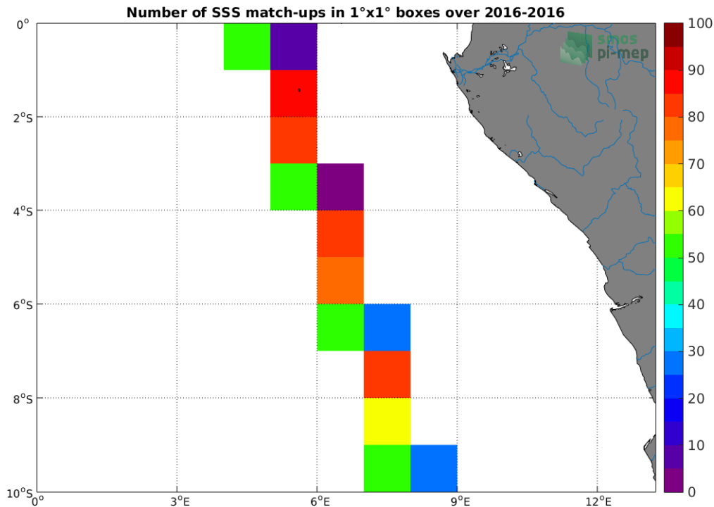
Figure 4: Number of SSS match-ups between TSG-LEGOS-DM SSS and the SMOS-L3-CATDS-CECOS-LOCEAN-V3-9DAYS-25KM SSS product for the Congo river plume Pi-MEP region over 1°x1° boxes and for the full satellite product period.
