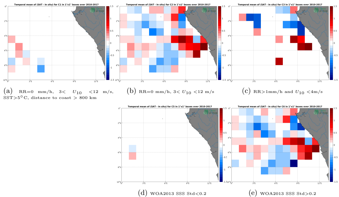
Figure 12: Temporal mean gridded over spatial boxes of size 1^\circ \times 1^\circ of \Delta SSS (SMOS-L3-CATDS-CECOS-LOCEAN-V3-9DAYS-25KM - TSG-GOSUD-Research-vessel) for 5 different subdatasets corresponding to: RR=0 mm/h, 3 < U_{10} < 12 m/s, SST > 5°C, distance to coast > 800 km (a), RR=0 mm/h, 3 < U_{10} < 12 m/s (b), RR > 1mm/h and U_{10} < 4 m/s (c), WOA2013 SSS Std < 0.2 (d), WOA2013 SSS Std > 0.2 (e).
