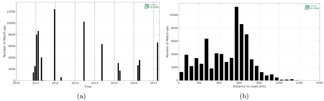
Figure 1: Number of match-ups between TSG-GOSUD-Research-vessel and SMOS-L3-CATDS-CECOS-LOCEAN-V3-9DAYS-25KM SSS as a function of time (a) and as function of the distance to coast (b) over the Congo river plume Pi-MEP region and for the full satellite product period.
