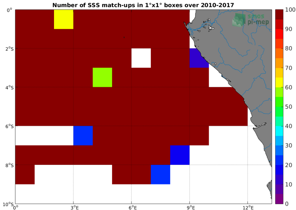
Figure 4: Number of SSS match-ups between TSG-GOSUD-Research-vessel SSS and the SMOS-L3-CATDS-CECOS-LOCEAN-V3-9DAYS-25KM SSS product for the Congo river plume Pi-MEP region over 1^\circ \times 1^\circ boxes and for the full satellite product period.
