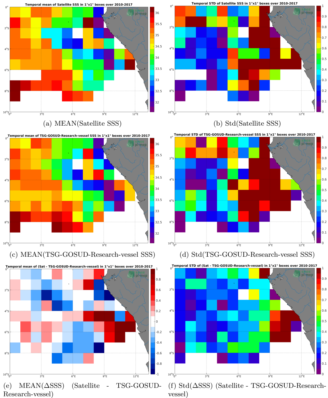
Figure 6: Temporal mean (left) and Std (right) of SSS from SMOS-L3-CATDS-CECOS-LOCEAN-V3-9DAYS-25KM (top), TSG-GOSUD-Research-vessel (middle), and of \Delta SSS (Satellite - TSG-GOSUD-Research-vessel). Only match-up pairs are used to generate these maps.
