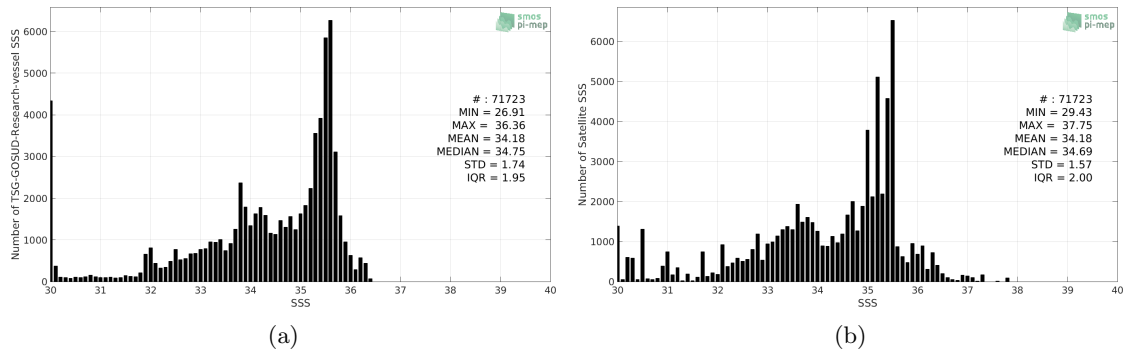
Figure 2: Histograms of SSS from TSG-GOSUD-Research-vessel (a) and SMOS-L3-CATDS-CECOS-LOCEAN-V3-9DAYS-25KM (b) considering all match-up pairs per bins of 0.1 over the Congo river plume Pi-MEP region and for the full satellite product period.
