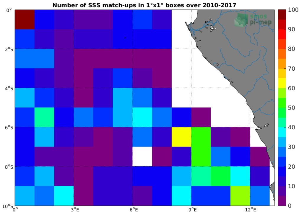
Figure 4: Number of SSS match-ups between Argo SSS and the SMOS-L3-CATDS-CECOS-LOCEAN-V3-9DAYS-25KM SSS product for the Congo river plume Pi-MEP region over 1°x1° boxes and for the full satellite product period.
