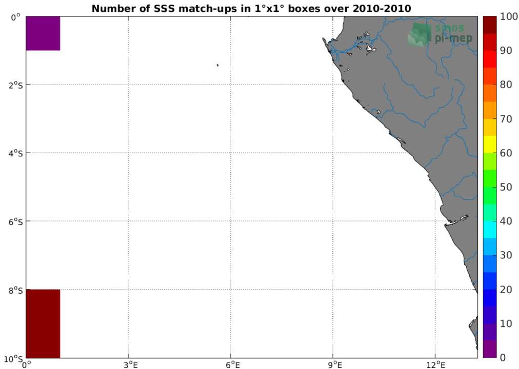
Figure 4: Number of SSS match-ups between TSG-SAMOS SSS and the SMOS-L3-CATDS-CECOS-LOCEAN-V3-18DAYS-25KM SSS product for the Congo river plume Pi-MEP region over 1^\circ \times 1^\circ boxes and for the full satellite product period.
