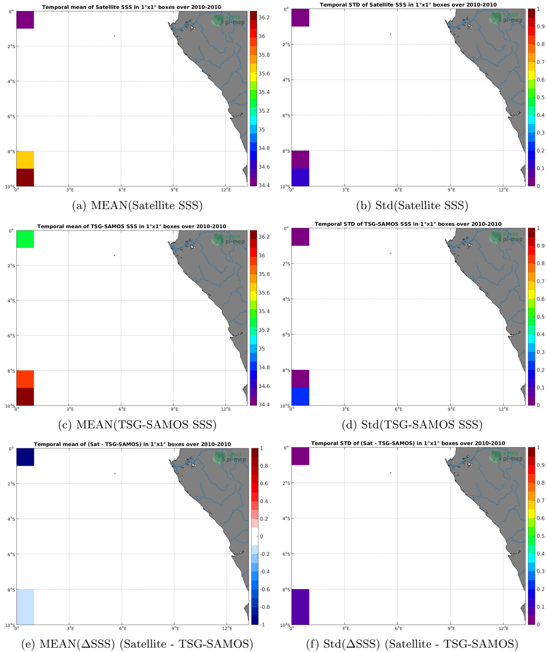
Figure 6: Temporal mean (left) and Std (right) of SSS from SMOS-L3-CATDS-CECOS-LOCEAN-V3-18DAYS-25KM (top), TSG-SAMOS (middle), and of \Delta SSS (Satellite - TSG-SAMOS). Only match-up pairs are used to generate these maps.
