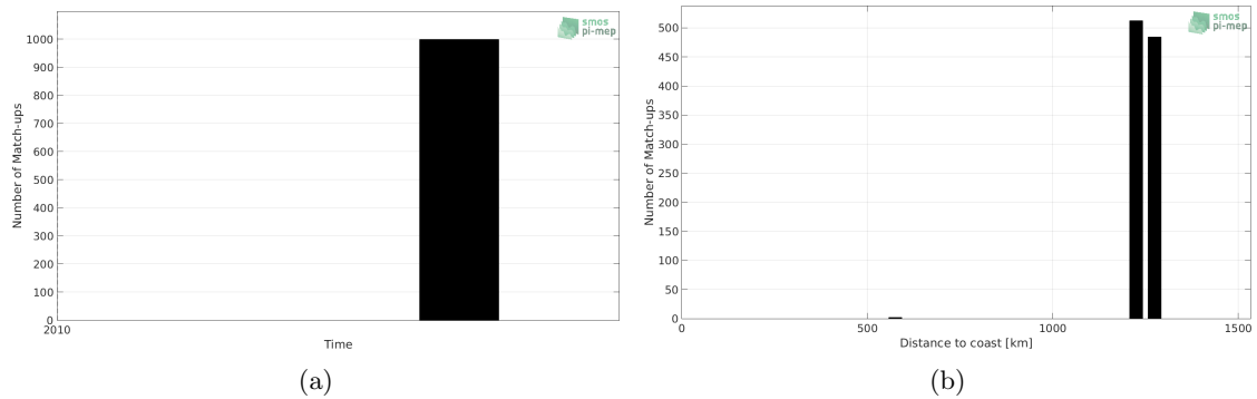
Figure 1: Number of match-ups between TSG-SAMOS and SMOS-L3-CATDS-CECOS-LOCEAN-V3-18DAYS-25KM SSS as a function of time (a) and as function of the distance to coast (b) over the Congo river plume Pi-MEP region and for the full satellite product period.
