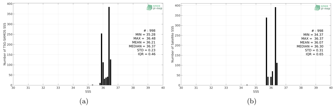
Figure 2: Histograms of SSS from TSG-SAMOS (a) and SMOS-L3-CATDS-CECOS-LOCEAN-V3-18DAYS-25KM (b) considering all match-up pairs per bins of 0.1 over the Congo river plume Pi-MEP region and for the full satellite product period.
