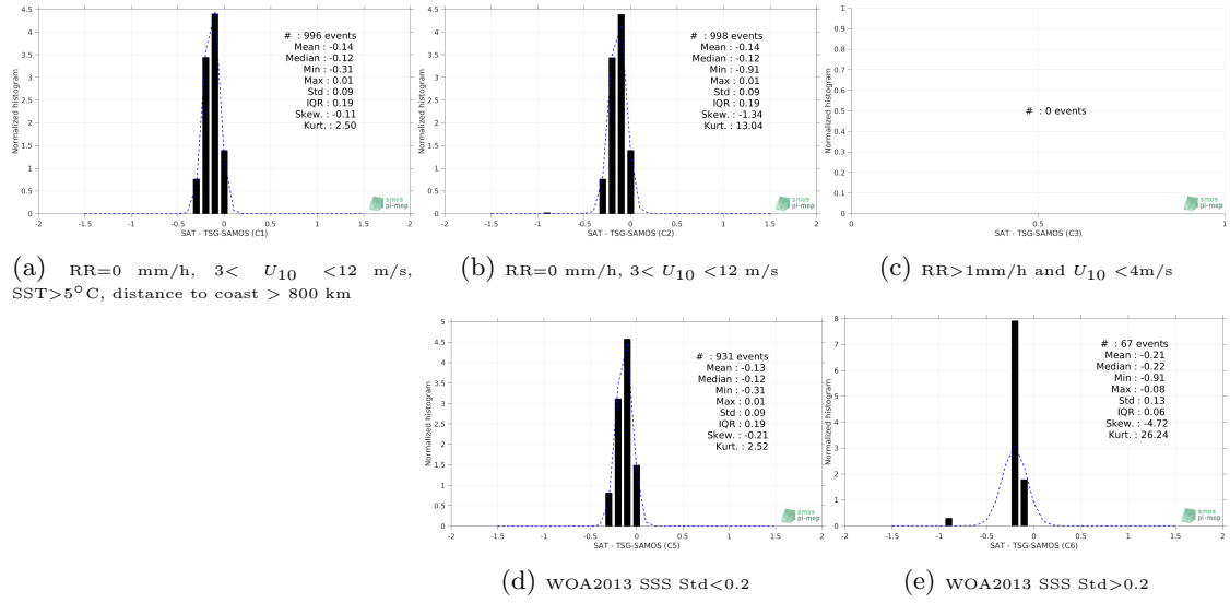
Figure 13: Normalized histogram of \Delta SSS (SMOS-L3-CATDS-CECOS-LOCEAN-V3-18DAYS-25KM - TSG-SAMOS) for 5 different subdatasets corresponding to: RR=0 mm/h, 3 < U_{10} < 12 m/s, SST > 5°C, distance to coast > 800 km (a), RR=0 mm/h, 3 < U_{10} < 12 m/s (b), RR > 1mm/h and U_{10} < 4 m/s (c), WOA2013 SSS Std < 0.2 (d), WOA2013 SSS Std > 0.2 (e).
