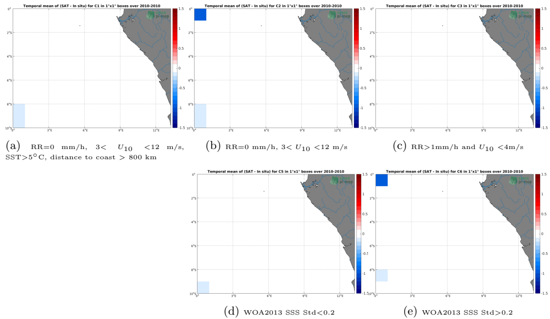
Figure 12: Temporal mean gridded over spatial boxes of size 1^\circ \times 1^\circ of \Delta SSS (SMOS-L3-CATDS-CECOS-LOCEAN-V3-18DAYS-25KM - TSG-SAMOS) for 5 different subdatasets corresponding to: RR=0 mm/h, 3 < U_{10} < 12 m/s, SST > 5^\circ C , distance to coast > 800 km (a), RR=0 mm/h, 3 < U_{10} < 12 m/s (b), RR > 1 mm/h and U_{10} < 4 m/s (c), WOA2013 SSS Std < 0.2 (d), WOA2013 SSS Std > 0.2 (e).
