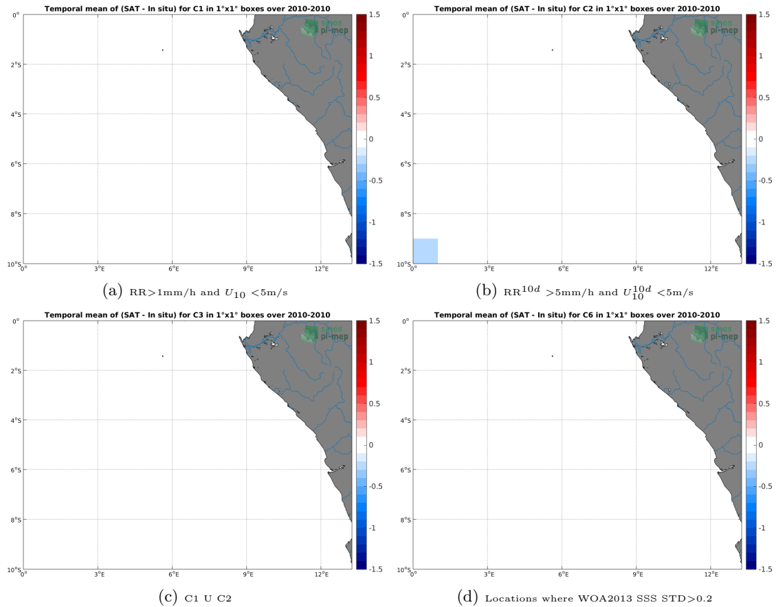
Figure 12: Temporal mean gridded over spatial boxes of size 1^\circ \times 1^\circ of \Delta SSS (SMOS-L3-CATDS-CECOS-LOCEAN-V3-18DAYS-25KM - TSG-SAMOS) for 4 different subdatasets corresponding to: RR > 1\text{mm/h} and U_{10} < 5\text{m/s} (a), RR^{10d} > 5\text{mm/h} and U_{10}^{10d} < 5\text{m/s} (b), C1 \cup C2 (c), Locations where WOA2013 SSS STD > 0.2 (d).
