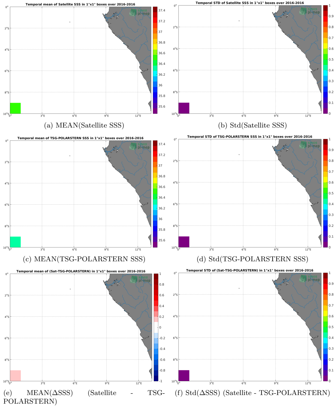
Figure 6: Temporal mean (left) and Std (right) of SSS from SMOS-L3-CATDS-CECOS-LOCEAN-V3-18DAYS-25KM (top), TSG-POLARSTERN (middle), and of \Delta SSS (Satellite - TSG-POLARSTERN). Only match-up pairs are used to generate these maps.
