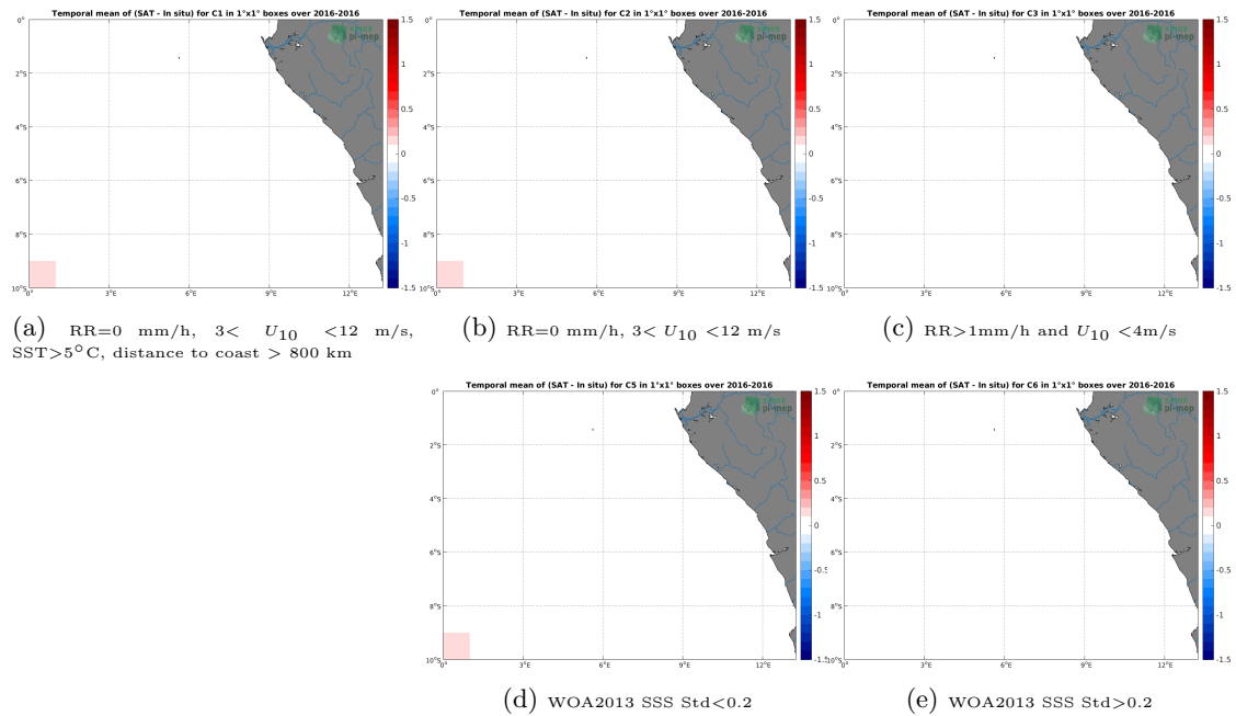
Figure 12: Temporal mean gridded over spatial boxes of size 1^\circ \times 1^\circ of \Delta SSS (SMOS-L3-CATDS-CECOS-LOCEAN-V3-18DAYS-25KM - TSG-POLARSTERN) for 5 different subdatasets corresponding to:RR=0 mm/h, 3 < U_{10} < 12 m/s, SST >5^\circ\text{C} , distance to coast > 800 km (a), RR=0 mm/h, 3 < U_{10} < 12 m/s (b), RR >1 mm/h and U_{10} < 4 m/s (c), WOA2013 SSS Std <0.2 (d), WOA2013 SSS Std >0.2 (e).
