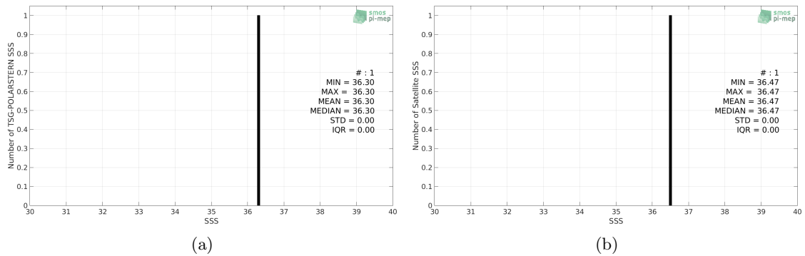
Figure 2: Histograms of SSS from TSG-POLARSTERN (a) and SMOS-L3-CATDS-CECOS-LOCEAN-V3-18DAYS-25KM (b) considering all match-up pairs per bins of 0.1 over the Congo river plume Pi-MEP region and for the full satellite product period.
