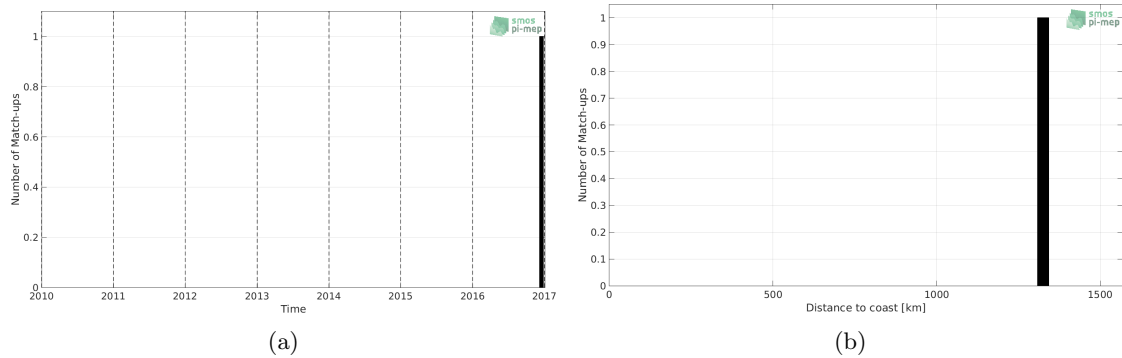
Figure 1: Number of match-ups between TSG-POLARSTERN and SMOS-L3-CATDS-CECOS-LOCEAN-V3-18DAYS-25KM SSS as a function of time (a) and as function of the distance to coast (b) over the Congo river plume Pi-MEP region and for the full satellite product period.
