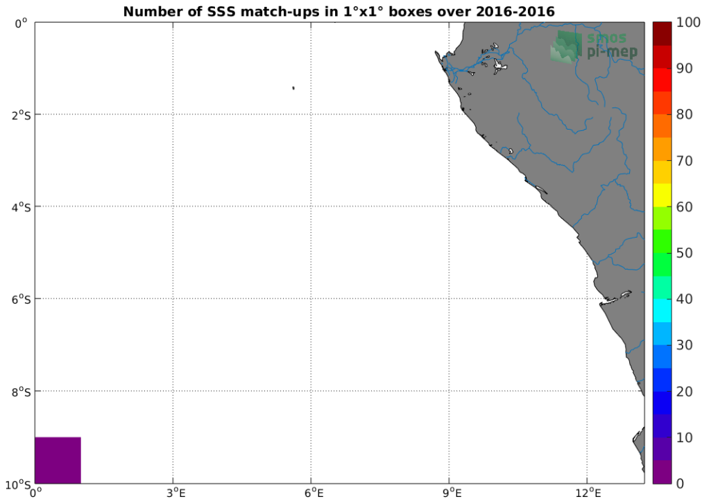
Figure 4: Number of SSS match-ups between TSG-POLARSTERN SSS and the SMOS-L3-CATDS-CECOS-LOCEAN-V3-18DAYS-25KM SSS product for the Congo river plume Pi-MEP region over 1°x1° boxes and for the full satellite product period.
