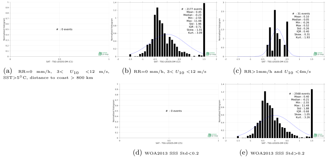
Figure 13: Normalized histogram of \Delta SSS (SMOS-L3-CATDS-CECOS-LOCEAN-V3-18DAYS-25KM - TSG-LEGOS-DM) for 5 different subdatasets corresponding to: RR=0 mm/h, 3 < U_{10} < 12 m/s, SST > 5°C, distance to coast > 800 km (a), RR=0 mm/h, 3 < U_{10} < 12 m/s (b), RR > 1mm/h and U_{10} < 4 m/s (c), WOA2013 SSS Std < 0.2 (d), WOA2013 SSS Std > 0.2 (e).
