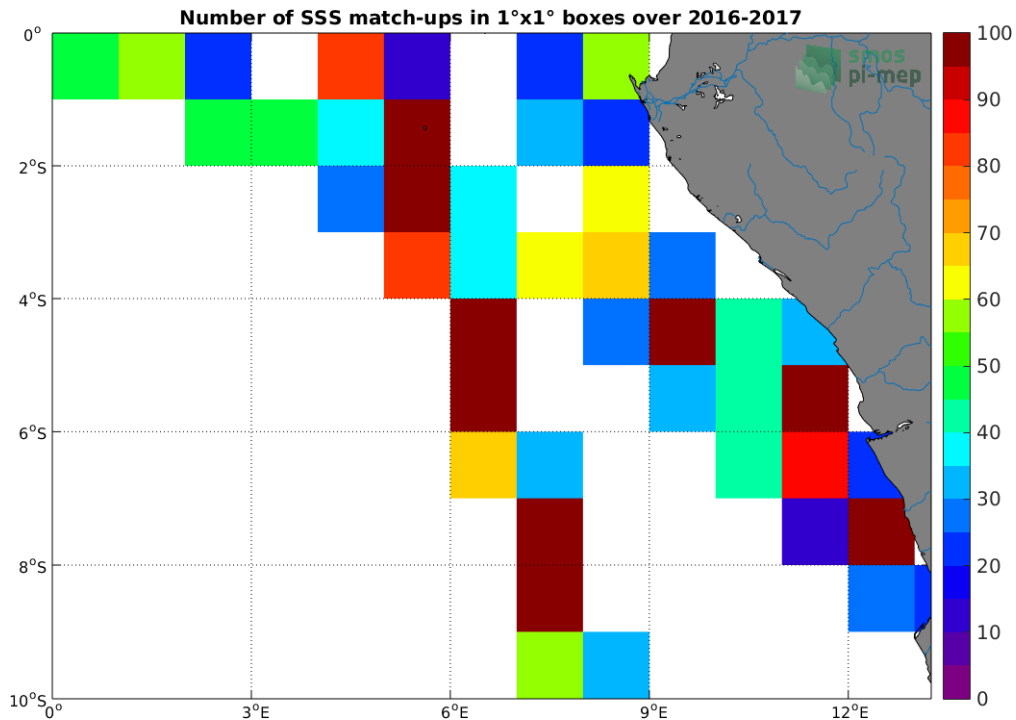
Figure 4: Number of SSS match-ups between TSG-LEGOS-DM SSS and the SMOS-L3-CATDS-CECOS-LOCEAN-V3-18DAYS-25KM SSS product for the Congo river plume Pi-MEP region over 1^\circ \times 1^\circ boxes and for the full satellite product period.
