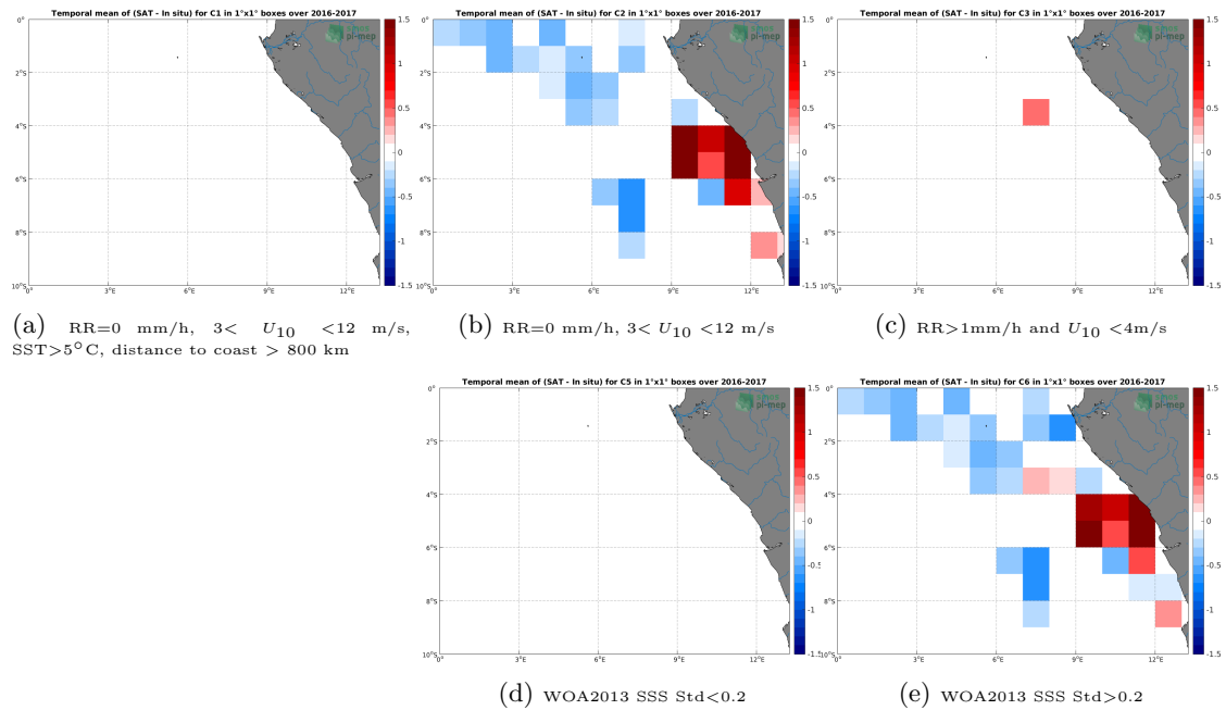
Figure 12: Temporal mean gridded over spatial boxes of size 1^\circ \times 1^\circ of \Delta SSS (SMOS-L3-CATDS-CECOS-LOCEAN-V3-18DAYS-25KM - TSG-LEGOS-DM) for 5 different subdatasets corresponding to:RR=0 mm/h, 3 < U_{10} < 12 m/s, SST > 5^\circ\text{C} , distance to coast > 800 km (a), RR=0 mm/h, 3 < U_{10} < 12 m/s (b), RR > 1 mm/h and U_{10} < 4 m/s (c), WOA2013 SSS Std < 0.2 (d), WOA2013 SSS Std > 0.2 (e).
