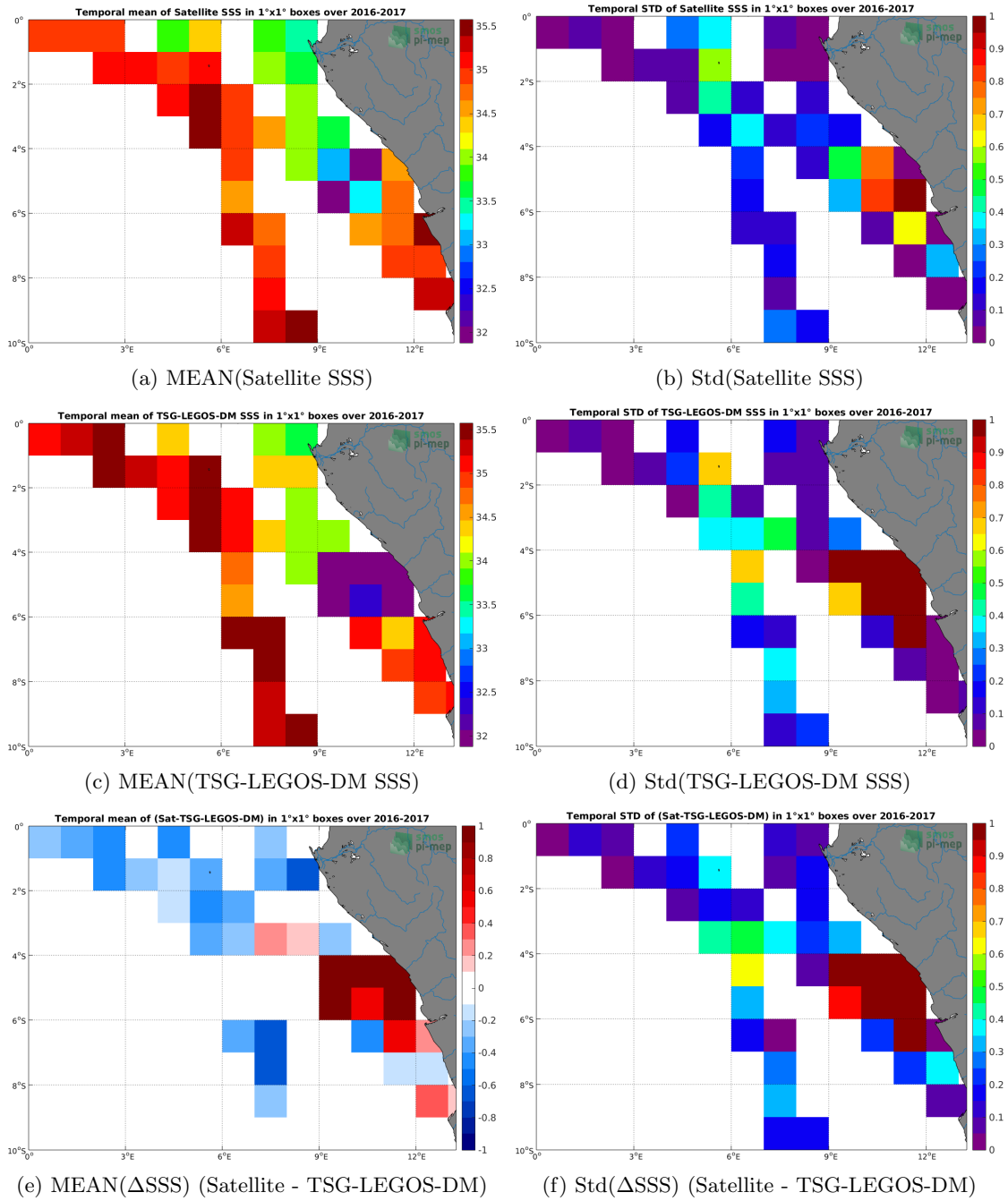
Figure 6: Temporal mean (left) and Std (right) of SSS from SMOS-L3-CATDS-CECOS-LOCEAN-V3-18DAYS-25KM (top), TSG-LEGOS-DM (middle), and of \Delta SSS (Satellite - TSG-LEGOS-DM). Only match-up pairs are used to generate these maps.
