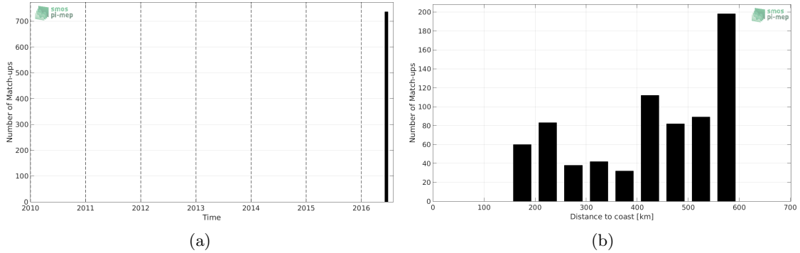
Figure 1: Number of match-ups between TSG-LEGOS-DM and SMOS-L3-CATDS-CECOS-LOCEAN-V3-18DAYS-25KM SSS as a function of time (a) and as function of the distance to coast (b) over the Congo river plume Pi-MEP region and for the full satellite product period.
