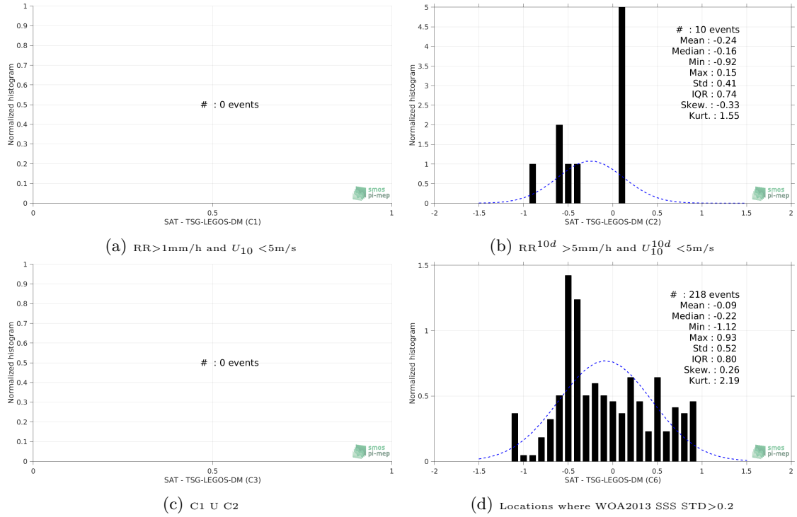
Figure 13: Normalized histogram of \Delta\text{SSS} (SMOS-L3-CATDS-CECOS-LOCEAN-V3-18DAYS-25KM - TSG-LEGOS-DM) for 6 different subdatasets corresponding to: RR > 1\text{mm/h} and U_{10} < 5\text{m/s} (a), RR^{10d} > 5\text{mm/h} and U_{10}^{10d} < 5\text{m/s} (b), C1 U C2 (c), Locations where WOA2013 SSS STD > 0.2 (d).
