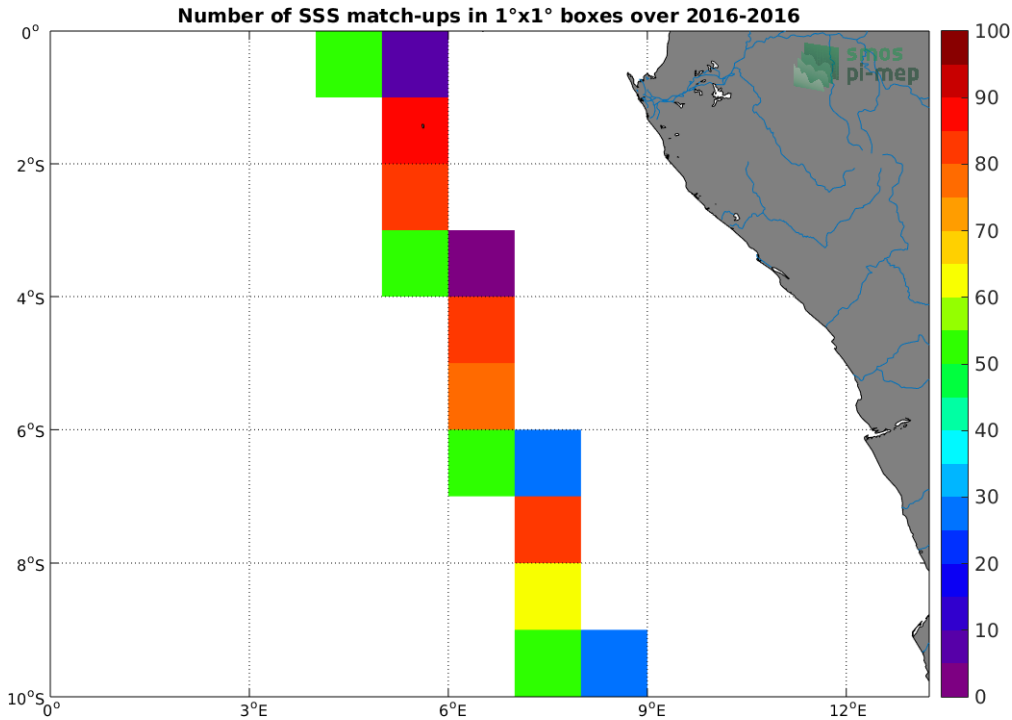
Figure 4: Number of SSS match-ups between TSG-LEGOS-DM SSS and the SMOS-L3-CATDS-CECOS-LOCEAN-V3-18DAYS-25KM SSS product for the Congo river plume Pi-MEP region over 1°x1° boxes and for the full satellite product period.
