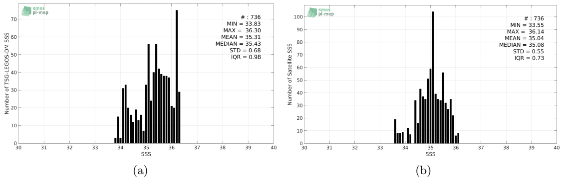
Figure 2: Histograms of SSS from TSG-LEGOS-DM (a) and SMOS-L3-CATDS-CECOS-LOCEAN-V3-18DAYS-25KM (b) considering all match-up pairs per bins of 0.1 over the Congo river plume Pi-MEP region and for the full satellite product period.
