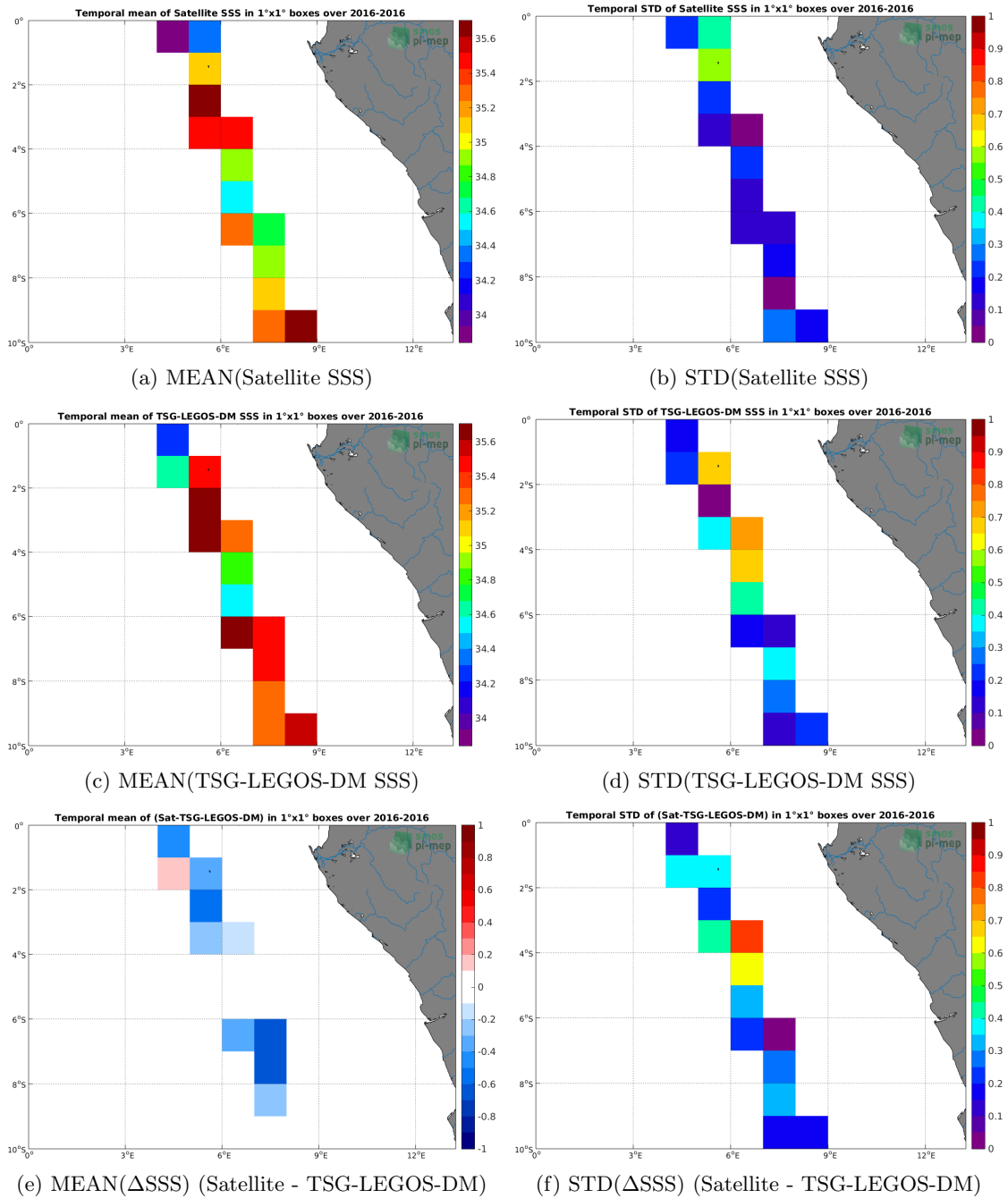
Figure 6: Temporal mean (left) and STD (right) of SSS from SMOS-L3-CATDS-CECOS-LOCEAN-V3-18DAYS-25KM (top), TSG-LEGOS-DM (middle), and of \Delta SSS (Satellite - TSG-LEGOS-DM). Only match-up pairs are used to generate these maps.
