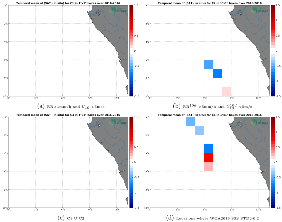
Figure 12: Temporal mean gridded over spatial boxes of size 1^\circ \times 1^\circ of \Delta SSS (SMOS-L3-CATDS-CECOS-LOCEAN-V3-18DAYS-25KM - TSG-LEGOS-DM) for 4 different subdatasets corresponding to: RR > 1\text{mm/h} and U_{10} < 5\text{m/s} (a), RR^{10d} > 5\text{mm/h} and U_{10}^{10d} < 5\text{m/s} (b), C1 \cup C2 (c), Locations where WOA2013 SSS STD > 0.2 (d).
