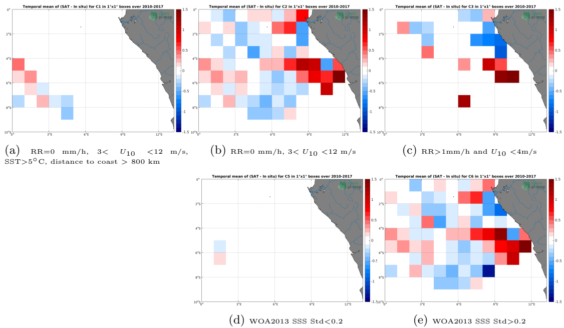
Figure 12: Temporal mean gridded over spatial boxes of size 1^\circ \times 1^\circ of \Delta SSS (SMOS-L3-CATDS-CECOS-LOCEAN-V3-18DAYS-25KM - TSG-GOSUD-Research-vessel) for 5 different subdatasets corresponding to:RR=0 mm/h, 3 < U_{10} < 12 m/s, SST>5°C, distance to coast > 800 km (a), RR=0 mm/h, 3 < U_{10} < 12 m/s (b), RR>1mm/h and U_{10} < 4 m/s (c), WOA2013 SSS Std<0.2 (d), WOA2013 SSS Std>0.2 (e).
