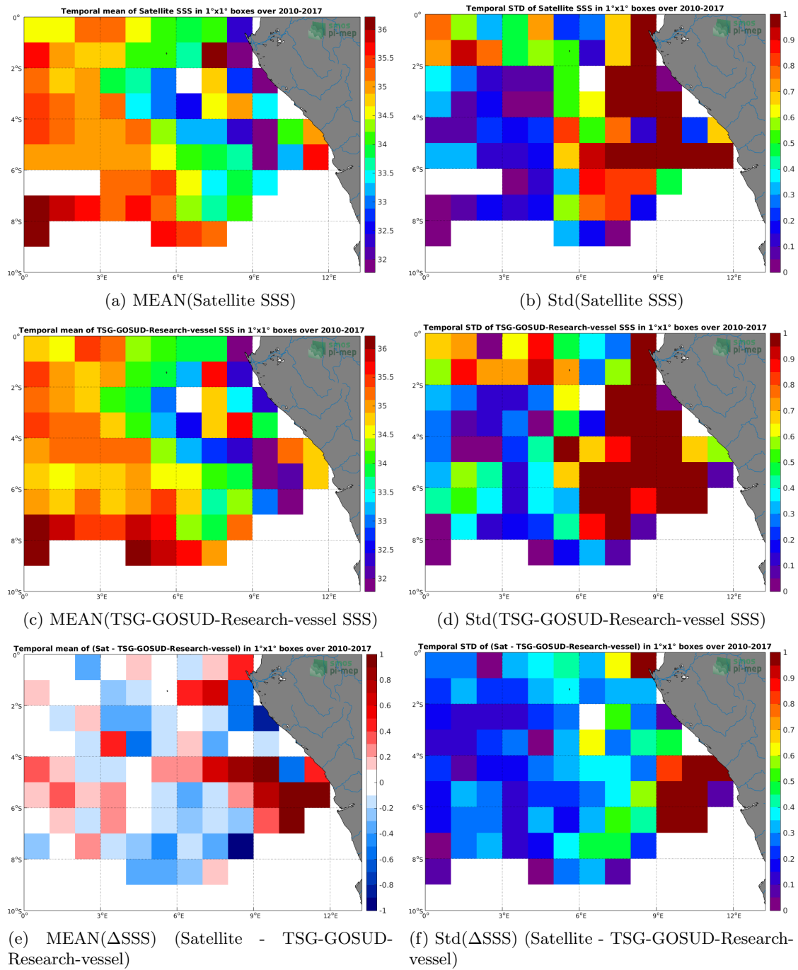
Figure 6: Temporal mean (left) and Std (right) of SSS from SMOS-L3-CATDS-CECOS-LOCEAN-V3-18DAYS-25KM (top), TSG-GOSUD-Research-vessel (middle), and of \Delta SSS (Satellite - TSG-GOSUD-Research-vessel). Only match-up pairs are used to generate these maps.
