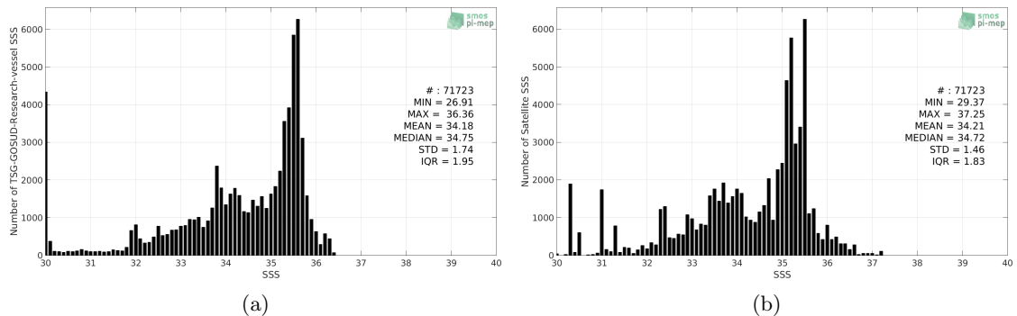
Figure 2: Histograms of SSS from TSG-GOSUD-Research-vessel (a) and SMOS-L3-CATDS-CECOS-LOCEAN-V3-18DAYS-25KM (b) considering all match-up pairs per bins of 0.1 over the Congo river plume Pi-MEP region and for the full satellite product period.
