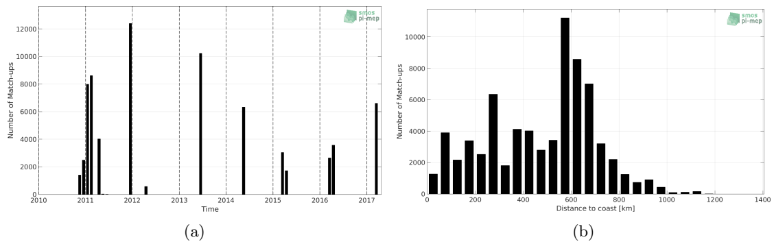
Figure 1: Number of match-ups between TSG-GOSUD-Research-vessel and SMOS-L3-CATDS-CECOS-LOCEAN-V3-18DAYS-25KM SSS as a function of time (a) and as function of the distance to coast (b) over the Congo river plume Pi-MEP region and for the full satellite product period.
