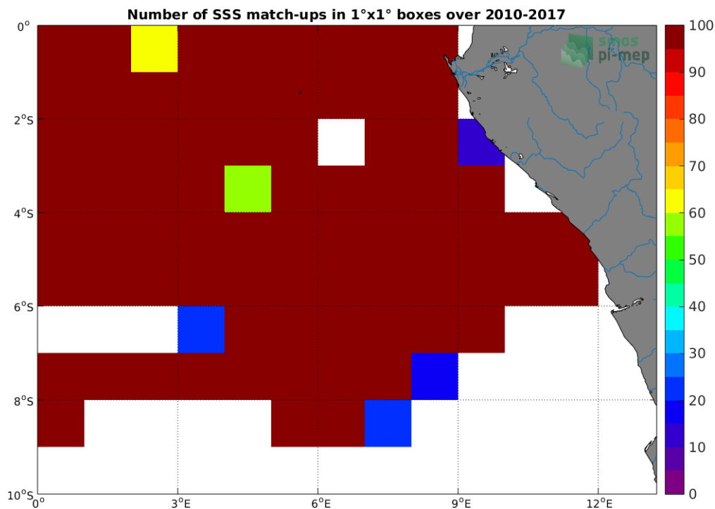
Figure 4: Number of SSS match-ups between TSG-GOSUD-Research-vessel SSS and the SMOS-L3-CATDS-CECOS-LOCEAN-V3-18DAYS-25KM SSS product for the Congo river plume Pi-MEP region over 1^\circ \times 1^\circ boxes and for the full satellite product period.
