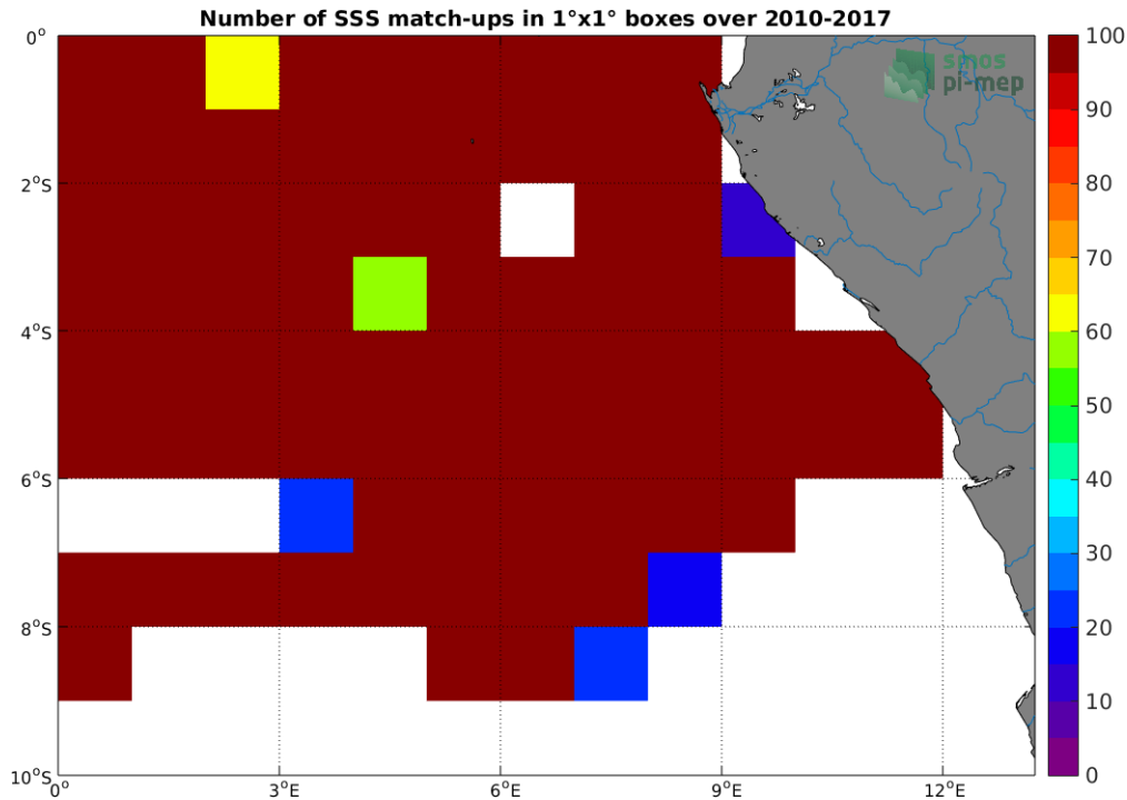
Figure 4: Number of SSS match-ups between TSG-GOSUD-Research-vessel SSS and the SMOS-L3-CATDS-CECOS-LOCEAN-V3-18DAYS-25KM SSS product for the Congo river plume Pi-MEP region over 1°x1° boxes and for the full satellite product period.
