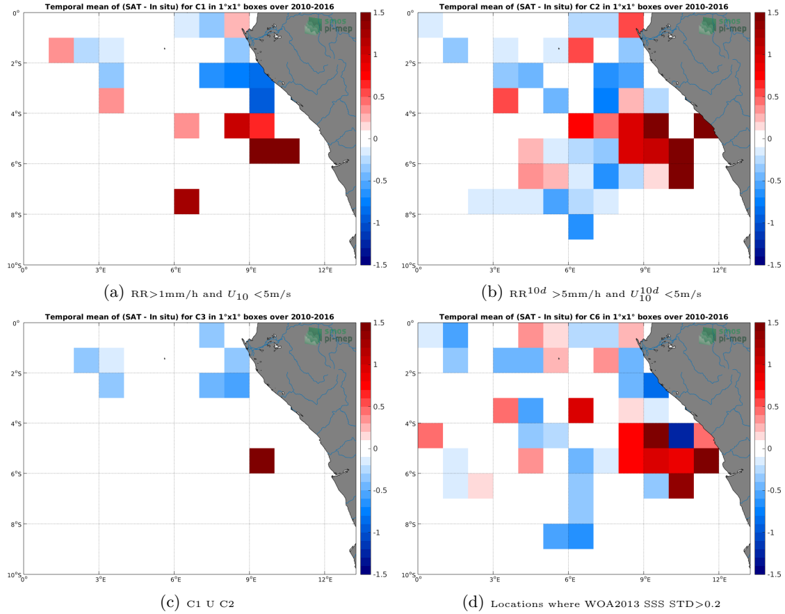
Figure 12: Temporal mean gridded over spatial boxes of size 1^\circ \times 1^\circ of \Delta SSS (SMOS-L3-CATDS-CECOS-LOCEAN-V3-18DAYS-25KM - TSG-GOSUD-Research-vessel) for 4 different subdatasets corresponding to: RR > 1\text{mm/h} and U_{10} < 5\text{m/s} (a), RR^{10d} > 5\text{mm/h} and U_{10}^{10d} < 5\text{m/s} (b), C1 \cup C2 (c), Locations where WOA2013 SSS STD > 0.2 (d).
