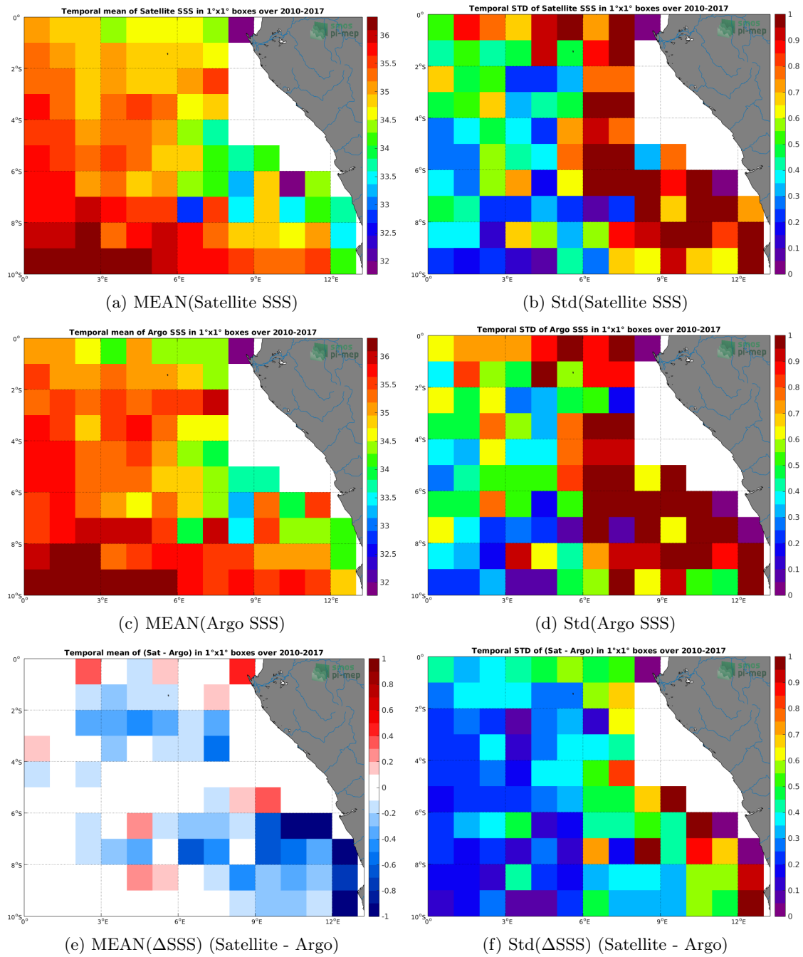
Figure 6: Temporal mean (left) and Std (right) of SSS from SMOS-L3-CATDS-CECOS-LOCEAN-V3-18DAYS-25KM (top), Argo (middle), and of \Delta SSS (Satellite - Argo). Only match-up pairs are used to generate these maps.
