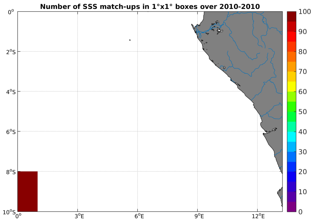
Figure 4: Number of SSS match-ups between TSG-SAMOS SSS and the SMOS-L3-CATDS-CECOS-LOCEAN-V2-9DAYS-25KM SSS product for the Congo river plume Pi-MEP region over 1°x1° boxes and for the full satellite product period.
