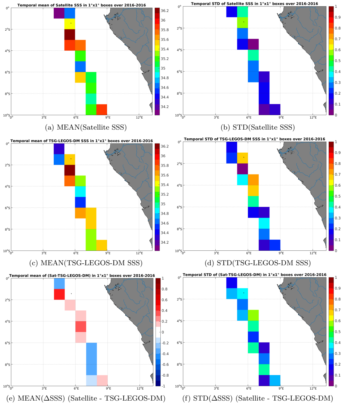
Figure 6: Temporal mean (left) and STD (right) of SSS from SMOS-L3-CATDS-CECOS-LOCEAN-V2-9DAYS-25KM (top), TSG-LEGOS-DM (middle), and of \Delta SSS (Satellite - TSG-LEGOS-DM). Only match-up pairs are used to generate these maps.
