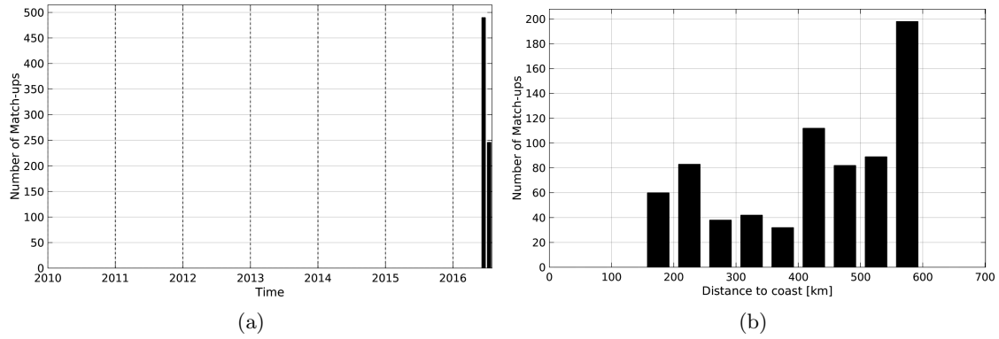
Figure 1: Number of match-ups between TSG-LEGOS-DM and SMOS-L3-CATDS-CECOS-LOCEAN-V2-9DAYS-25KM SSS as a function of time (a) and as function of the distance to coast (b) over the Congo river plume Pi-MEP region and for the full satellite product period.
