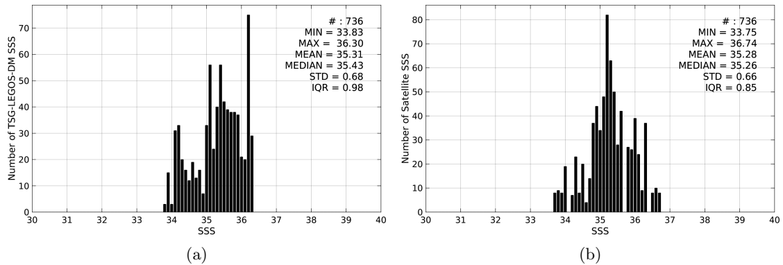
Figure 2: Histograms of SSS from TSG-LEGOS-DM (a) and SMOS-L3-CATDS-CECOS-LOCEAN-V2-9DAYS-25KM (b) considering all match-up pairs per bins of 0.1 over the Congo river plume Pi-MEP region and for the full satellite product period.
