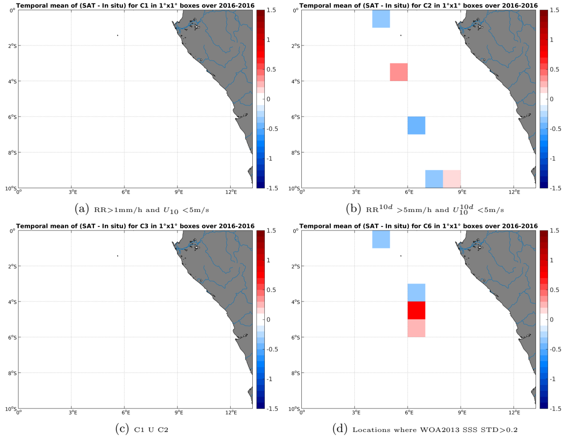
Figure 12: Temporal mean gridded over spatial boxes of size 1^\circ \times 1^\circ of \Delta SSS (SMOS-L3-CATDS-CECOS-LOCEAN-V2-9DAYS-25KM - TSG-LEGOS-DM) for 4 different subdatasets corresponding to: RR > 1\text{mm/h} and U_{10} < 5\text{m/s} (a), RR^{10d} > 5\text{mm/h} and U_{10}^{10d} < 5\text{m/s} (b), C1 \cup C2 (c), Locations where WOA2013 SSS STD > 0.2 (d).
