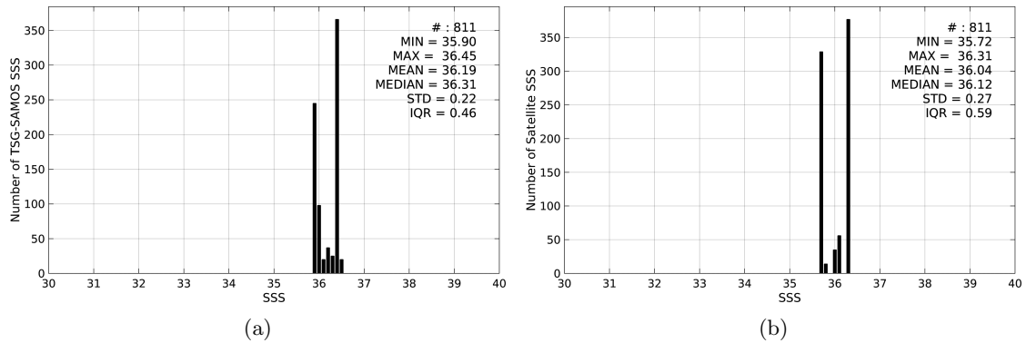
Figure 2: Histograms of SSS from TSG-SAMOS (a) and SMOS-L3-CATDS-CECOS-LOCEAN-V2-18DAYS-25KM (b) considering all match-up pairs per bins of 0.1 over the Congo river plume Pi-MEP region and for the full satellite product period.
