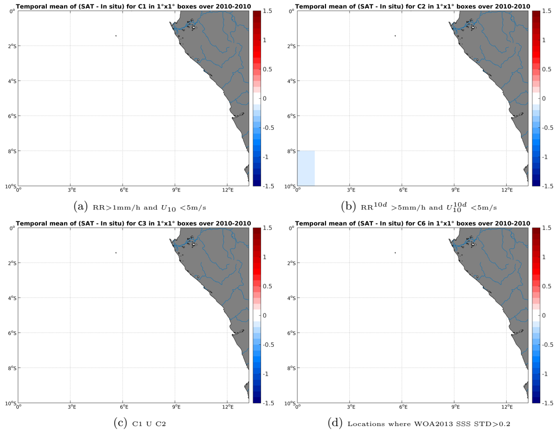
Figure 12: Temporal mean gridded over spatial boxes of size 1^\circ \times 1^\circ of \Delta SSS (SMOS-L3-CATDS-CECOS-LOCEAN-V2-18DAYS-25KM - TSG-SAMOS) for 4 different subdatasets corresponding to: RR > 1\text{mm/h} and U_{10} < 5\text{m/s} (a), RR^{10d} > 5\text{mm/h} and U_{10}^{10d} < 5\text{m/s} (b), C1 \cup C2 (c), Locations where WOA2013 SSS STD > 0.2 (d).
