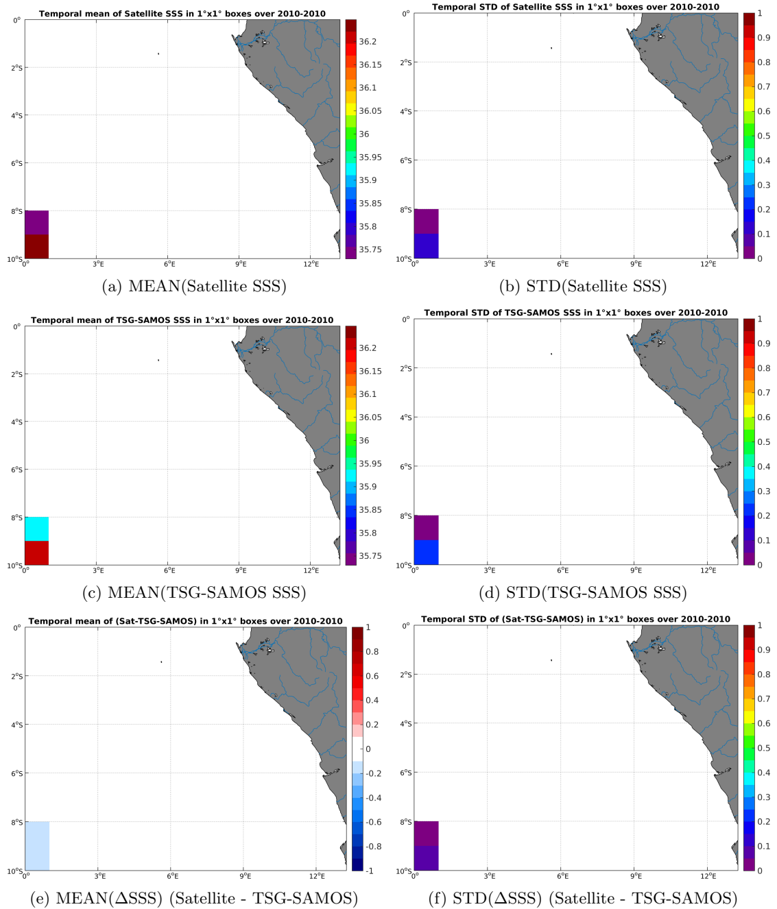
Figure 6: Temporal mean (left) and STD (right) of SSS from SMOS-L3-CATDS-CECOS-LOCEAN-V2-18DAYS-25KM (top), TSG-SAMOS (middle), and of \Delta SSS (Satellite - TSG-SAMOS). Only match-up pairs are used to generate these maps.
