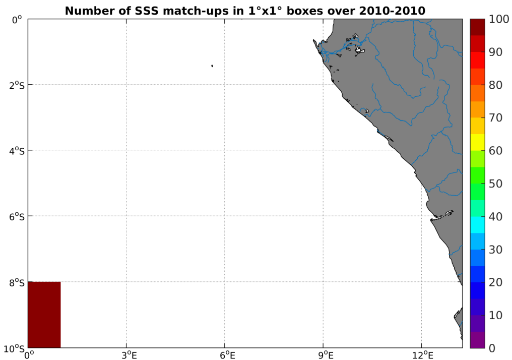
Figure 4: Number of SSS match-ups between TSG-SAMOS SSS and the SMOS-L3-CATDS-CECOS-LOCEAN-V2-18DAYS-25KM SSS product for the Congo river plume Pi-MEP region over 1^\circ \times 1^\circ boxes and for the full satellite product period.
