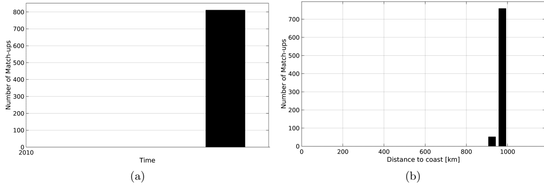
Figure 1: Number of match-ups between TSG-SAMOS and SMOS-L3-CATDS-CECOS-LOCEAN-V2-18DAYS-25KM SSS as a function of time (a) and as function of the distance to coast (b) over the Congo river plume Pi-MEP region and for the full satellite product period.
