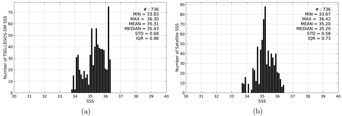
Figure 2: Histograms of SSS from TSG-LEGOS-DM (a) and SMOS-L3-CATDS-CECOS-LOCEAN-V2-18DAYS-25KM (b) considering all match-up pairs per bins of 0.1 over the Congo river plume Pi-MEP region and for the full satellite product period.
