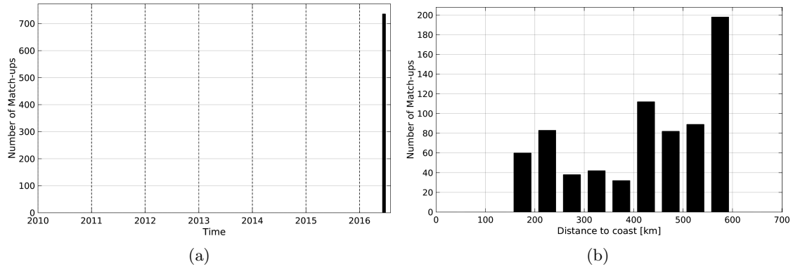
Figure 1: Number of match-ups between TSG-LEGOS-DM and SMOS-L3-CATDS-CECOS-LOCEAN-V2-18DAYS-25KM SSS as a function of time (a) and as function of the distance to coast (b) over the Congo river plume Pi-MEP region and for the full satellite product period.
