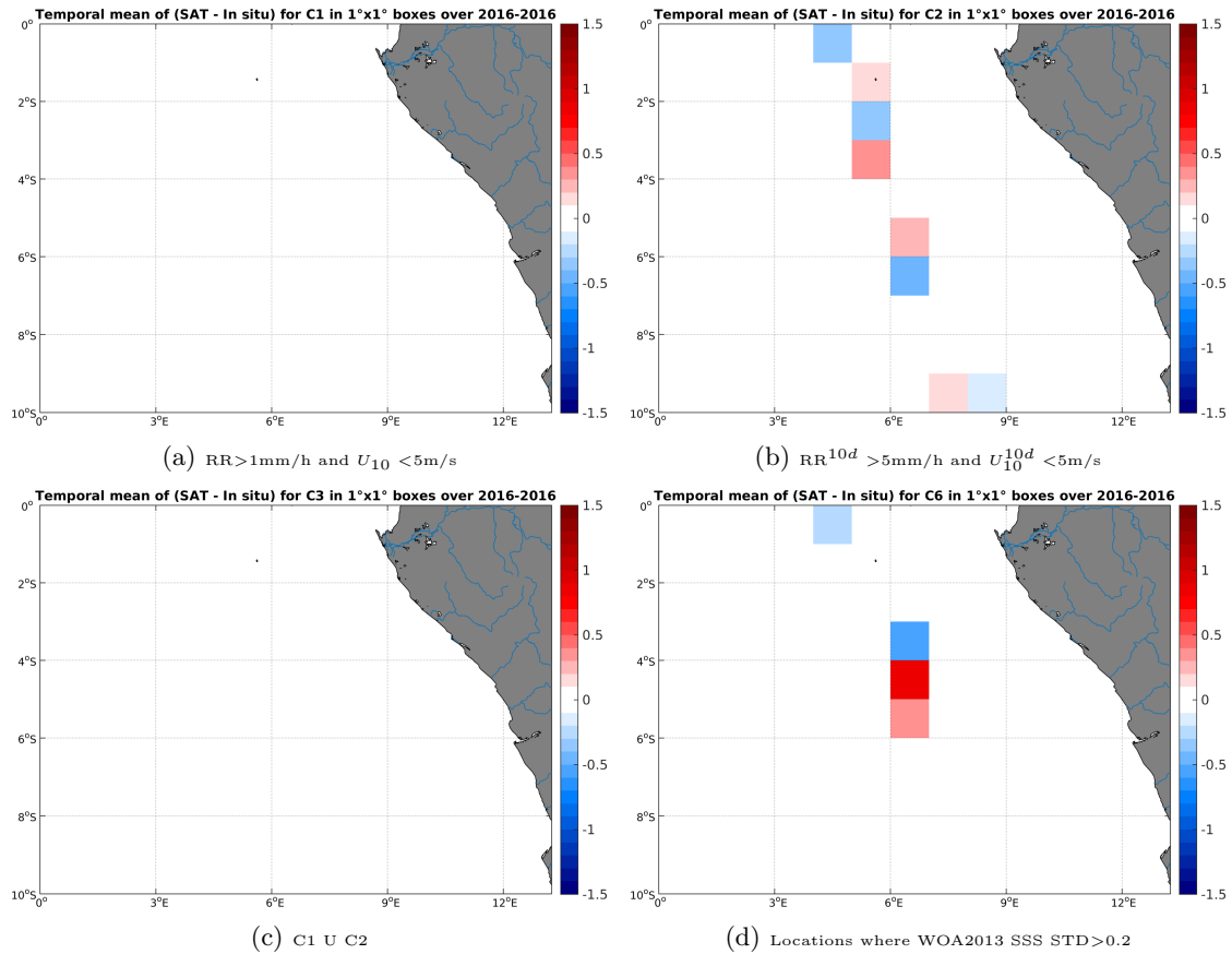
Figure 12: Temporal mean gridded over spatial boxes of size 1^\circ \times 1^\circ of \Delta SSS (SMOS-L3-CATDS-CECOS-LOCEAN-V2-18DAYS-25KM - TSG-LEGOS-DM) for 4 different subdatasets corresponding to: RR > 1\text{mm/h} and U_{10} < 5\text{m/s} (a), RR^{10d} > 5\text{mm/h} and U_{10}^{10d} < 5\text{m/s} (b), C1 \cup C2 (c), Locations where WOA2013 SSS STD > 0.2 (d).
