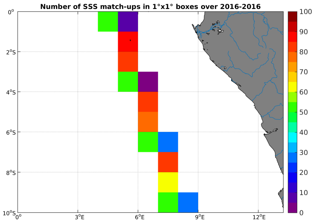
Figure 4: Number of SSS match-ups between TSG-LEGOS-DM SSS and the SMOS-L3-CATDS-CECOS-LOCEAN-V2-18DAYS-25KM SSS product for the Congo river plume Pi-MEP region over 1^\circ \times 1^\circ boxes and for the full satellite product period.
