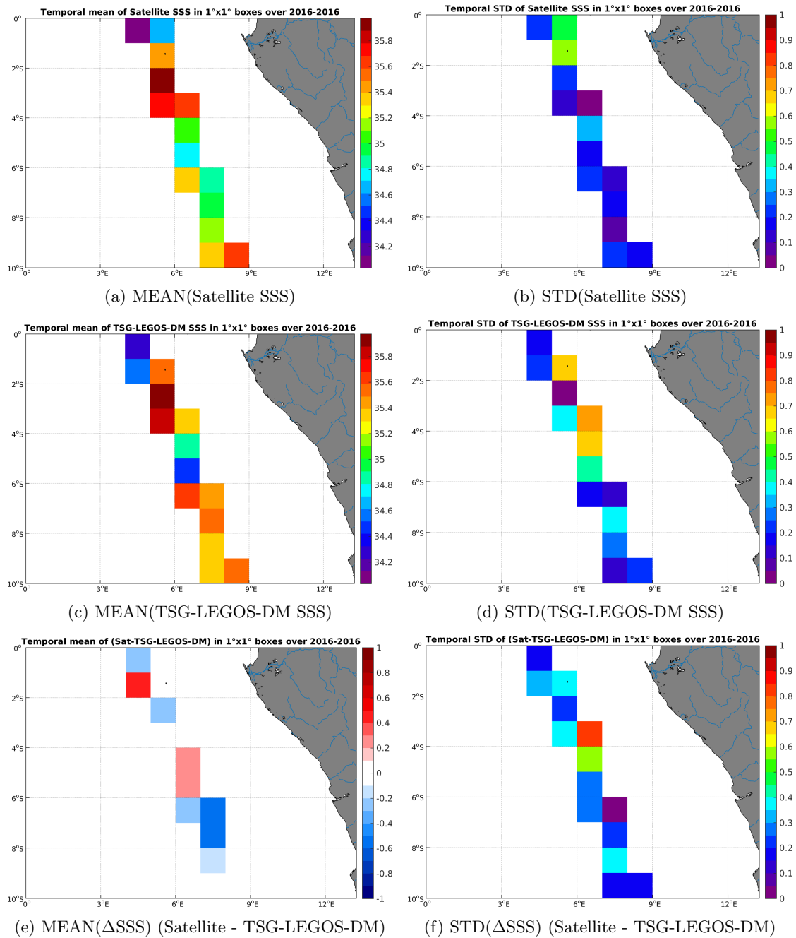
Figure 6: Temporal mean (left) and STD (right) of SSS from SMOS-L3-CATDS-CECOS-LOCEAN-V2-18DAYS-25KM (top), TSG-LEGOS-DM (middle), and of \Delta SSS (Satellite - TSG-LEGOS-DM). Only match-up pairs are used to generate these maps.
