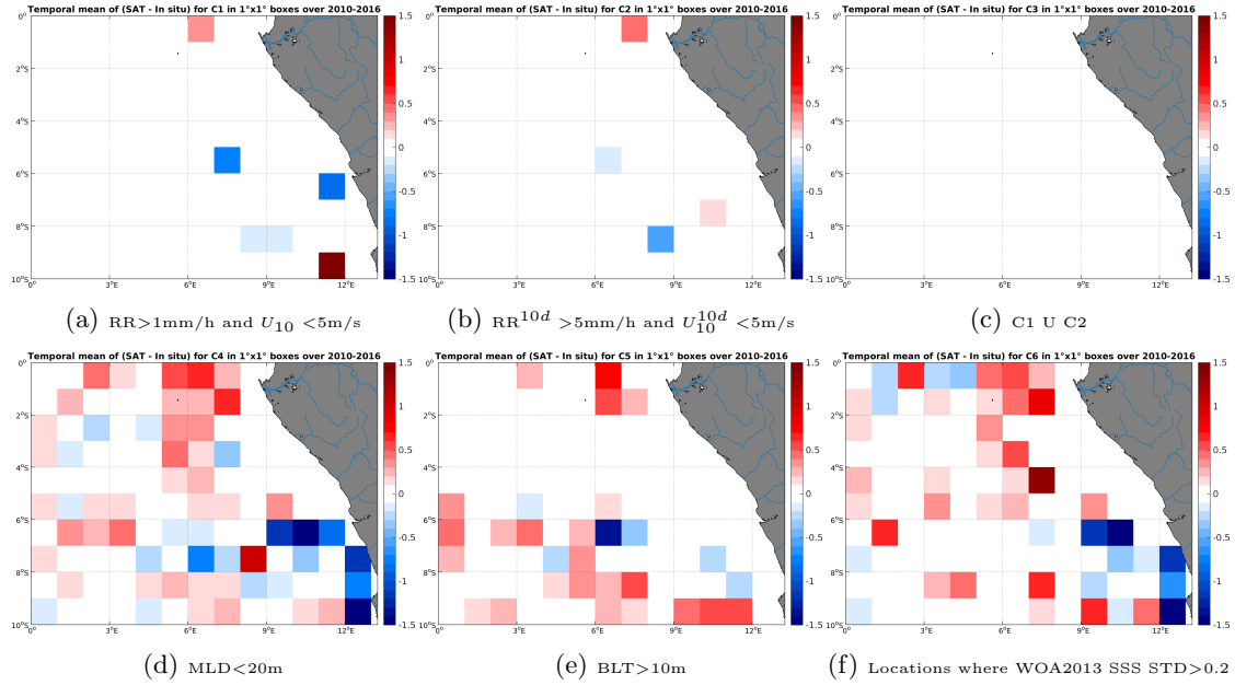
Figure 12: Temporal mean gridded over spatial boxes of size 1^\circ \times 1^\circ of \Delta SSS (SMOS-L3-CATDS-CECOS-LOCEAN-V2-18DAYS-25KM - Argo) for 6 different subdatasets corresponding to: RR > 1\text{mm/h} and U_{10} < 5\text{m/s} (a), RR^{10d} > 5\text{mm/h} and U_{10}^{10d} < 5\text{m/s} (b), C1 U C2 (c), MLD < 20\text{m} (d), BLT > 10\text{m} (e), Locations where WOA2013 SSS STD > 0.2 (f).
