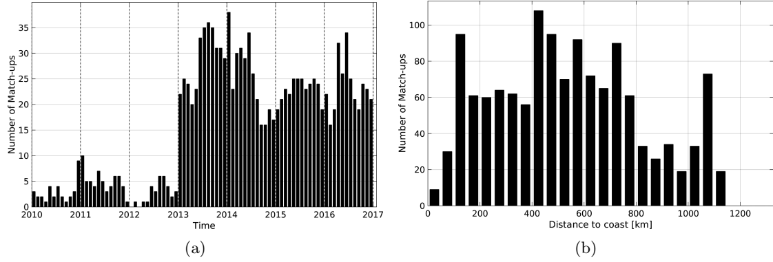
Figure 1: Number of match-ups between Argo and SMOS-L3-CATDS-CECOS-LOCEAN-V2-18DAYS-25KM SSS as a function of time (a) and as function of the distance to coast (b) over the Congo river plume Pi-MEP region and for the full satellite product period.
