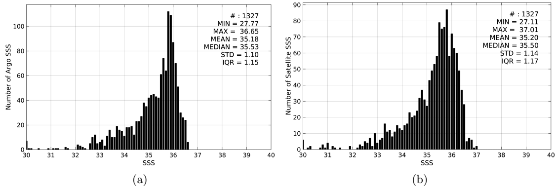
Figure 2: Histograms of SSS from Argo (a) and SMOS-L3-CATDS-CECOS-LOCEAN-V2-18DAYS-25KM (b) considering all match-up pairs per bins of 0.1 over the Congo river plume Pi-MEP region and for the full satellite product period.
