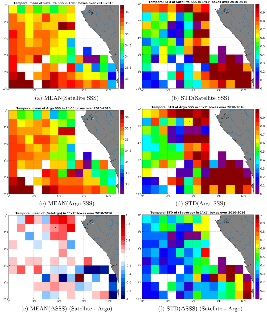
Figure 6: Temporal mean (left) and STD (right) of SSS from SMOS-L3-CATDS-CECOS-LOCEAN-V2-18DAYS-25KM (top), Argo (middle), and of \Delta SSS (Satellite - Argo). Only match-up pairs are used to generate these maps.
