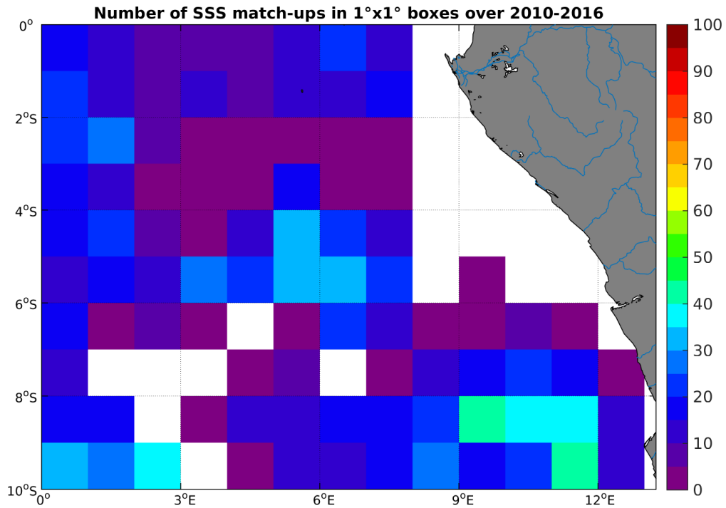
Figure 4: Number of SSS match-ups between Argo SSS and the SMOS-L3-CATDS-CECOS-LOCEAN-V2-18DAYS-25KM SSS product for the Congo river plume Pi-MEP region over 1^\circ \times 1^\circ boxes and for the full satellite product period.
