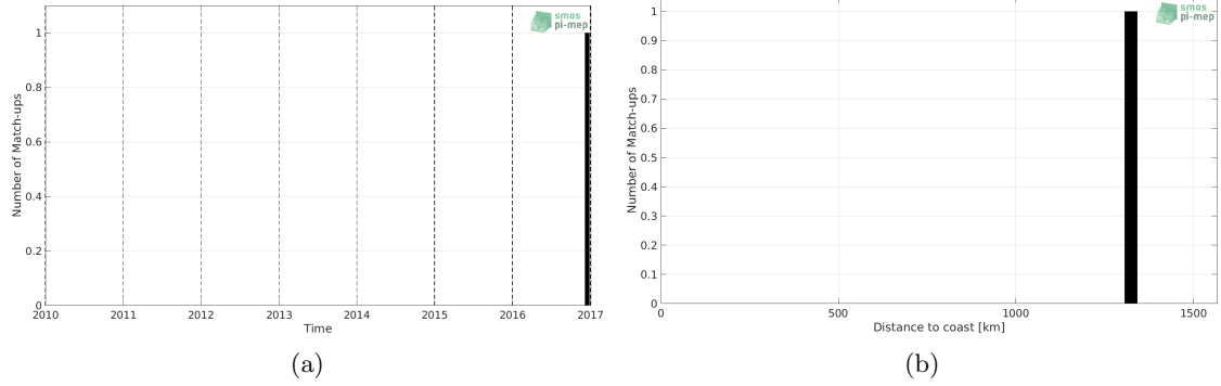
Figure 1: Number of match-ups between TSG (Polarstern) and SMOS SSS L3 v2 - Monthly - 0.25 Deg (CATDS-CECOS-IFREMER) SSS as a function of time (a) and as function of the distance to coast (b) over the Congo river plume Pi-MEP region and for the full satellite product period.
