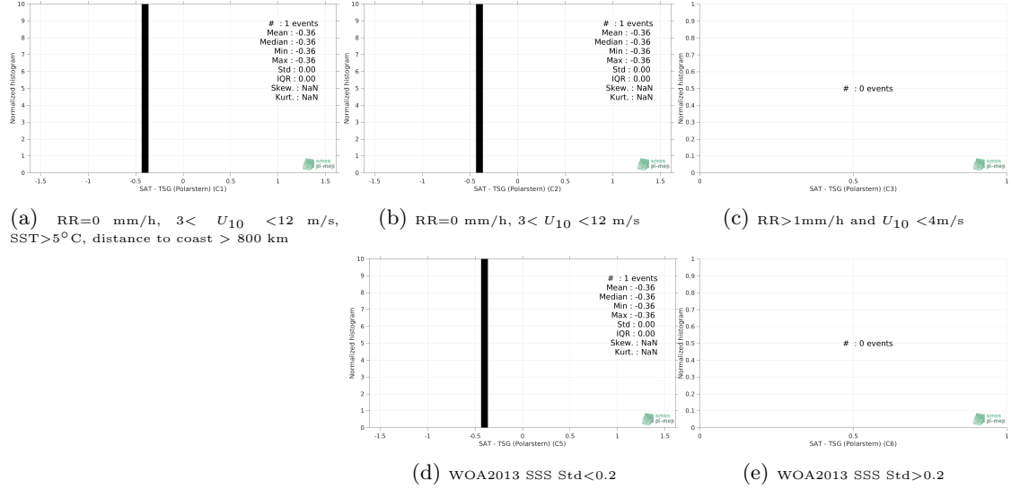
Figure 13: Normalized histogram of \Delta\text{SSS} (SMOS SSS L3 v2 - Monthly - 0.25 Deg (CATDS-CECOS-IFREMER) - TSG (Polarstern)) for 5 different subdatasets corresponding to: RR=0 mm/h, 3 < U_{10} < 12 m/s, SST > 5^\circ\text{C} , distance to coast > 800 km (a), RR=0 mm/h, 3 < U_{10} < 12 m/s (b), RR > 1\text{mm/h} and U_{10} < 4\text{m/s} (c), WOA2013 SSS Std < 0.2 (d), WOA2013 SSS Std > 0.2 (e).
