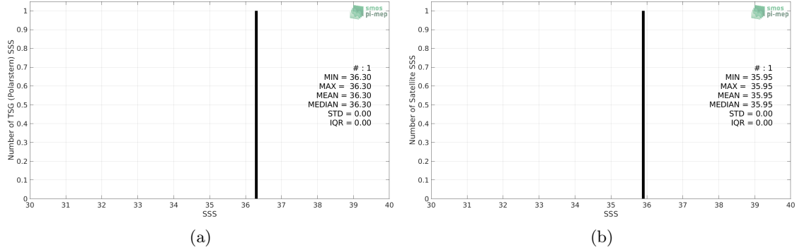
Figure 2: Histograms of SSS from TSG (Polarstern) (a) and SMOS SSS L3 v2 - Monthly - 0.25 Deg (CATDS-CECOS-IFREMER) (b) considering all match-up pairs per bins of 0.1 over the Congo river plume Pi-MEP region and for the full satellite product period.
