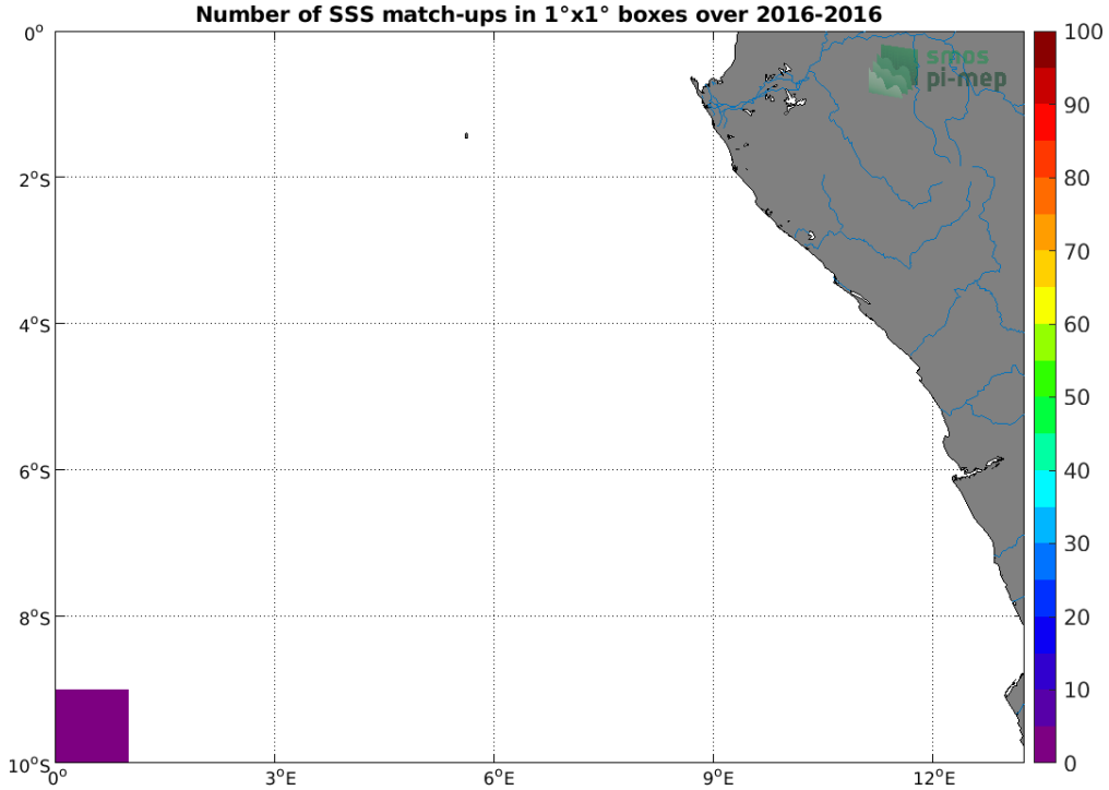
Figure 4: Number of SSS match-ups between TSG (Polarstern) SSS and the SMOS SSS L3 v2 - Monthly - 0.25 Deg (CATDS-CECOS-IFREMER) SSS product for the Congo river plume Pi-MEP region over 1^\circ \times 1^\circ boxes and for the full satellite product period.
