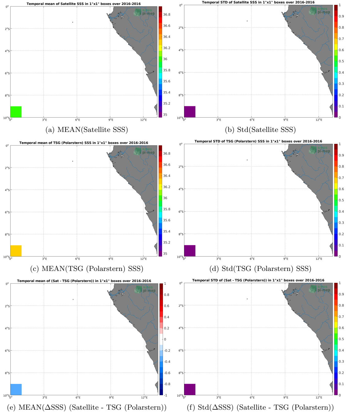
Figure 6: Temporal mean (left) and Std (right) of SSS from SMOS SSS L3 v2 - Monthly - 0.25 Deg (CATDS-CECOS-IFREMER) (top), TSG (Polarstern) (middle), and of \Delta SSS (Satellite - TSG (Polarstern)). Only match-up pairs are used to generate these maps.
