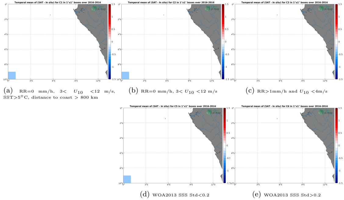
Figure 12: Temporal mean gridded over spatial boxes of size 1^{\circ}\times 1^{\circ} of \Delta\text{SSS} (SMOS SSS L3 v2 - Monthly - 0.25 Deg (CATDS-CECOS-IFREMER) - TSG (Polarstern)) for 5 different subdatasets corresponding to:RR=0 mm/h, 3 < U_{10} < 12 m/s, SST >5^{\circ}\text{C} , distance to coast > 800 km (a), RR=0 mm/h, 3 < U_{10} < 12 m/s (b), RR >1 mm/h and U_{10} < 4 m/s (c), WOA2013 SSS Std <0.2 (d), WOA2013 SSS Std >0.2 (e).
