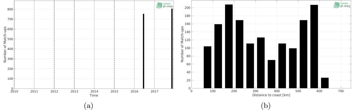
Figure 1: Number of match-ups between TSG (LEGOS-DM) and SMOS SSS L3 v2 - Monthly - 0.25 Deg (CATDS-CECOS-IFREMER) SSS as a function of time (a) and as function of the distance to coast (b) over the Congo river plume Pi-MEP region and for the full satellite product period.
