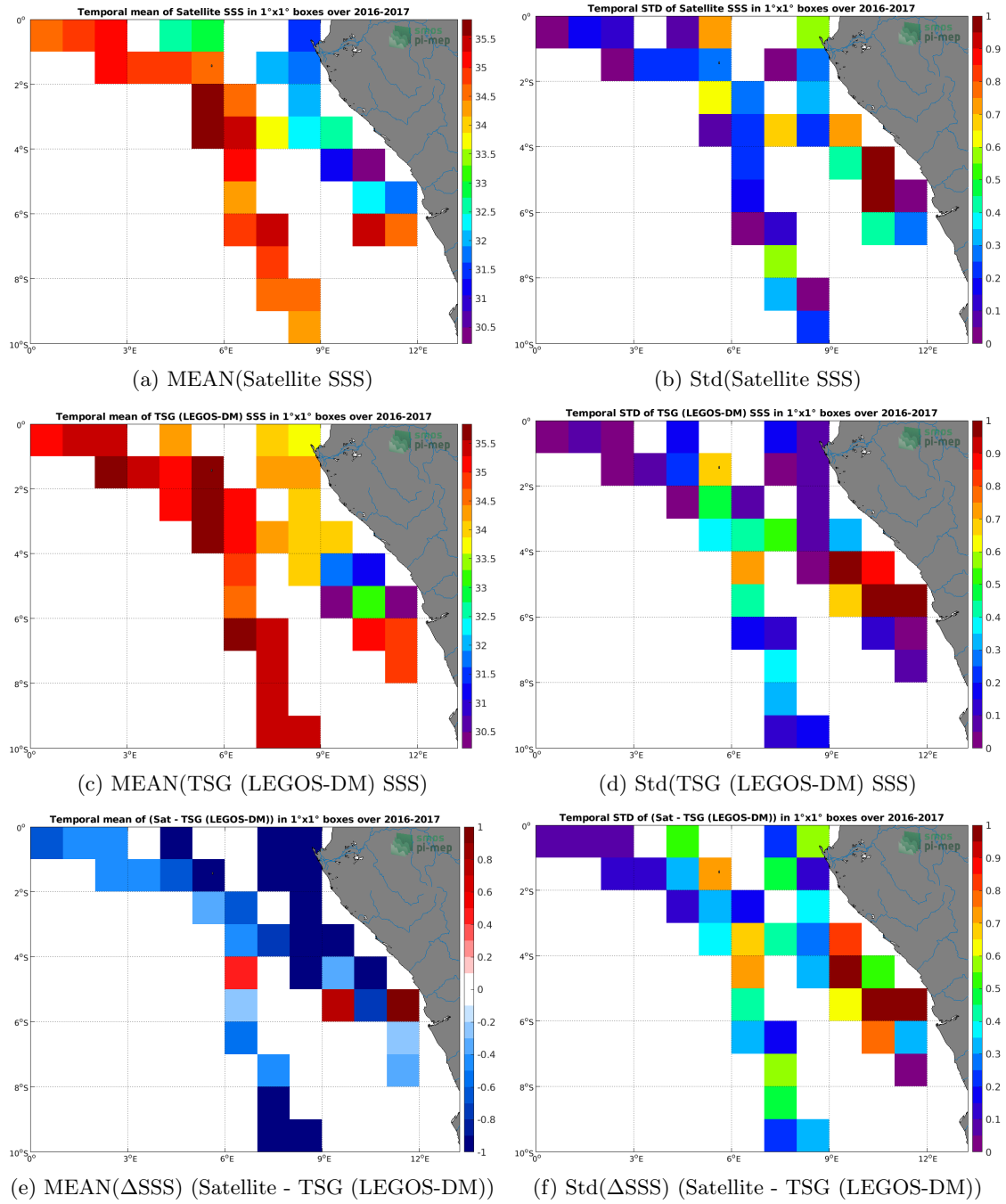
Figure 6: Temporal mean (left) and Std (right) of SSS from SMOS SSS L3 v2 - Monthly - 0.25 Deg (CATDS-CECOS-IFREMER) (top), TSG (LEGOS-DM) (middle), and of \Delta SSS (Satellite - TSG (LEGOS-DM)). Only match-up pairs are used to generate these maps.
