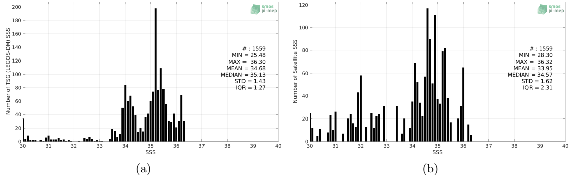
Figure 2: Histograms of SSS from TSG (LEGOS-DM) (a) and SMOS SSS L3 v2 - Monthly - 0.25 Deg (CATDS-CECOS-IFREMER) (b) considering all match-up pairs per bins of 0.1 over the Congo river plume Pi-MEP region and for the full satellite product period.
