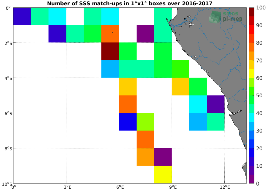
Figure 4: Number of SSS match-ups between TSG (LEGOS-DM) SSS and the SMOS SSS L3 v2 - Monthly - 0.25 Deg (CATDS-CECOS-IFREMER) SSS product for the Congo river plume Pi-MEP region over 1^\circ \times 1^\circ boxes and for the full satellite product period.
