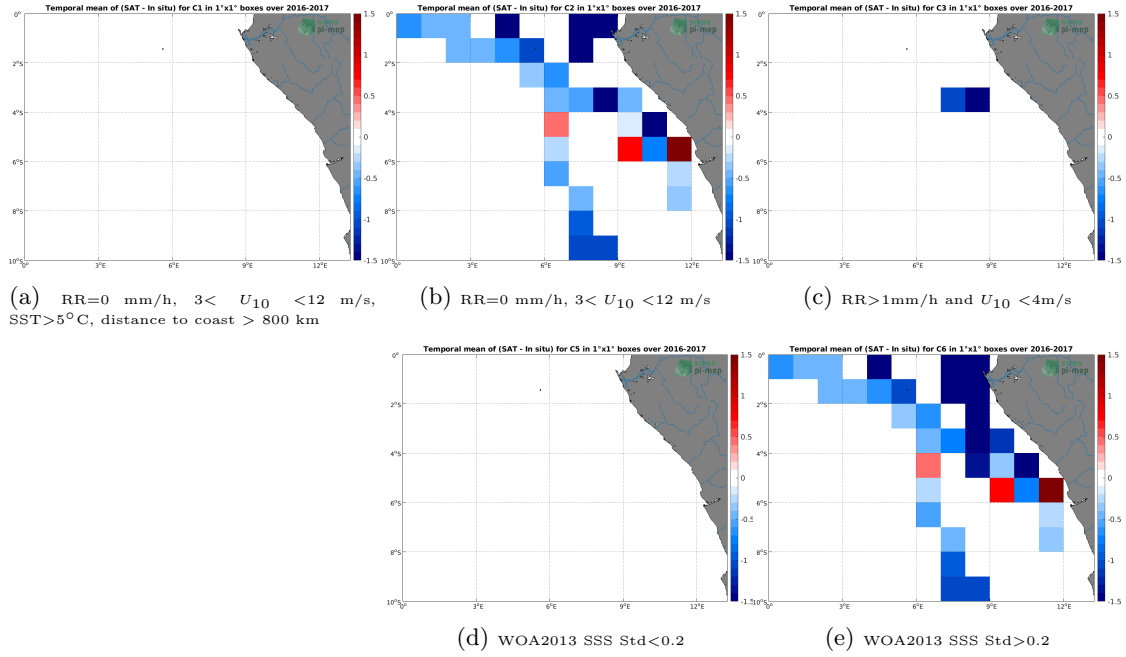
Figure 12: Temporal mean gridded over spatial boxes of size 1^{\circ}\times 1^{\circ} of \Delta\text{SSS} (SMOS SSS L3 v2 - Monthly - 0.25 Deg (CATDS-CECOS-IFREMER) - TSG (LEGOS-DM)) for 5 different subdatasets corresponding to:RR=0 mm/h, 3 < U_{10} < 12 m/s, SST >5^{\circ}\text{C} , distance to coast > 800 km (a), RR=0 mm/h, 3 < U_{10} < 12 m/s (b), RR >1 mm/h and U_{10} < 4 m/s (c), WOA2013 SSS Std <0.2 (d), WOA2013 SSS Std >0.2 (e).
