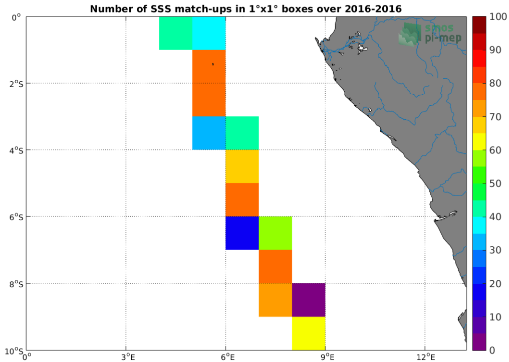
Figure 4: Number of SSS match-ups between TSG-LEGOS-DM SSS and the SMOS-L3-CATDS-IFREMER-CECOS-V2-MONTHLY-0.25DEG SSS product for the Congo river plume Pi-MEP region over 1^\circ \times 1^\circ boxes and for the full satellite product period.
