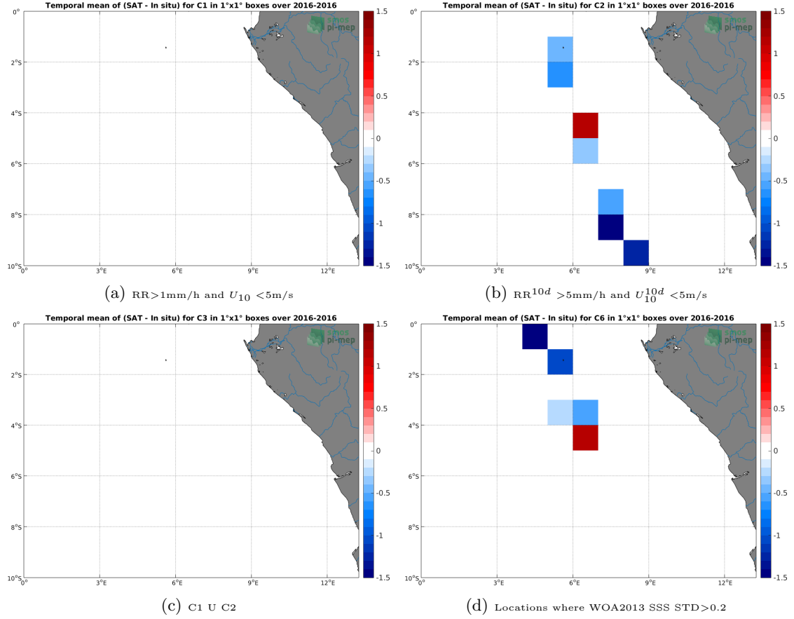
Figure 12: Temporal mean gridded over spatial boxes of size 1^\circ \times 1^\circ of \Delta SSS (SMOS-L3-CATDS-IFREMER-CECOS-V2-MONTHLY-0.25DEG - TSG-LEGOS-DM) for 4 different subdatasets corresponding to: RR > 1\text{mm/h} and U_{10} < 5\text{m/s} (a), RR^{10d} > 5\text{mm/h} and U_{10}^{10d} < 5\text{m/s} (b), C1 \cup C2 (c), Locations where WOA2013 SSS STD > 0.2 (d).
