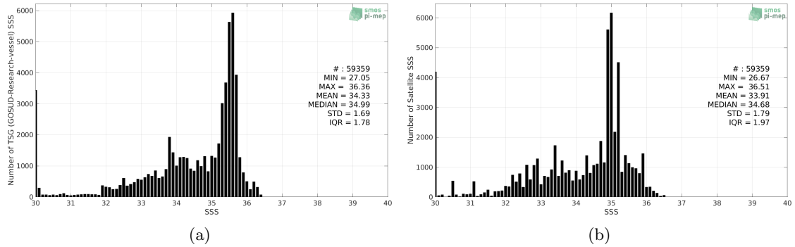
Figure 2: Histograms of SSS from TSG (GOSUD-Research-vessel) (a) and SMOS SSS L3 v2 - Monthly - 0.25 Deg (CATDS-CECOS-IFREMER) (b) considering all match-up pairs per bins of 0.1 over the Congo river plume Pi-MEP region and for the full satellite product period.
