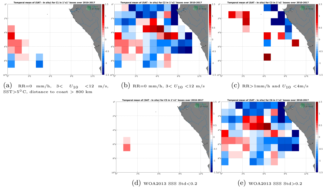
Figure 12: Temporal mean gridded over spatial boxes of size 1^\circ \times 1^\circ of \Delta SSS (SMOS SSS L3 v2 - Monthly - 0.25 Deg (CATDS-CECOS-IFREMER) - TSG (GOSUD-Research-vessel)) for 5 different subdatasets corresponding to: RR=0 mm/h, 3 < U_{10} < 12 m/s, SST > 5^\circ\text{C} , distance to coast > 800 km (a), RR=0 mm/h, 3 < U_{10} < 12 m/s (b), RR > 1 mm/h and U_{10} < 4 m/s (c), WOA2013 SSS Std < 0.2 (d), WOA2013 SSS Std > 0.2 (e).
