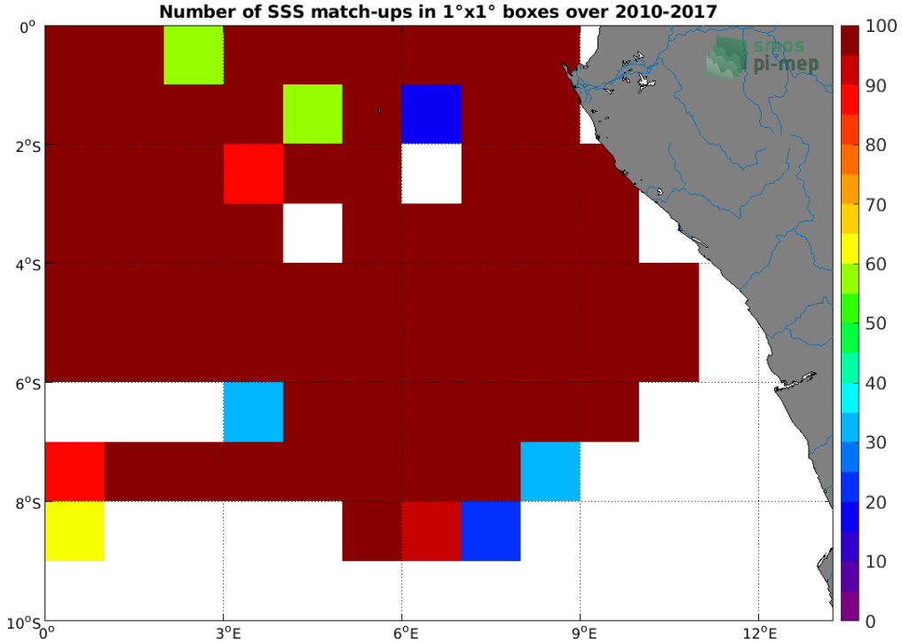
Figure 4: Number of SSS match-ups between TSG (GOSUD-Research-vessel) SSS and the SMOS SSS L3 v2 - Monthly - 0.25 Deg (CATDS-CECOS-IFREMER) SSS product for the Congo river plume Pi-MEP region over 1^\circ \times 1^\circ boxes and for the full satellite product period.
