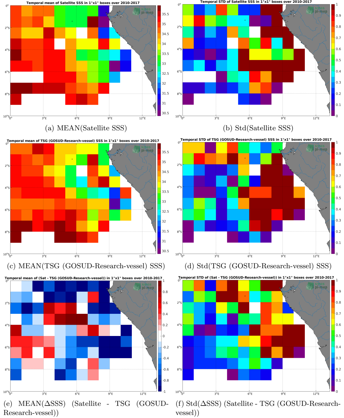
Figure 6: Temporal mean (left) and Std (right) of SSS from SMOS SSS L3 v2 - Monthly - 0.25 Deg (CATDS-CECOS-IFREMER) (top), TSG (GOSUD-Research-vessel) (middle), and of \Delta SSS (Satellite - TSG (GOSUD-Research-vessel)). Only match-up pairs are used to generate these maps.
