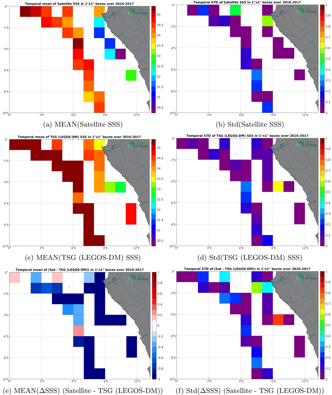
Figure 6: Temporal mean (left) and Std (right) of SSS from SMOS SSS L3 v2 - Daily - 0.5 Deg (CATDS-CECOS-IFREMER) (top), TSG (LEGOS-DM) (middle), and of \Delta SSS (Satellite - TSG (LEGOS-DM)). Only match-up pairs are used to generate these maps.
