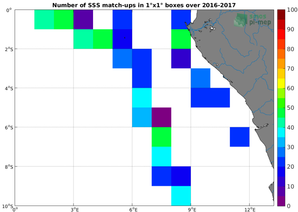
Figure 4: Number of SSS match-ups between TSG (LEGOS-DM) SSS and the SMOS SSS L3 v2 - Daily - 0.5 Deg (CATDS-CECOS-IFREMER) SSS product for the Congo river plume Pi-MEP region over 1°x1° boxes and for the full satellite product period.
