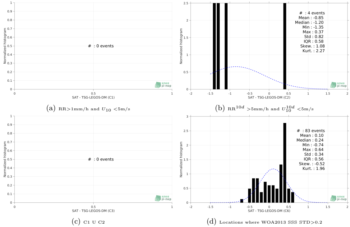
Figure 13: Normalized histogram of \Delta\text{SSS} (SMOS-L3-CATDS-CECOS-IFREMER-V2-1DAY-0.5DEG - TSG-LEGOS-DM) for 6 different subdatasets corresponding to: RR > 1\text{mm/h} and U_{10} < 5\text{m/s} (a), RR^{10d} > 5\text{mm/h} and U_{10}^{10d} < 5\text{m/s} (b), C1 U C2 (c), Locations where WOA2013 SSS STD > 0.2 (d).
