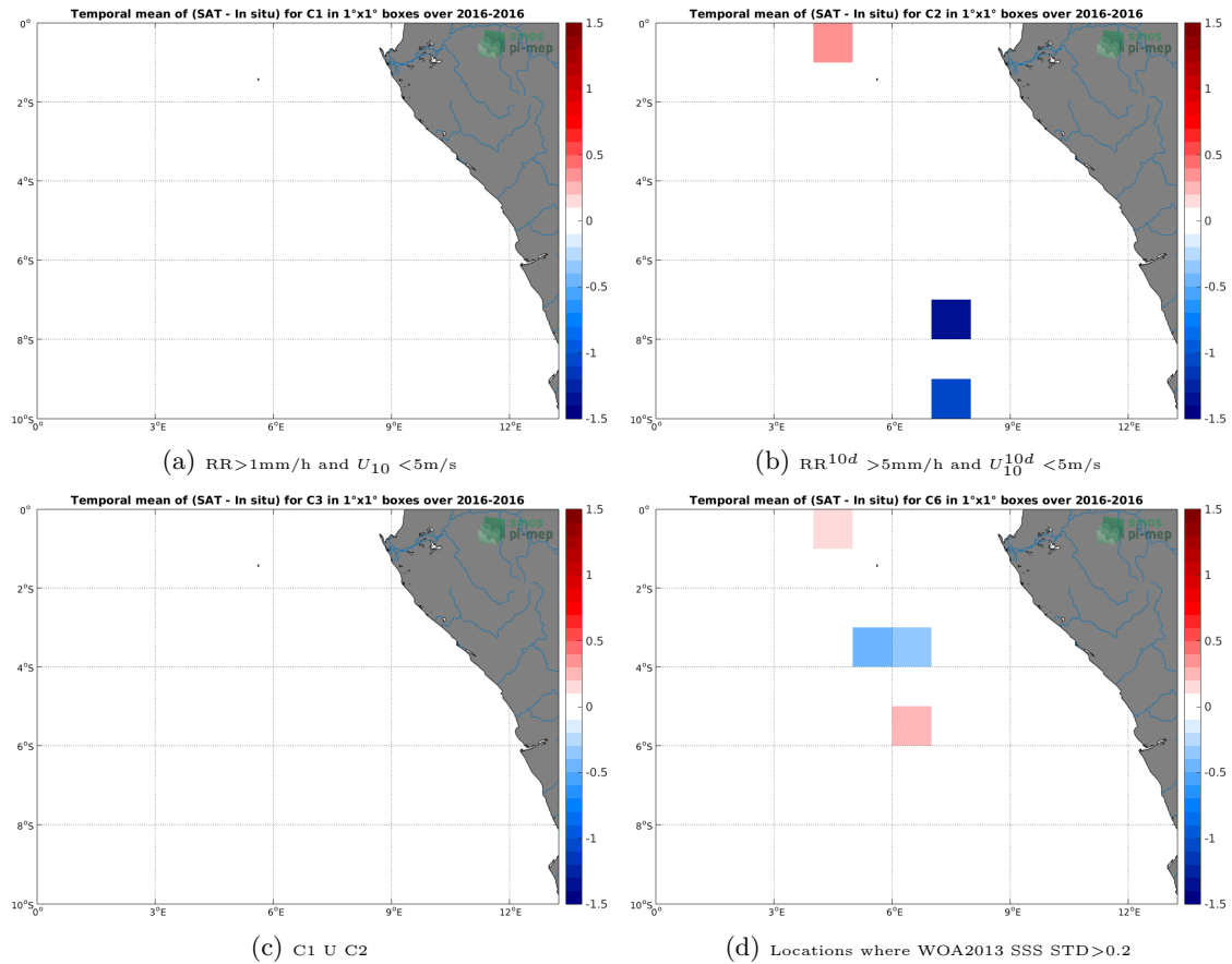
Figure 12: Temporal mean gridded over spatial boxes of size 1^\circ \times 1^\circ of \Delta SSS (SMOS-L3-CATDS-CECOS-IFREMER-V2-1DAY-0.5DEG - TSG-LEGOS-DM) for 4 different subdatasets corresponding to: RR > 1\text{mm/h} and U_{10} < 5\text{m/s} (a), RR^{10d} > 5\text{mm/h} and U_{10}^{10d} < 5\text{m/s} (b), C1 \cup C2 (c), Locations where WOA2013 SSS STD > 0.2 (d).
