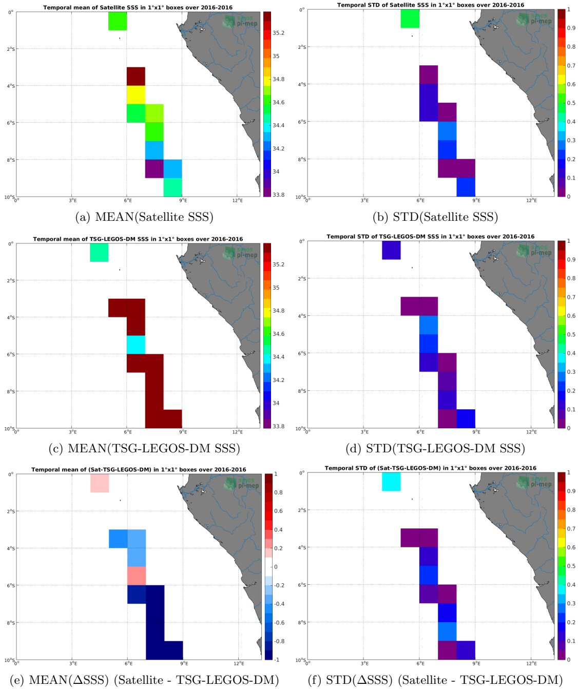
Figure 6: Temporal mean (left) and STD (right) of SSS from SMOS-L3-CATDS-CECOS-IFREMER-V2-1DAY-0.5DEG (top), TSG-LEGOS-DM (middle), and of \Delta SSS (Satellite - TSG-LEGOS-DM). Only match-up pairs are used to generate these maps.
