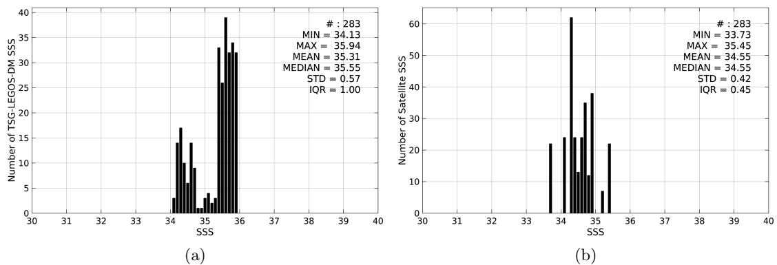
Figure 2: Histograms of SSS from TSG-LEGOS-DM (a) and SMOS-L3-CATDS-CECOS-IFREMER-V2-1DAY-0.5DEG (b) considering all match-up pairs per bins of 0.1 over the Congo river plume Pi-MEP region and for the full satellite product period.
