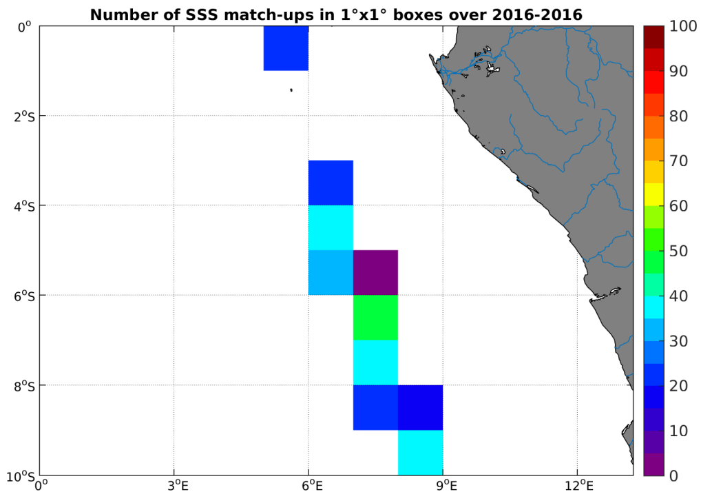
Figure 4: Number of SSS match-ups between TSG-LEGOS-DM SSS and the SMOS-L3-CATDS-CECOS-IFREMER-V2-1DAY-0.5DEG SSS product for the Congo river plume Pi-MEP region over 1^\circ \times 1^\circ boxes and for the full satellite product period.
