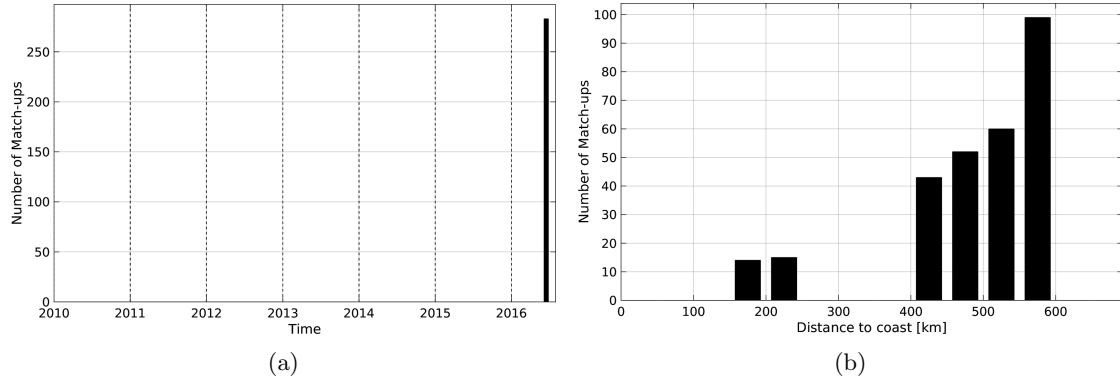
Figure 1: Number of match-ups between TSG-LEGOS-DM and SMOS-L3-CATDS-CECOS-IFREMER-V2-1DAY-0.5DEG SSS as a function of time (a) and as function of the distance to coast (b) over the Congo river plume Pi-MEP region and for the full satellite product period.
