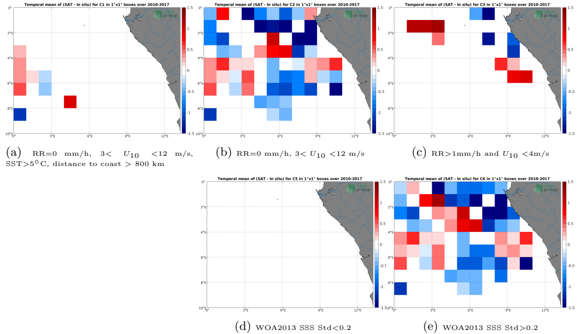
Figure 12: Temporal mean gridded over spatial boxes of size 1^{\circ}\times 1^{\circ} of \Delta SSS (SMOS SSS L3 v2 - Daily - 0.5 Deg (CATDS-CECOS-IFREMER) - TSG (GOSUD-Research-vessel)) for 5 different subdatasets corresponding to:RR=0 mm/h, 3 < U_{10} < 12 m/s, SST >5^{\circ}\text{C} , distance to coast > 800 km (a), RR=0 mm/h, 3 < U_{10} < 12 m/s (b), RR >1 mm/h and U_{10} < 4 m/s (c), WOA2013 SSS Std <0.2 (d), WOA2013 SSS Std >0.2 (e).
