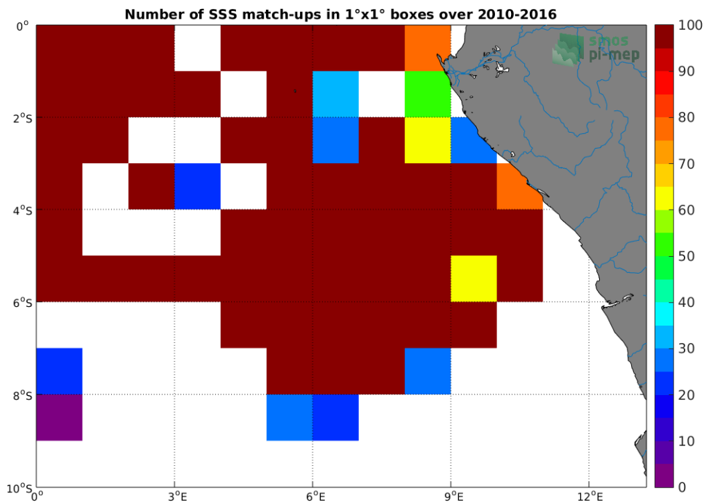
Figure 4: Number of SSS match-ups between TSG-GOSUD-Research-vessel SSS and the SMOS-L3-CATDS-CECOS-IFREMER-V2-1DAY-0.5DEG SSS product for the Congo river plume Pi-MEP region over 1^{\circ} \times 1^{\circ} boxes and for the full satellite product period.
