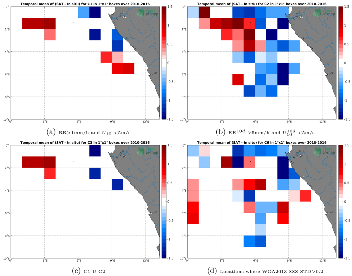
Figure 12: Temporal mean gridded over spatial boxes of size 1^\circ \times 1^\circ of \Delta SSS (SMOS-L3-CATDS-CECOS-IFREMER-V2-1DAY-0.5DEG - TSG-GOSUD-Research-vessel) for 4 different subdatasets corresponding to: RR > 1mm/h and U_{10} < 5m/s (a), RR^{10d} > 5mm/h and U_{10}^{10d} < 5m/s (b), C1 U C2 (c), Locations where WOA2013 SSS STD > 0.2 (d).
