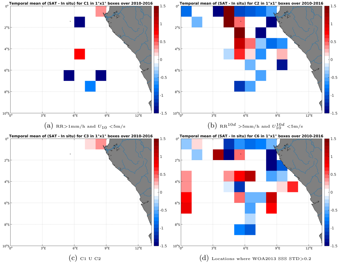
Figure 12: Temporal mean gridded over spatial boxes of size 1°x1° of \Delta SSS (SMOS-L3-CATDS-CECOS-IFREMER-V2-1DAY-0.5DEG - TSG-GOSUD-Research-vessel) for 4 different subdatasets corresponding to:RR>1mm/h and U_{10} < 5m/s (a), RR^{10d} > 5mm/h and U_{10}^{10d} < 5m/s (b), C1 U C2 (c),Locations where WOA2013 SSS STD>0.2 (d).
