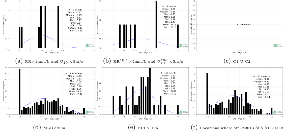
Figure 13: Normalized histogram of \Delta SSS (SMOS-L3-CATDS-CECOS-IFREMER-V2-1DAY-0.5DEG - Argo) for 6 different subdatasets corresponding to: RR > 1mm/h and U_{10} < 5 m/s (a), RR^{10d} > 5 mm/h and U_{10}^{10d} < 5 m/s (b), C1 U C2 (c), MLD < 20m (d), BLT > 10m (e), Locations where WOA2013 SSS STD > 0.2 (f).
