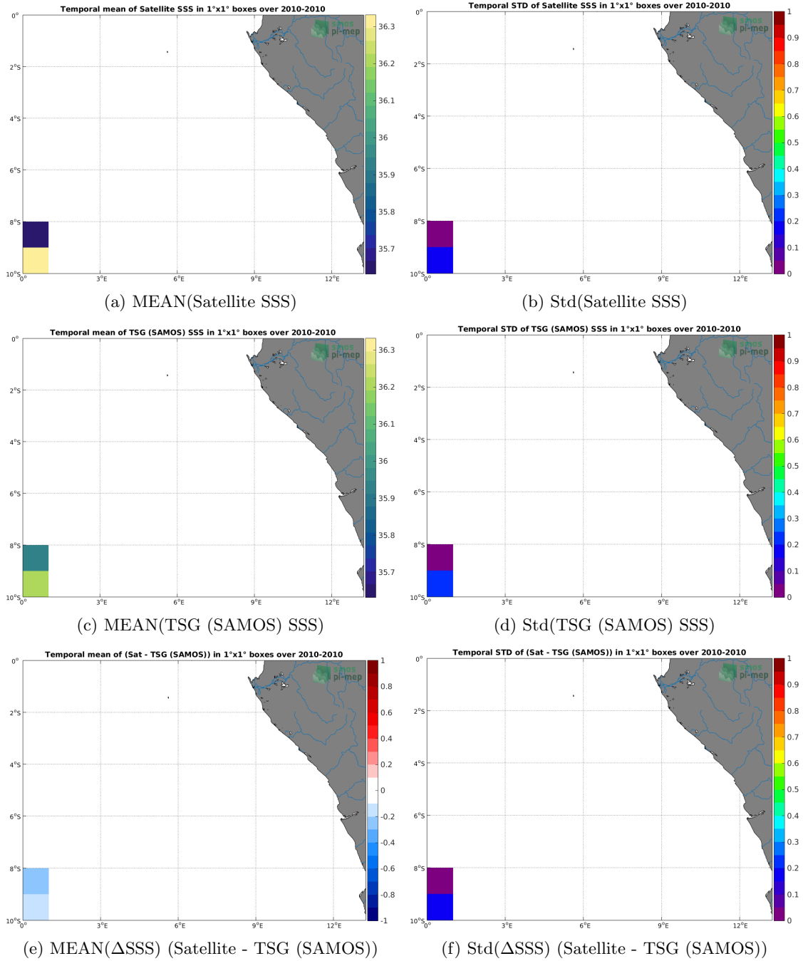
Figure 6: Temporal mean (left) and Std (right) of SSS from SMOS SSS L3 v335 - Monthly - 25 km (CATDS-CPDC) (top), TSG (SAMOS) (middle), and of \Delta SSS (Satellite - TSG (SAMOS)). Only match-up pairs are used to generate these maps.
