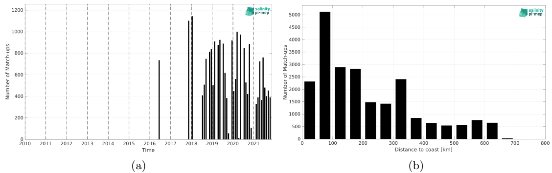
Figure 2: Number of match-ups between TSG (LEGOS-DM) and SMOS SSS L3 v335 - Monthly - 25 km (CATDS-CPDC) SSS as a function of time (a) and as function of the distance to coast (b) over the Congo river plume Pi-MEP region and for the full satellite product period.
