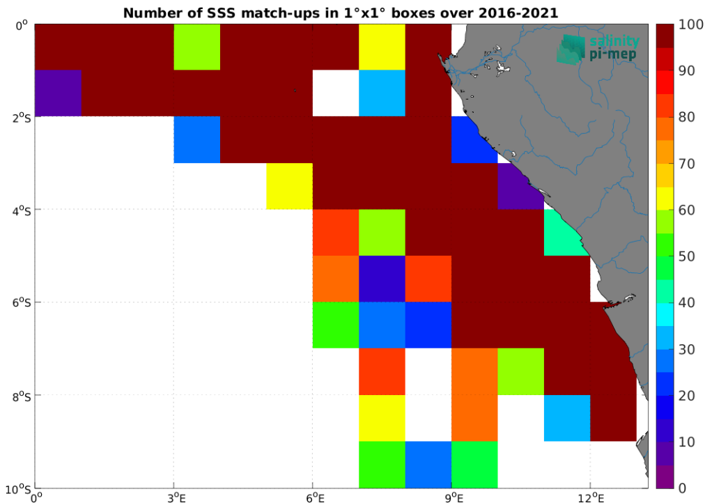
Figure 5: Number of SSS match-ups between TSG (LEGOS-DM) SSS and the SMOS SSS L3 v335 - Monthly - 25 km (CATDS-CPDC) SSS product for the Congo river plume Pi-MEP region over 1^\circ \times 1^\circ boxes and for the full satellite product period.
