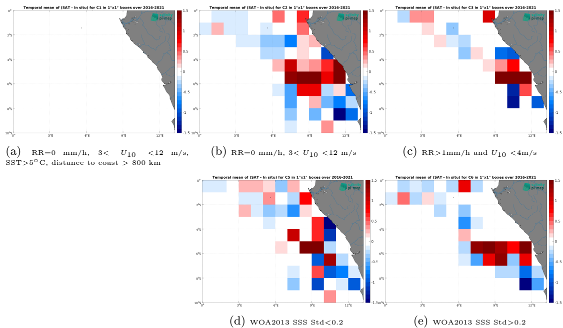
Figure 14: Temporal mean gridded over spatial boxes of size 1^\circ \times 1^\circ of \Delta SSS (SMOS SSS L3 v335 - Monthly - 25 km (CATDS-CPDC) - TSG (LEGOS-DM)) for 5 different subdatasets corresponding to:RR=0 mm/h, 3 < U_{10} < 12 m/s, SST > 5^\circ\text{C} , distance to coast > 800 km (a), RR=0 mm/h, 3 < U_{10} < 12 m/s (b), RR > 1 mm/h and U_{10} < 4 m/s (c), WOA2013 SSS Std < 0.2 (d), WOA2013 SSS Std > 0.2 (e).
