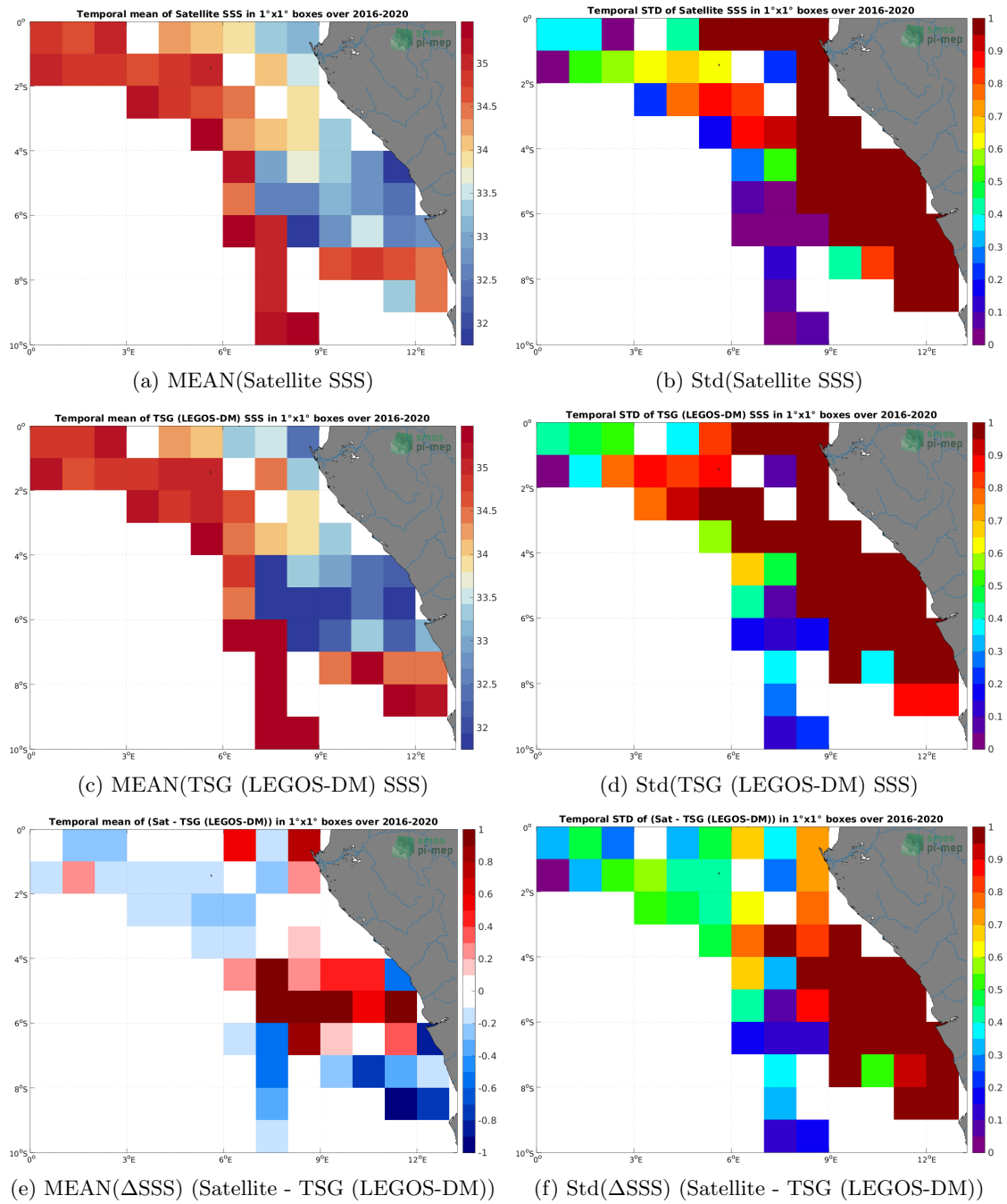
Figure 6: Temporal mean (left) and Std (right) of SSS from SMOS SSS L3 v335 - Monthly - 25 km (CATDS-CPDC) (top), TSG (LEGOS-DM) (middle), and of \Delta SSS (Satellite - TSG (LEGOS-DM)). Only match-up pairs are used to generate these maps.
