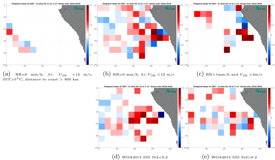
Figure 12: Temporal mean gridded over spatial boxes of size 1^\circ \times 1^\circ of \Delta\text{SSS} (SMOS SSS L3 v335 - Monthly - 25 km (CATDS-CPDC) - TSG (GOSUD-Research-vessel)) for 5 different subdatasets corresponding to:RR=0 mm/h, 3 < U_{10} < 12 m/s, SST > 5^\circ\text{C} , distance to coast > 800 km (a), RR=0 mm/h, 3 < U_{10} < 12 m/s (b), RR > 1 mm/h and U_{10} < 4 m/s (c), WOA2013 SSS Std < 0.2 (d), WOA2013 SSS Std > 0.2 (e).
