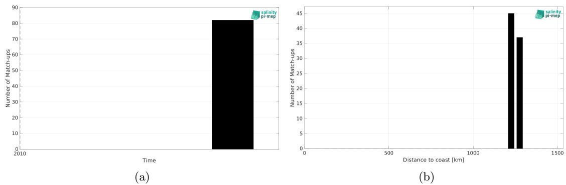
Figure 1: Number of match-ups between TSG (SAMOS) and SMOS SSS L3 v335 - 10 Days - 25 km (CATDS-CPDC) SSS as a function of time (a) and as function of the distance to coast (b) over the Congo river plume Pi-MEP region and for the full satellite product period.
