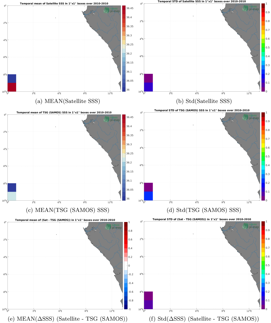
Figure 6: Temporal mean (left) and Std (right) of SSS from SMOS SSS L3 v335 - 10 Days - 25 km (CATDS-CPDC) (top), TSG (SAMOS) (middle), and of \Delta SSS (Satellite - TSG (SAMOS)). Only match-up pairs are used to generate these maps.
