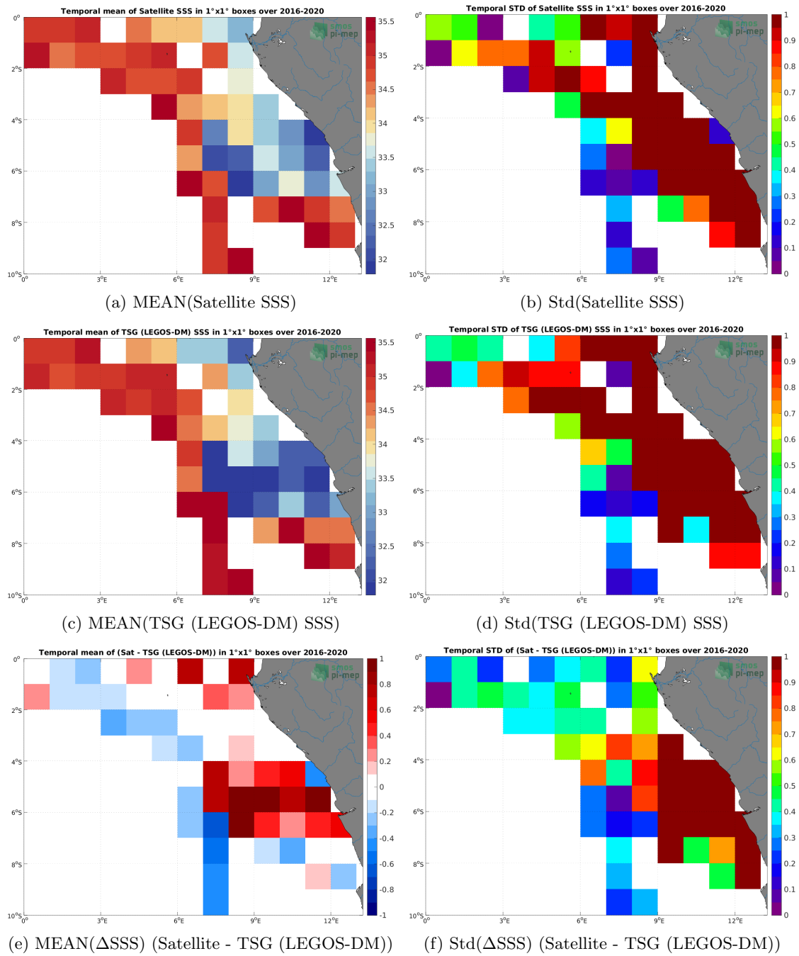
Figure 6: Temporal mean (left) and Std (right) of SSS from SMOS SSS L3 v335 - 10 Days - 25 km (CATDS-CPDC) (top), TSG (LEGOS-DM) (middle), and of \Delta SSS (Satellite - TSG (LEGOS-DM)). Only match-up pairs are used to generate these maps.
