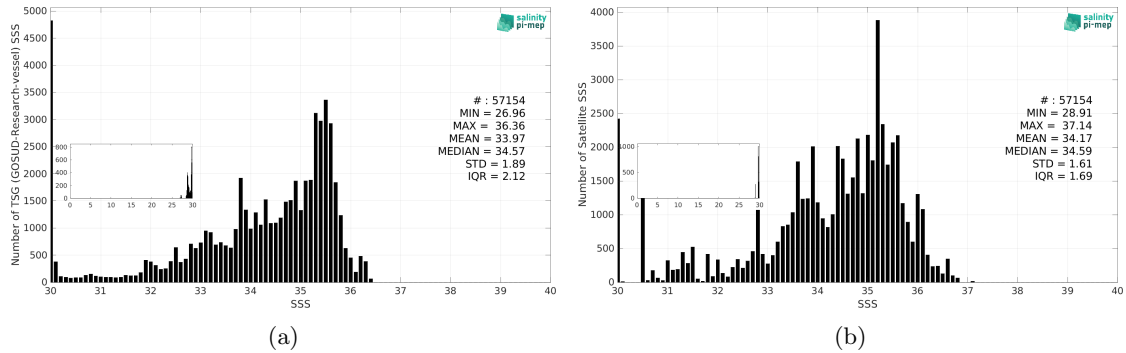
Figure 3: Histograms of SSS from TSG (GOSUD-Research-vessel) (a) and SMOS SSS L3 v335 - 10 Days - 25 km (CATDS-CPDC) (b) considering all match-up pairs per bins of 0.1 over the Congo river plume Pi-MEP region and for the full satellite product period.
