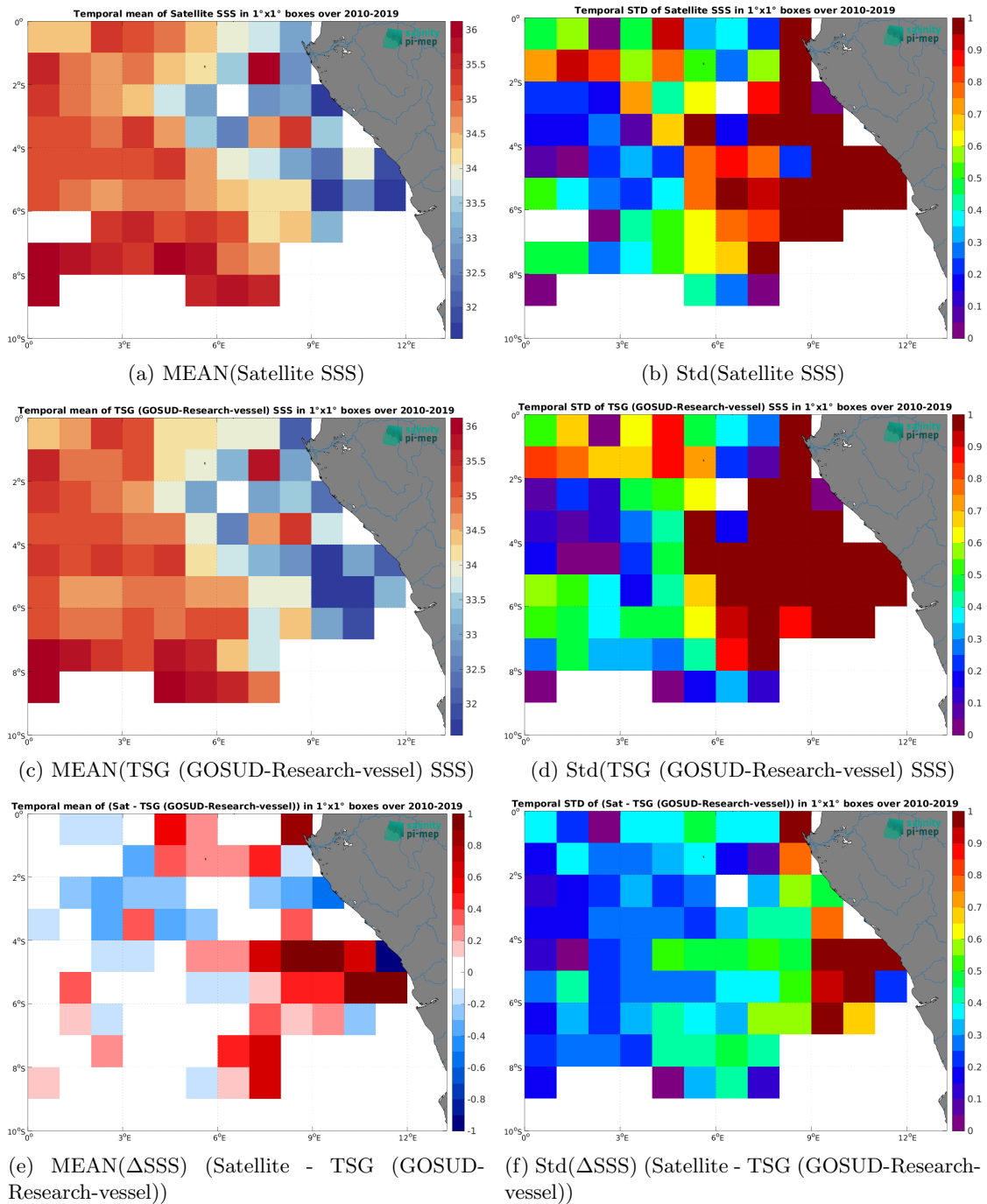
Figure 7: Temporal mean (left) and Std (right) of SSS from SMOS SSS L3 v335 - 10 Days - 25 km (CATDS-CPDC) (top), TSG (GOSUD-Research-vessel) (middle), and of \Delta SSS (Satellite - TSG (GOSUD-Research-vessel)). Only match-up pairs are used to generate these maps.
