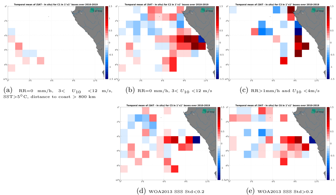
Figure 14: Temporal mean gridded over spatial boxes of size 1^\circ \times 1^\circ of \Delta SSS (SMOS SSS L3 v335 - 10 Days - 25 km (CATDS-CPDC) - TSG (GOSUD-Research-vessel)) for 5 different subdatasets corresponding to:RR=0 mm/h, 3 < U_{10} < 12 m/s, SST>5°C, distance to coast > 800 km (a), RR=0 mm/h, 3 < U_{10} < 12 m/s (b), RR>1mm/h and U_{10} < 4 m/s (c), WOA2013 SSS Std<0.2 (d), WOA2013 SSS Std>0.2 (e).
