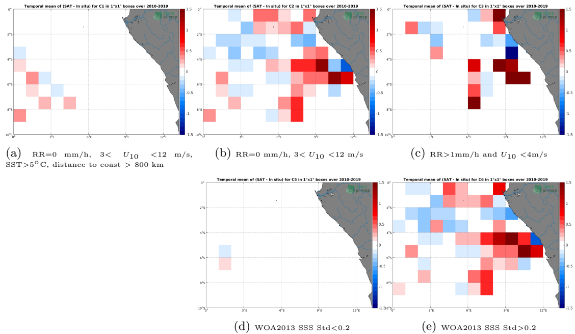
Figure 12: Temporal mean gridded over spatial boxes of size 1^{\circ}\times 1^{\circ} of \Delta SSS (SMOS SSS L3 v335 - 10 Days - 25 km (CATDS-CPDC) - TSG (GOSUD-Research-vessel)) for 5 different subdatasets corresponding to:RR=0 mm/h, 3 < U_{10} < 12 m/s, SST >5^{\circ}\text{C} , distance to coast > 800 km (a), RR=0 mm/h, 3 < U_{10} < 12 m/s (b), RR >1 mm/h and U_{10} < 4 m/s (c), WOA2013 SSS Std <0.2 (d), WOA2013 SSS Std >0.2 (e).
