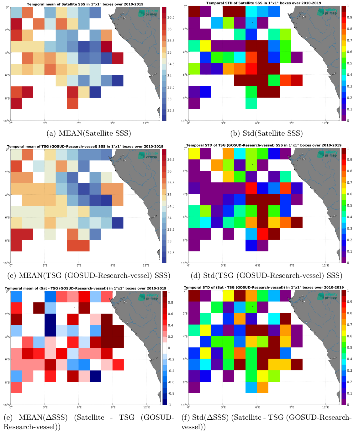
Figure 7: Temporal mean (left) and Std (right) of SSS from SMOS SSS L2Q v333 - 0.25 Deg (CATDS-CPDC) (top), TSG (GOSUD-Research-vessel) (middle), and of \Delta SSS (Satellite - TSG (GOSUD-Research-vessel)). Only match-up pairs are used to generate these maps.
