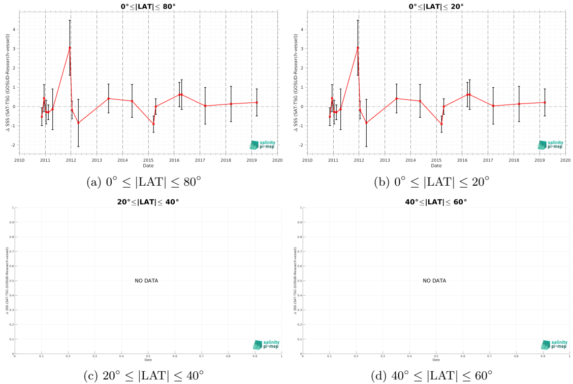
Figure 11: Monthly median (red curves) of \Delta SSS (Satellite - in situ ) between SMOS SSS L2Q v333 - 0.25 Deg (CATDS-CPDC) and TSG (GOSUD-Research-vessel) SSS as function of time for all the collected Pi-MEP match-up pairs estimated over the Congo river plume Pi-MEP region and for the full satellite product period are shown for different latitude bands: (a) 80^{\circ}\text{S}-80^{\circ}\text{N} , (b) 20^{\circ}\text{S}-20^{\circ}\text{N} , (c) 40^{\circ}\text{S}-20^{\circ}\text{S} and 20^{\circ}\text{N}-40^{\circ}\text{N} and (d) 60^{\circ}\text{S}-40^{\circ}\text{S} and 40^{\circ}\text{N}-60^{\circ}\text{N} .
