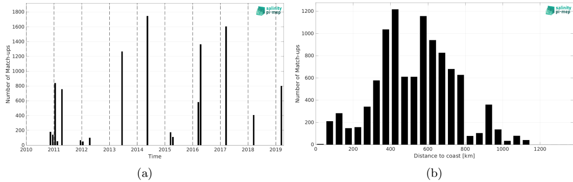
Figure 2: Number of match-ups between TSG (GOSUD-Research-vessel) and SMOS SSS L2Q v333 - 0.25 Deg (CATDS-CPDC) SSS as a function of time (a) and as function of the distance to coast (b) over the Congo river plume Pi-MEP region and for the full satellite product period.
