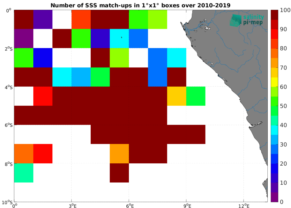
Figure 5: Number of SSS match-ups between TSG (GOSUD-Research-vessel) SSS and the SMOS SSS L2Q v333 - 0.25 Deg (CATDS-CPDC) SSS product for the Congo river plume Pi-MEP region over 1^\circ \times 1^\circ boxes and for the full satellite product period.
