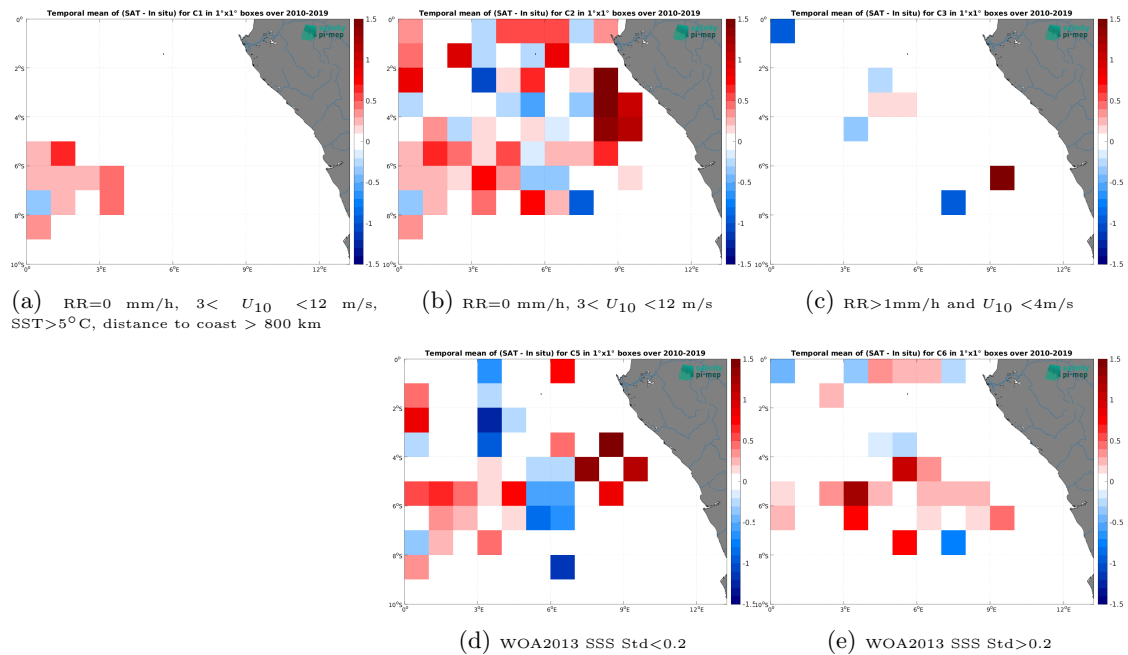
Figure 14: Temporal mean gridded over spatial boxes of size 1^\circ \times 1^\circ of \Delta SSS (SMOS SSS L2Q v333 - 0.25 Deg (CATDS-CPDC) - TSG (GOSUD-Research-vessel)) for 5 different subdatasets corresponding to:RR=0 mm/h, 3 < U_{10} < 12 m/s, SST>5°C, distance to coast > 800 km (a), RR=0 mm/h, 3 < U_{10} < 12 m/s (b), RR>1mm/h and U_{10} < 4 m/s (c), WOA2013 SSS Std<0.2 (d), WOA2013 SSS Std>0.2 (e).
