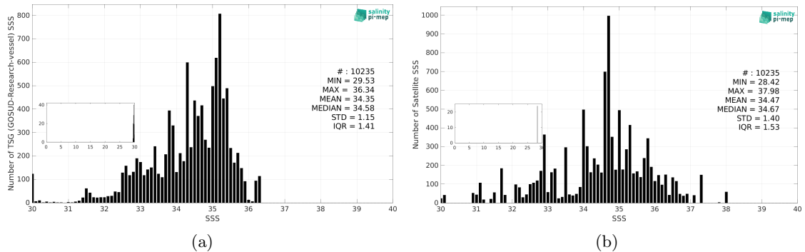
Figure 3: Histograms of SSS from TSG (GOSUD-Research-vessel) (a) and SMOS SSS L2Q v333 - 0.25 Deg (CATDS-CPDC) (b) considering all match-up pairs per bins of 0.1 over the Congo river plume Pi-MEP region and for the full satellite product period.
