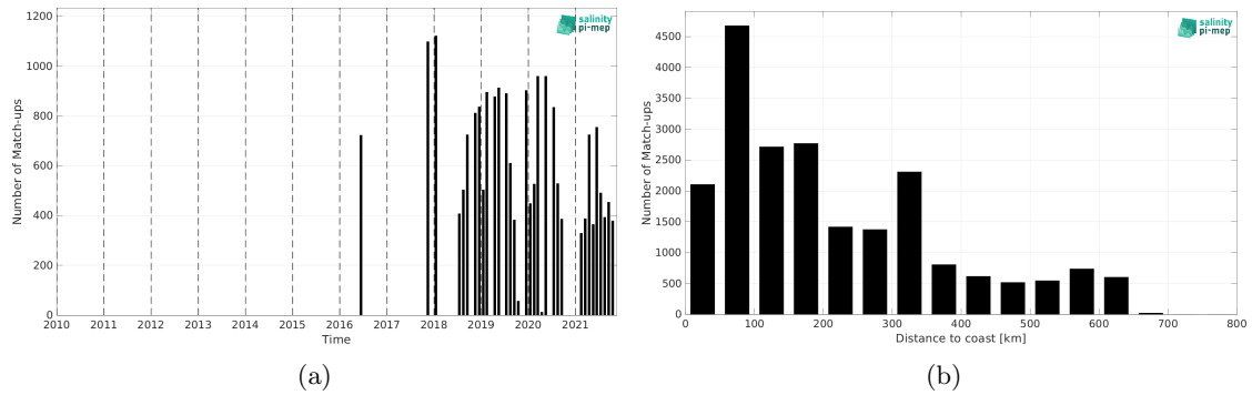
Figure 1: Number of match-ups between TSG (LEGOS-DM) and SMOS SSS L3 v332 - 9 Days (CATDS-CPDC) SSS as a function of time (a) and as function of the distance to coast (b) over the Congo river plume Pi-MEP region and for the full satellite product period.
