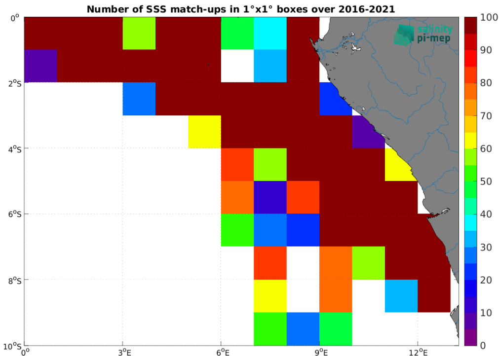
Figure 4: Number of SSS match-ups between TSG (LEGOS-DM) SSS and the SMOS SSS L3 v332 - 9 Days (CATDS-CPDC) SSS product for the Congo river plume Pi-MEP region over 1^\circ \times 1^\circ boxes and for the full satellite product period.
