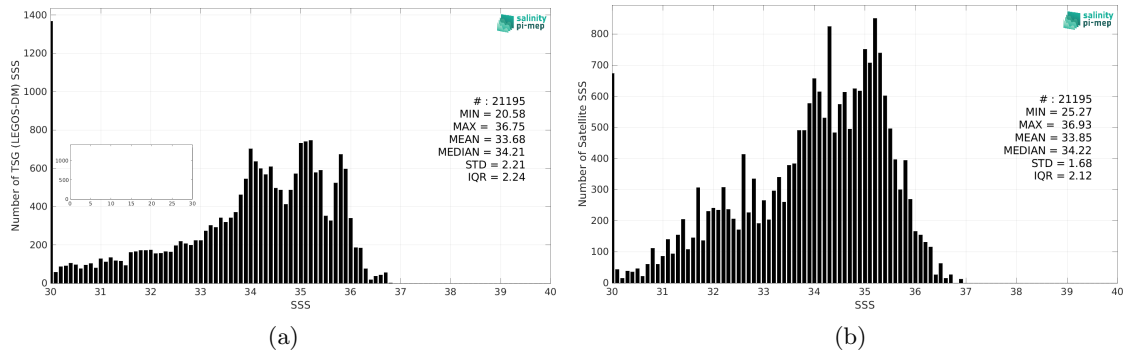
Figure 2: Histograms of SSS from TSG (LEGOS-DM) (a) and SMOS SSS L3 v332 - 9 Days (CATDS-CPDC) (b) considering all match-up pairs per bins of 0.1 over the Congo river plume Pi-MEP region and for the full satellite product period.
