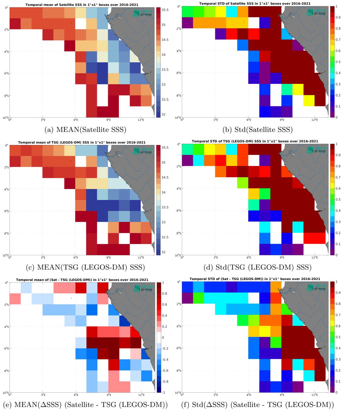
Figure 6: Temporal mean (left) and Std (right) of SSS from SMOS SSS L3 v332 - 9 Days (CATDS-CPDC) (top), TSG (LEGOS-DM) (middle), and of \Delta SSS (Satellite - TSG (LEGOS-DM)). Only match-up pairs are used to generate these maps.
