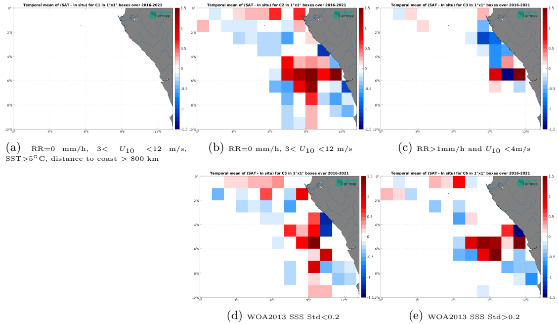
Figure 12: Temporal mean gridded over spatial boxes of size 1^\circ \times 1^\circ of \Delta SSS (SMOS SSS L3 v332 - 9 Days (CATDS-CPDC) - TSG (LEGOS-DM)) for 5 different subdatasets corresponding to:RR=0 mm/h, 3 < U_{10} < 12 m/s, SST > 5°C, distance to coast > 800 km (a), RR=0 mm/h, 3 < U_{10} < 12 m/s (b), RR > 1mm/h and U_{10} < 4 m/s (c), WOA2013 SSS Std < 0.2 (d), WOA2013 SSS Std > 0.2 (e).
