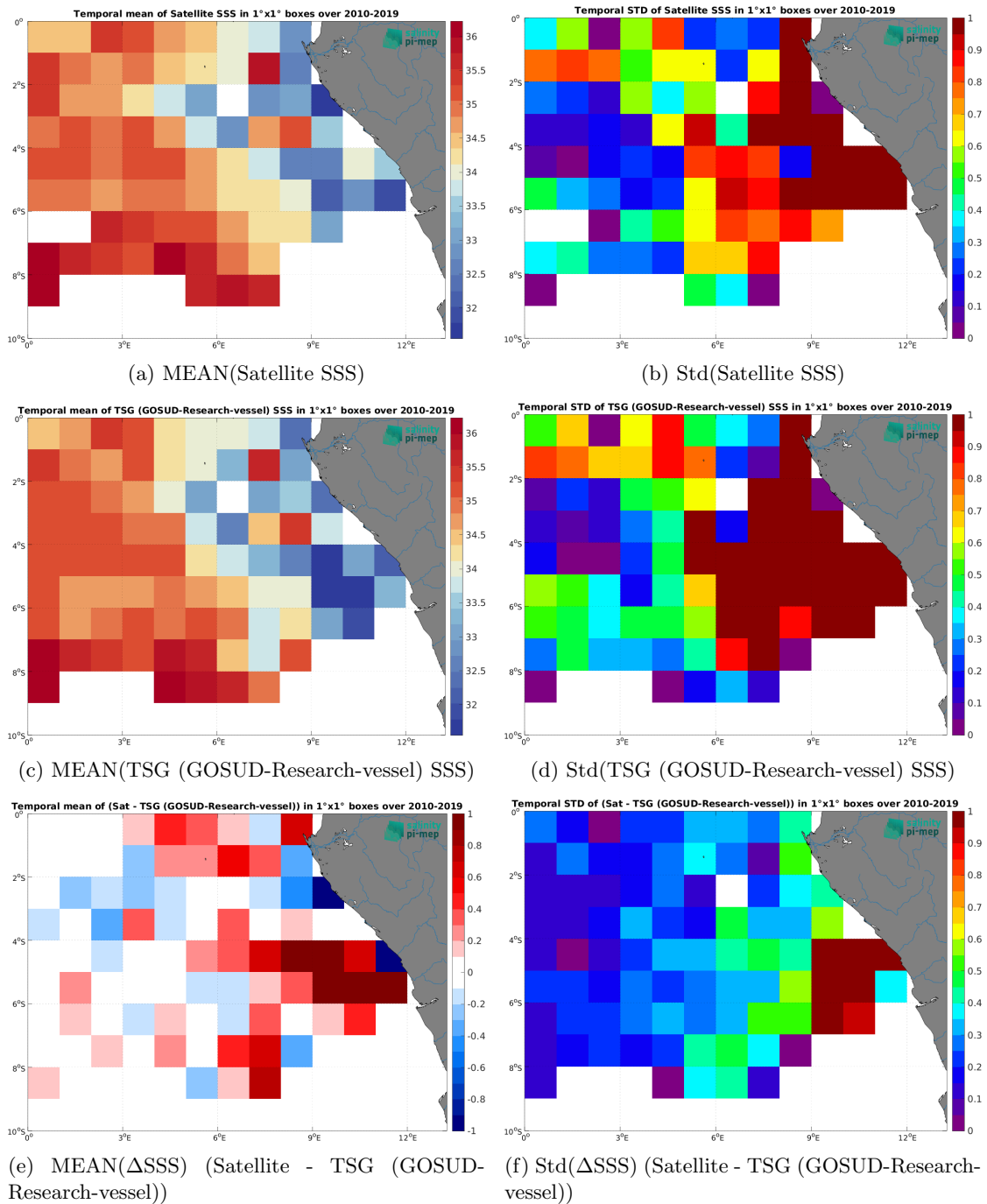
Figure 7: Temporal mean (left) and Std (right) of SSS from SMOS SSS L3 v332 - 9 Days (CATDS-CPDC) (top), TSG (GOSUD-Research-vessel) (middle), and of \Delta SSS (Satellite - TSG (GOSUD-Research-vessel)). Only match-up pairs are used to generate these maps.
