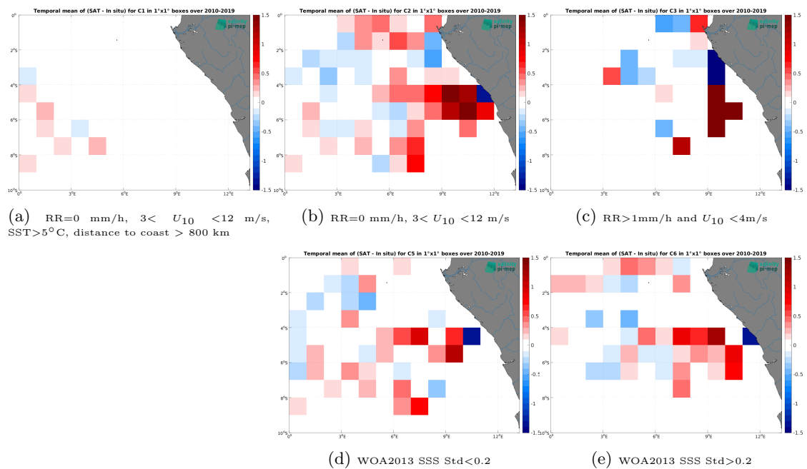
Figure 14: Temporal mean gridded over spatial boxes of size 1^\circ \times 1^\circ of \Delta SSS (SMOS SSS L3 v332 - 9 Days (CATDS-CPDC) - TSG (GOSUD-Research-vessel)) for 5 different subdatasets corresponding to:RR=0 mm/h, 3 < U_{10} < 12 m/s, SST>5°C, distance to coast > 800 km (a), RR=0 mm/h, 3 < U_{10} < 12 m/s (b), RR>1mm/h and U_{10} < 4 m/s (c), WOA2013 SSS Std<0.2 (d), WOA2013 SSS Std>0.2 (e).
