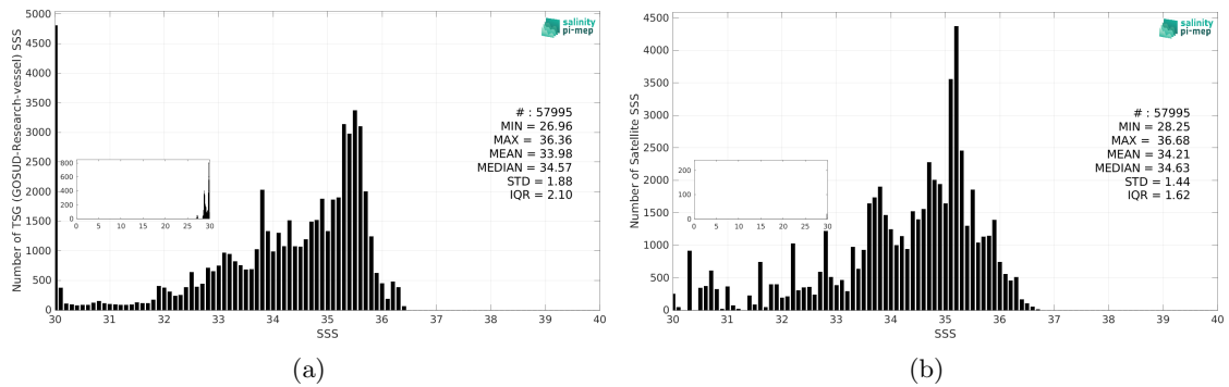
Figure 3: Histograms of SSS from TSG (GOSUD-Research-vessel) (a) and SMOS SSS L3 v332 - 9 Days (CATDS-CPDC) (b) considering all match-up pairs per bins of 0.1 over the Congo river plume Pi-MEP region and for the full satellite product period.
