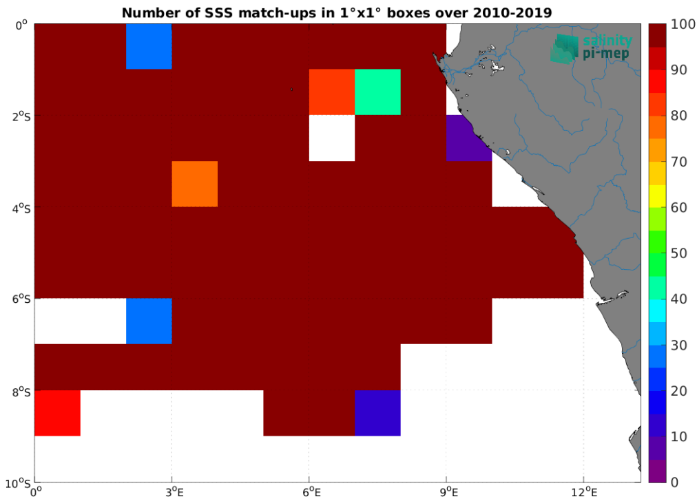
Figure 5: Number of SSS match-ups between TSG (GOSUD-Research-vessel) SSS and the SMOS SSS L3 v332 - 9 Days (CATDS-CPDC) SSS product for the Congo river plume Pi-MEP region over 1^\circ \times 1^\circ boxes and for the full satellite product period.
