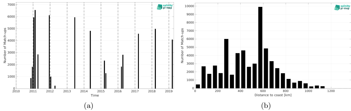
Figure 2: Number of match-ups between TSG (GOSUD-Research-vessel) and SMOS SSS L3 v332 - 9 Days (CATDS-CPDC) SSS as a function of time (a) and as function of the distance to coast (b) over the Congo river plume Pi-MEP region and for the full satellite product period.
