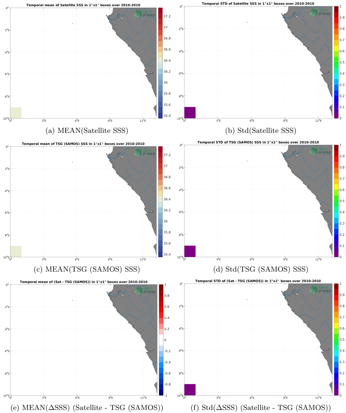
Figure 6: Temporal mean (left) and Std (right) of SSS from SMOS SSS L2Q v331 - 0.25 Deg (CATDS-CPDC) (top), TSG (SAMOS) (middle), and of \Delta SSS (Satellite - TSG (SAMOS)). Only match-up pairs are used to generate these maps.
