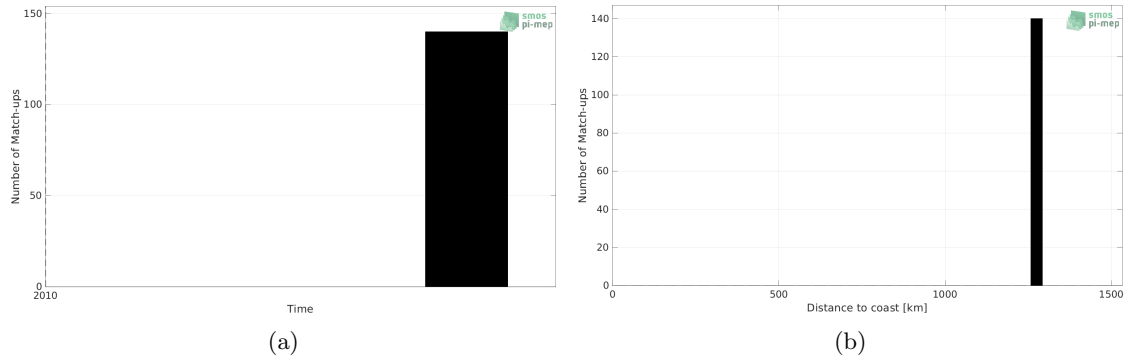
Figure 1: Number of match-ups between TSG (SAMOS) and SMOS SSS L2Q v331 - 0.25 Deg (CATDS-CPDC) SSS as a function of time (a) and as function of the distance to coast (b) over the Congo river plume Pi-MEP region and for the full satellite product period.
