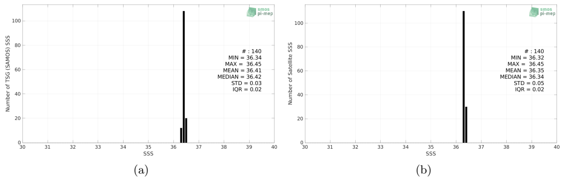
Figure 2: Histograms of SSS from TSG (SAMOS) (a) and SMOS SSS L2Q v331 - 0.25 Deg (CATDS-CPDC) (b) considering all match-up pairs per bins of 0.1 over the Congo river plume Pi-MEP region and for the full satellite product period.
