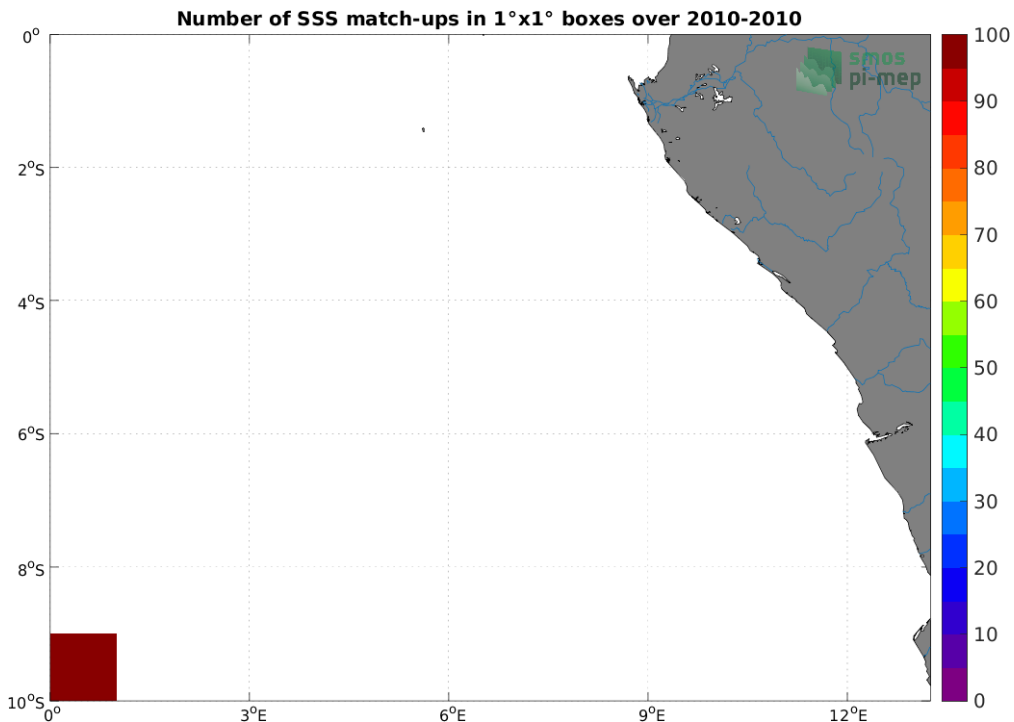
Figure 4: Number of SSS match-ups between TSG (SAMOS) SSS and the SMOS SSS L2Q v331 - 0.25 Deg (CATDS-CPDC) SSS product for the Congo river plume Pi-MEP region over 1^\circ \times 1^\circ boxes and for the full satellite product period.
