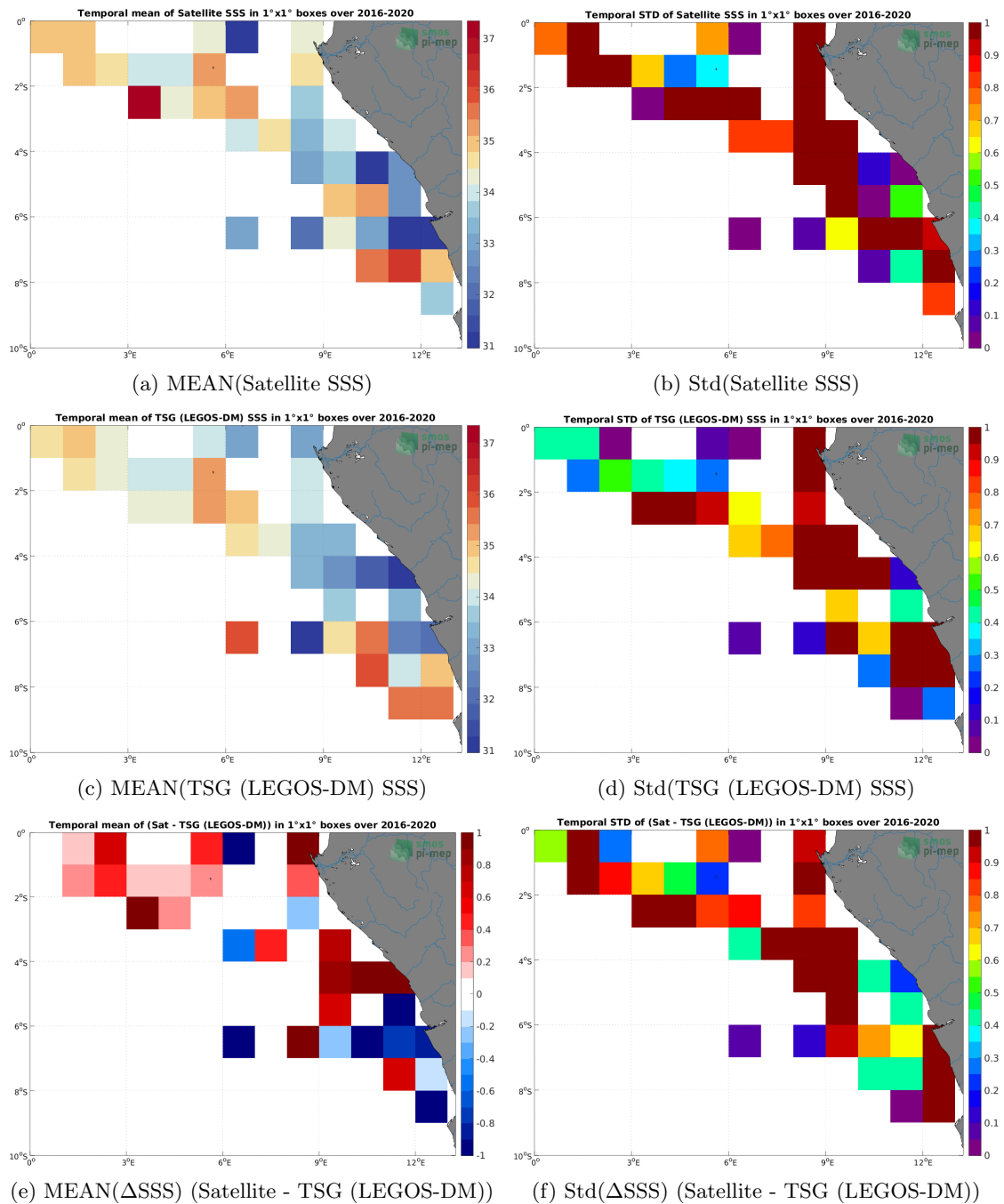
Figure 6: Temporal mean (left) and Std (right) of SSS from SMOS SSS L2Q v331 - 0.25 Deg (CATDS-CPDC) (top), TSG (LEGOS-DM) (middle), and of \Delta SSS (Satellite - TSG (LEGOS-DM)). Only match-up pairs are used to generate these maps.
