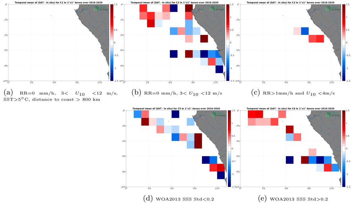
Figure 12: Temporal mean gridded over spatial boxes of size 1^{\circ}\times 1^{\circ} of \Delta\text{SSS} (SMOS SSS L2Q v331 - 0.25 Deg (CATDS-CPDC) - TSG (LEGOS-DM)) for 5 different subdatasets corresponding to:RR=0 mm/h, 3 < U_{10} < 12 m/s, SST >5^{\circ}\text{C} , distance to coast > 800 km (a), RR=0 mm/h, 3 < U_{10} < 12 m/s (b), RR >1 mm/h and U_{10} < 4 m/s (c), WOA2013 SSS Std <0.2 (d), WOA2013 SSS Std >0.2 (e).
