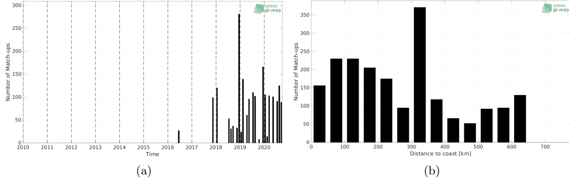
Figure 1: Number of match-ups between TSG (LEGOS-DM) and SMOS SSS L2Q v331 - 0.25 Deg (CATDS-CPDC) SSS as a function of time (a) and as function of the distance to coast (b) over the Congo river plume Pi-MEP region and for the full satellite product period.
