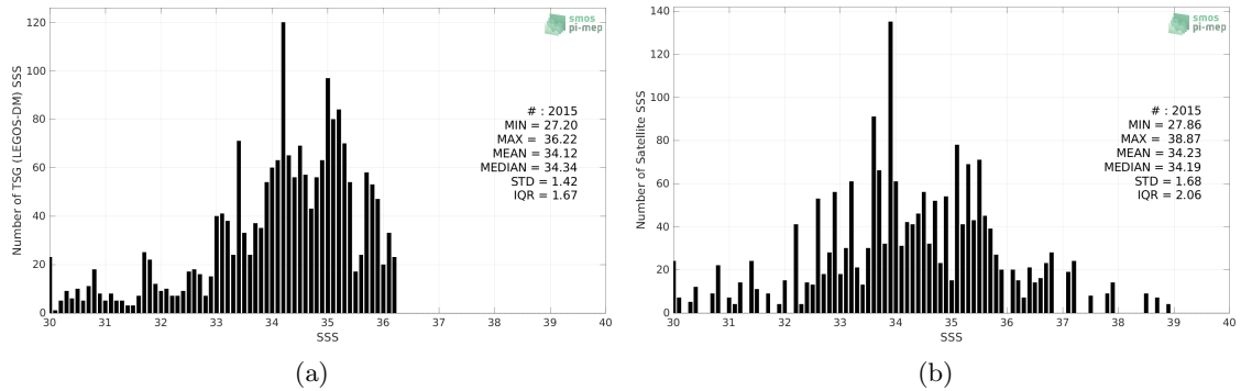
Figure 2: Histograms of SSS from TSG (LEGOS-DM) (a) and SMOS SSS L2Q v331 - 0.25 Deg (CATDS-CPDC) (b) considering all match-up pairs per bins of 0.1 over the Congo river plume Pi-MEP region and for the full satellite product period.
