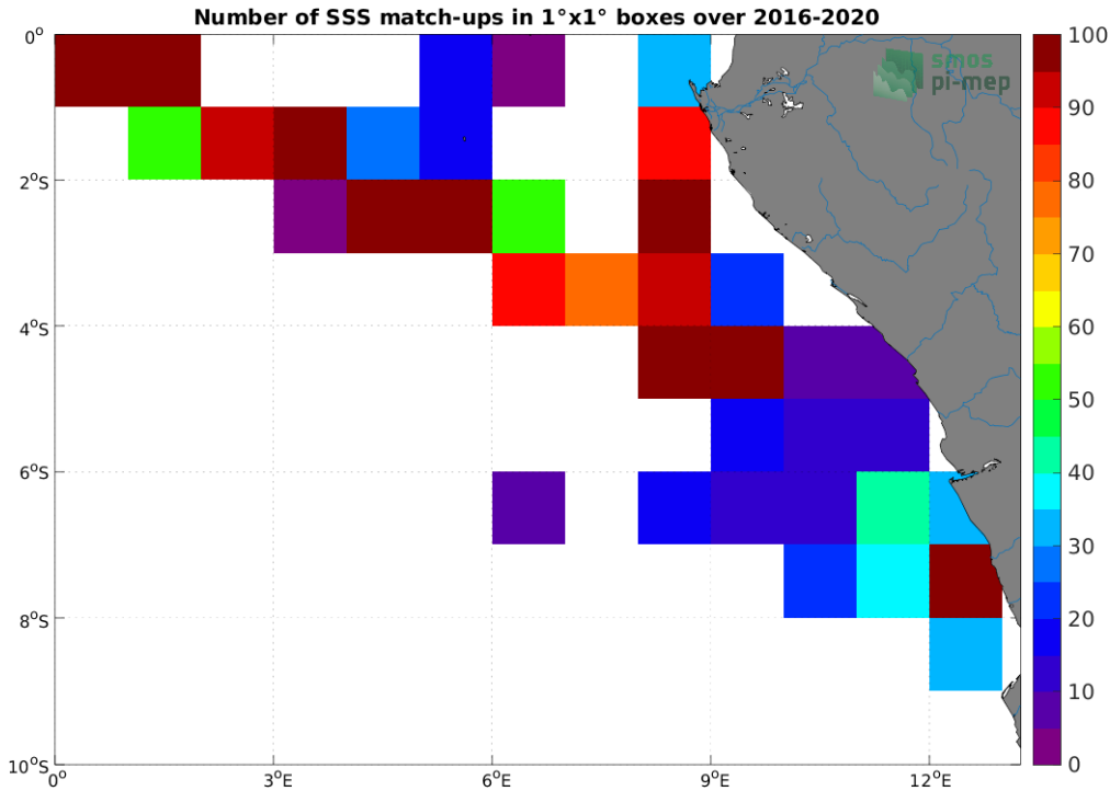
Figure 4: Number of SSS match-ups between TSG (LEGOS-DM) SSS and the SMOS SSS L2Q v331 - 0.25 Deg (CATDS-CPDC) SSS product for the Congo river plume Pi-MEP region over 1^\circ \times 1^\circ boxes and for the full satellite product period.
