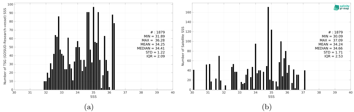
Figure 2: Histograms of SSS from TSG (GOSUD-Research-vessel) (a) and SMOS SSS L2Q v331 - 0.25 Deg (CATDS-CPDC) (b) considering all match-up pairs per bins of 0.1 over the Congo river plume Pi-MEP region and for the full satellite product period.
