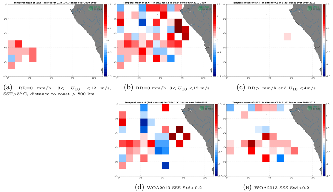
Figure 12: Temporal mean gridded over spatial boxes of size 1^\circ \times 1^\circ of \Delta SSS (SMOS SSS L2Q v331 - 0.25 Deg (CATDS-CPDC) - TSG (GOSUD-Research-vessel)) for 5 different subdatasets corresponding to:RR=0 mm/h, 3 < U_{10} < 12 m/s, SST >5^\circ\text{C} , distance to coast > 800 km (a), RR=0 mm/h, 3 < U_{10} < 12 m/s (b), RR >1 mm/h and U_{10} < 4 m/s (c), WOA2013 SSS Std <0.2 (d), WOA2013 SSS Std >0.2 (e).
