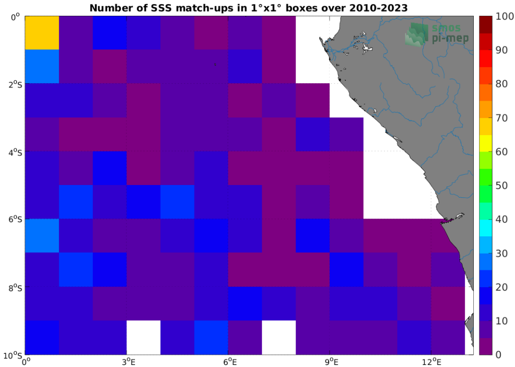
Figure 4: Number of SSS match-ups between Argo SSS and the SMOS SSS L2Q v331 - 0.25 Deg (CATDS-CPDC) SSS product for the Congo river plume Pi-MEP region over 1^\circ \times 1^\circ boxes and for the full satellite product period.
