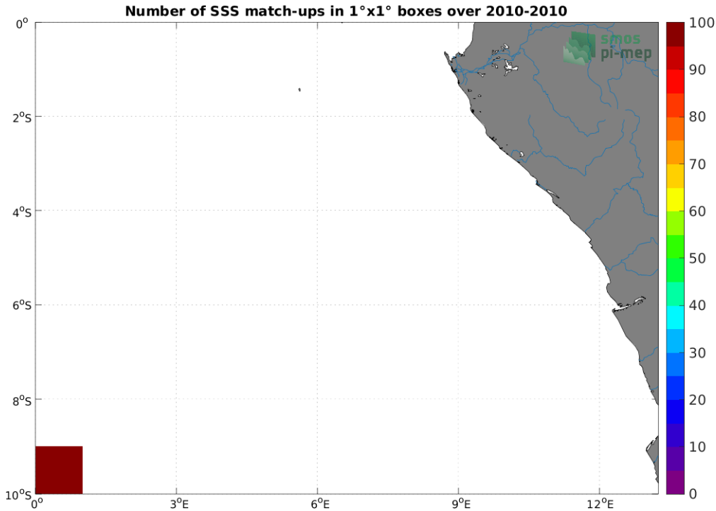
Figure 4: Number of SSS match-ups between TSG (SAMOS) SSS and the SMOS SSS L2Q v330 - 0.25 Deg (CATDS-CPDC) SSS product for the Congo river plume Pi-MEP region over 1°x1° boxes and for the full satellite product period.
