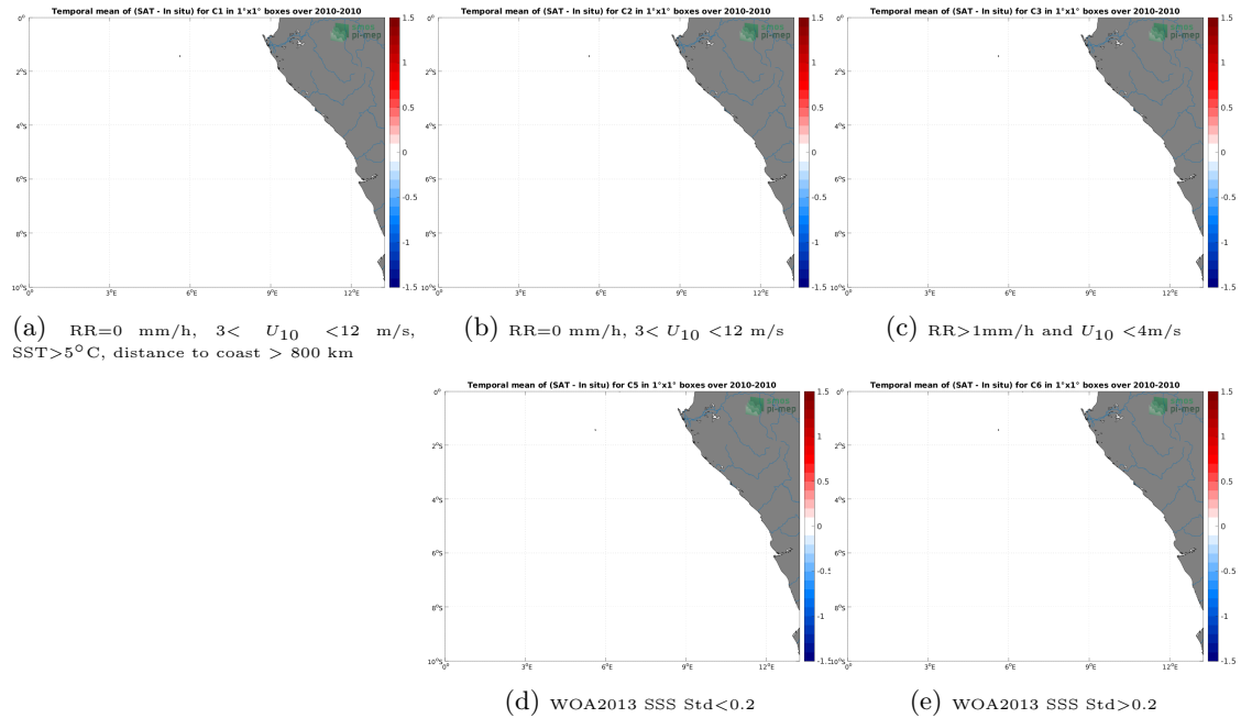
Figure 12: Temporal mean gridded over spatial boxes of size 1^\circ \times 1^\circ of \Delta\text{SSS} (SMOS SSS L2Q v330 - 0.25 Deg (CATDS-CPDC) - TSG (SAMOS)) for 5 different subdatasets corresponding to:RR=0 mm/h, 3 < U_{10} < 12 m/s, SST > 5^\circ\text{C} , distance to coast > 800 km (a), RR=0 mm/h, 3 < U_{10} < 12 m/s (b), RR > 1 mm/h and U_{10} < 4 m/s (c), WOA2013 SSS Std < 0.2 (d), WOA2013 SSS Std > 0.2 (e).
